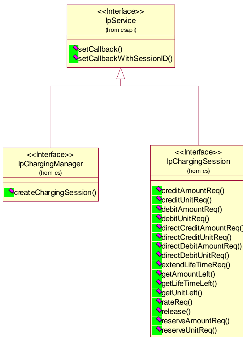
Figure 2: Service Interfaces
