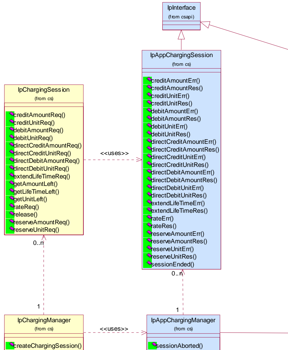
Figure 1: Application Interfaces
