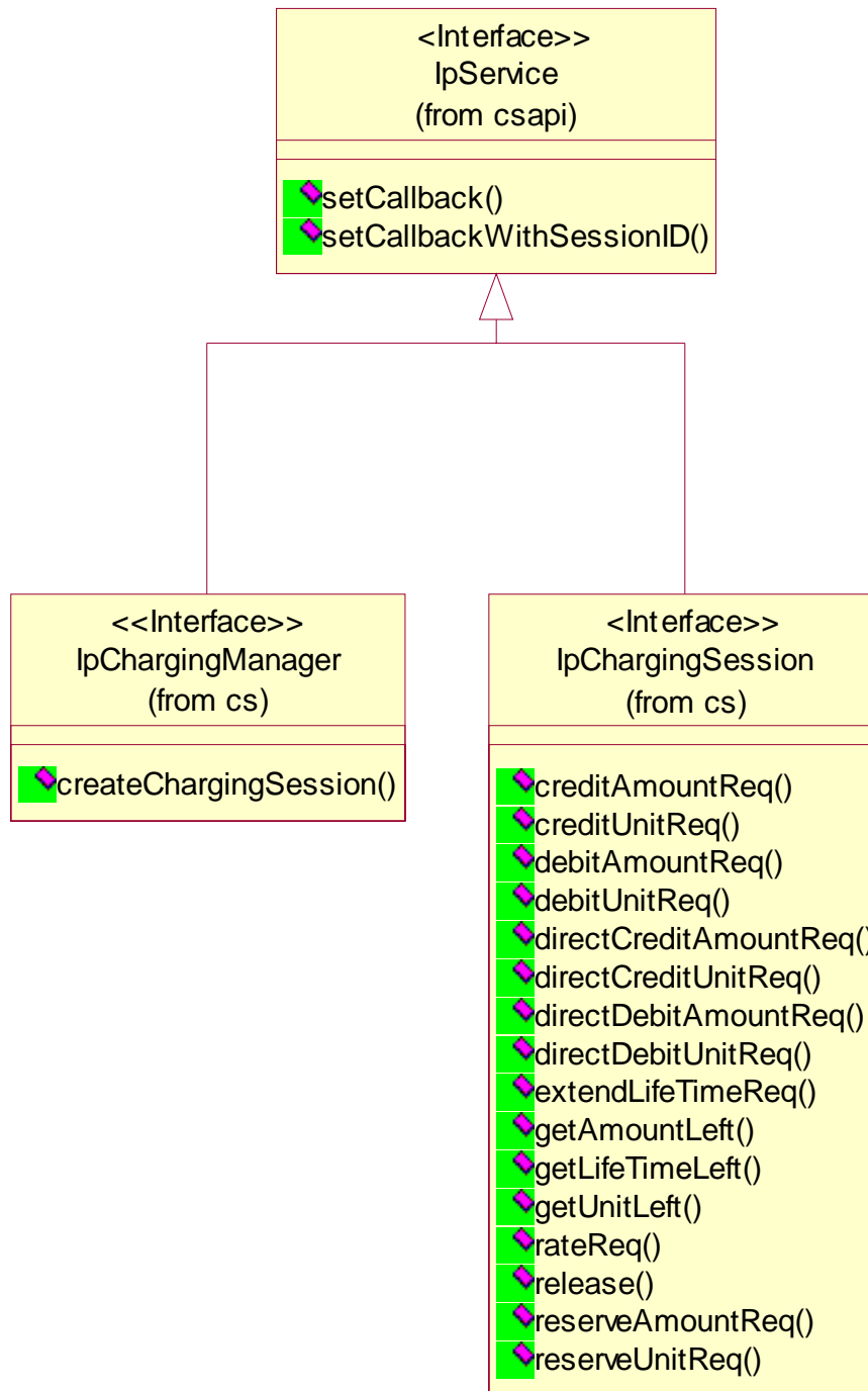
Figure 2: Service Interfaces
