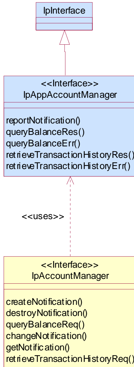
Figure 1: Application Interfaces
