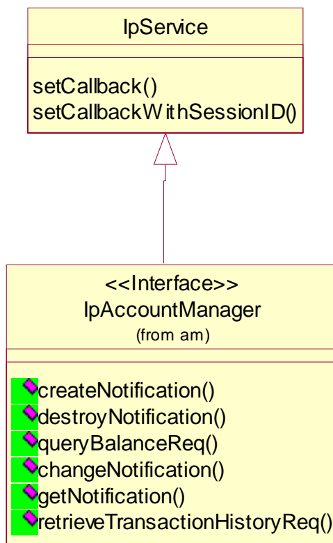
Figure 2: Service Interfaces
