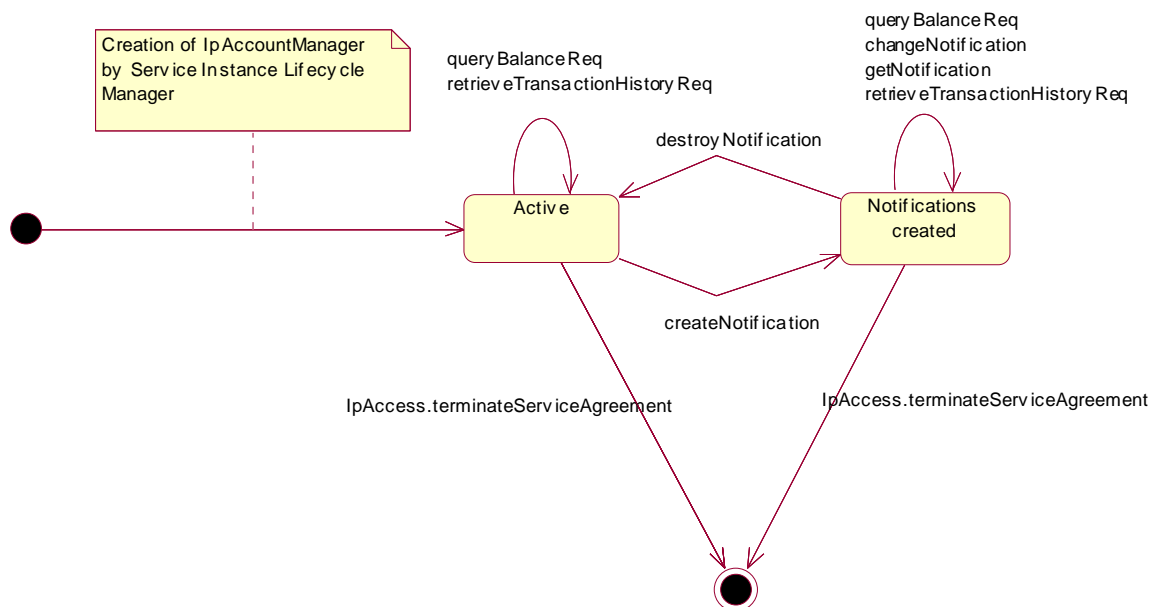
Figure 3: Application view on the IpAccountManager
