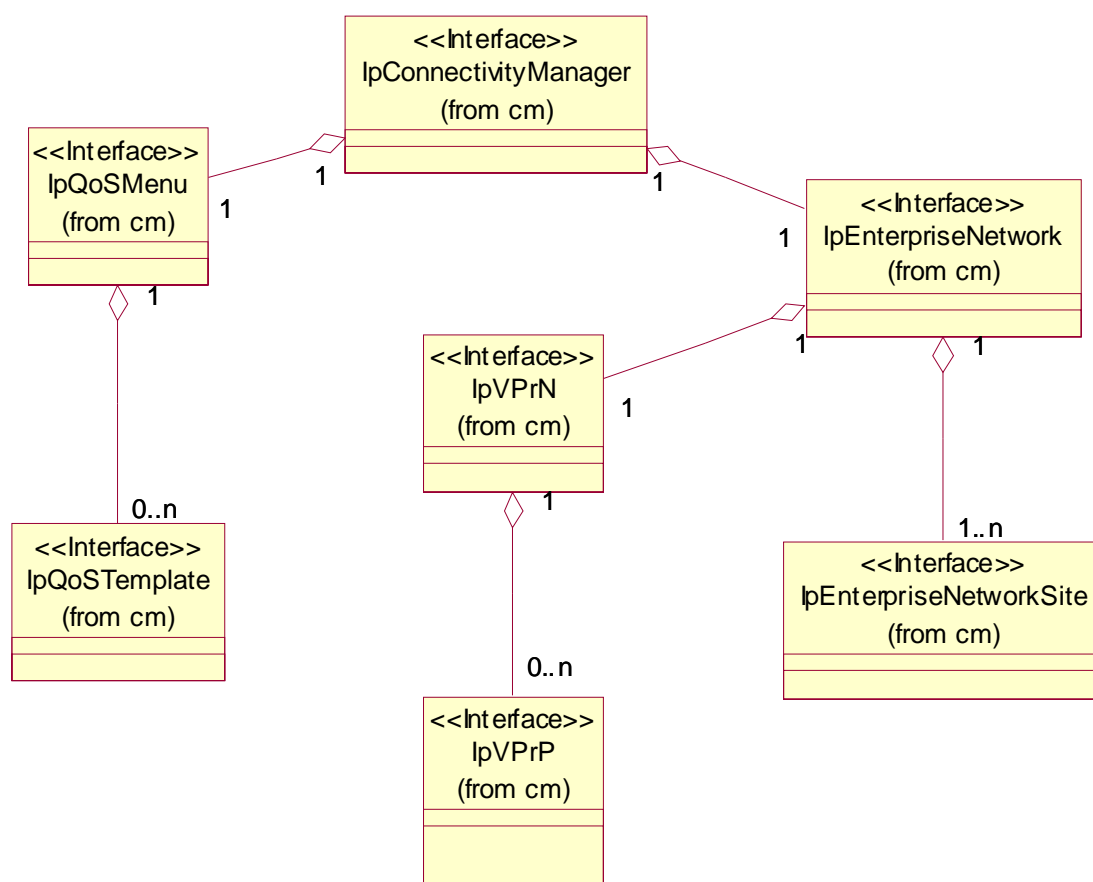
Figure 1: Connectivity Management High level class diagram
