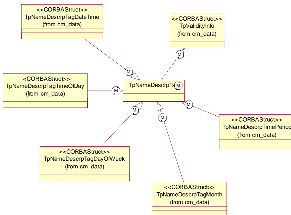
Figure 7: Validity Data Type Classes
