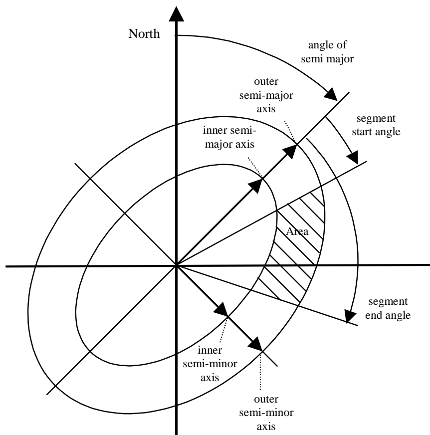
Figure 7: Description of an Ellipse Arc
