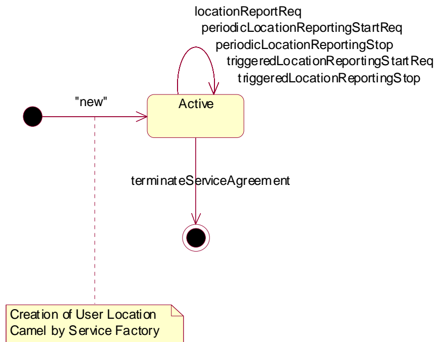
Figure 5: State Transition Diagram for User Location Camel
