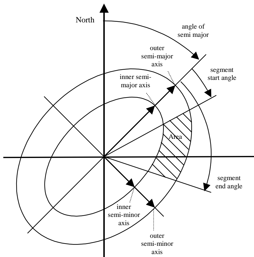
Figure 7: Description of an Ellipse Arc
