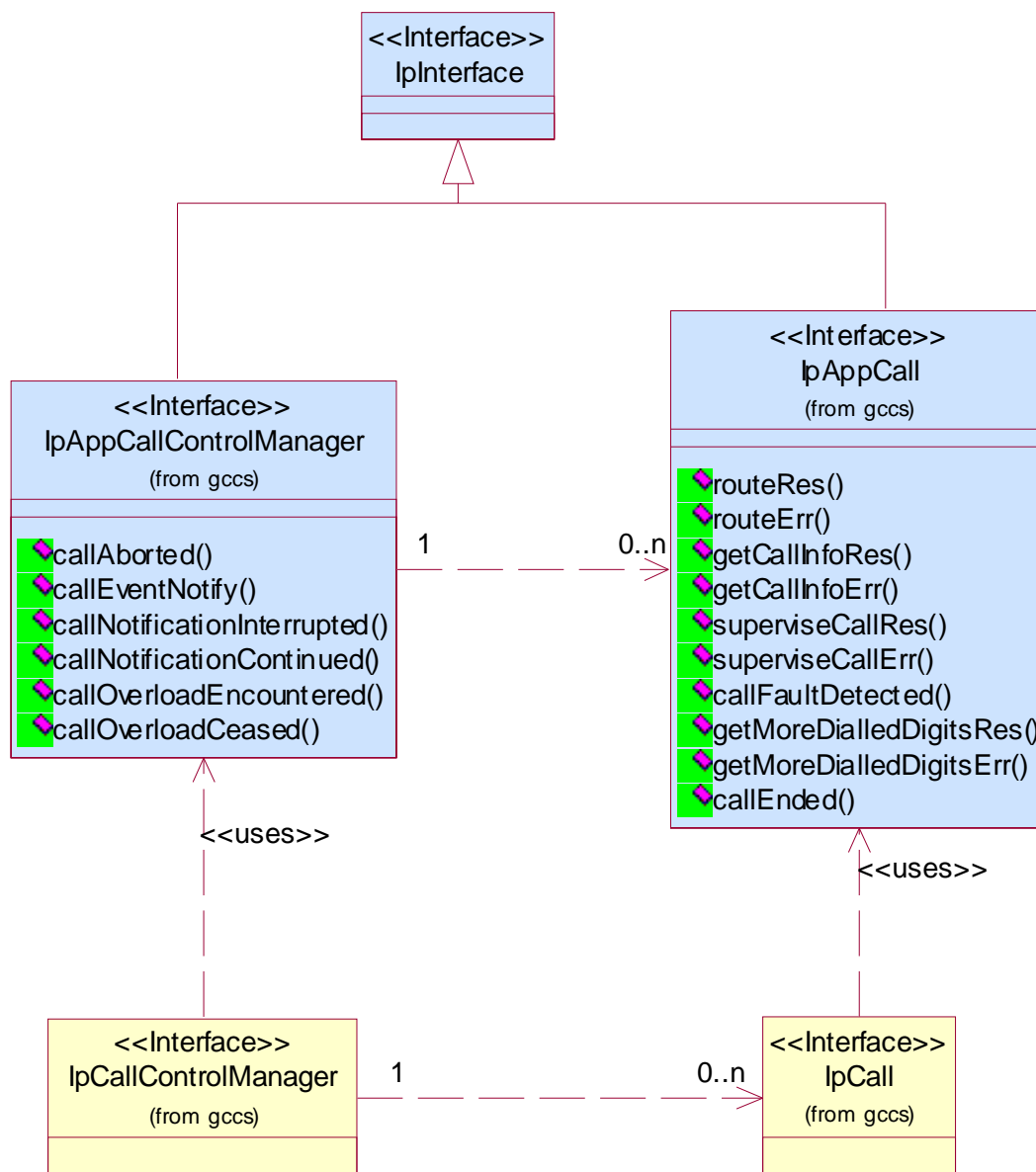
Figure 2: Application Interfaces
