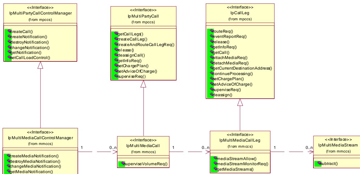
Figure 16: Service Interfaces
