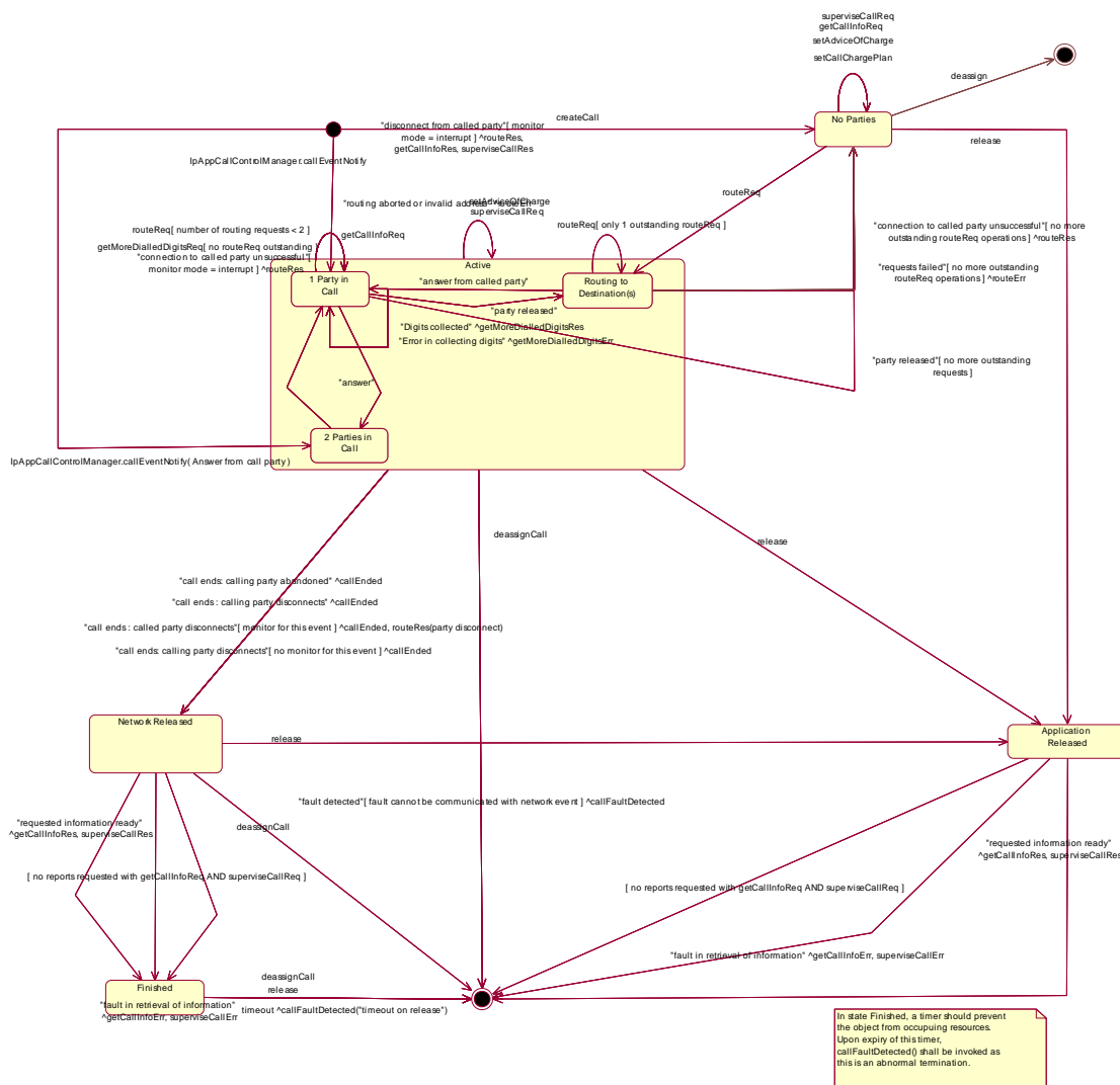
Figure 4: Application view on the IpCall object
