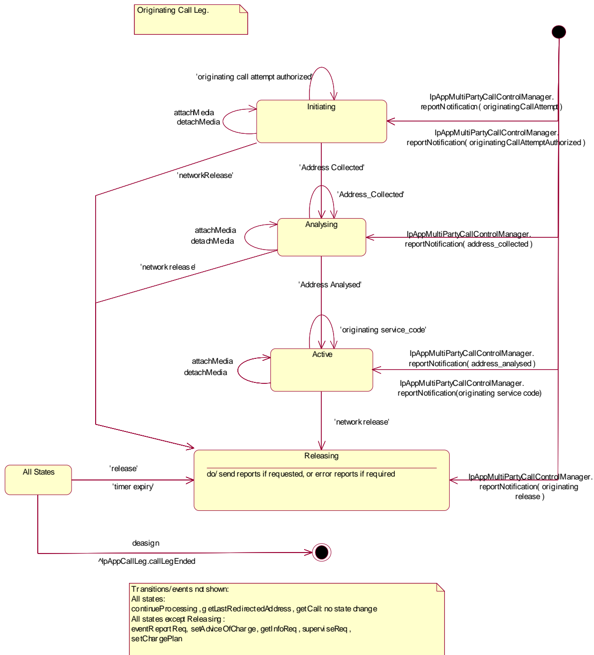
Figure 9: Originating Leg
