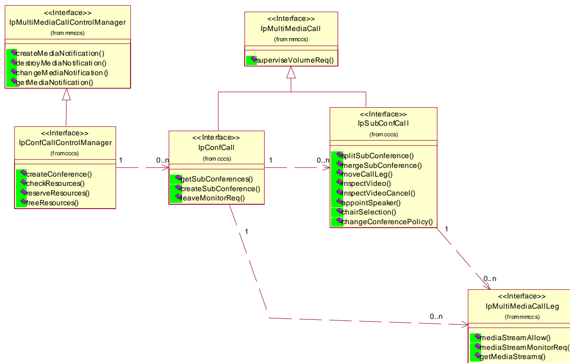
Figure 18: Service Interfaces
