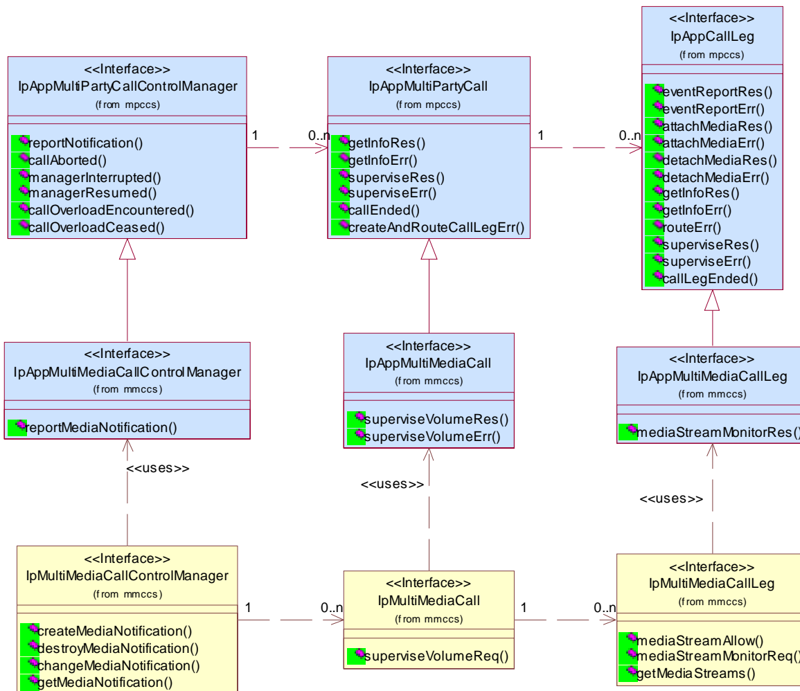
Figure 15: Application Interfaces
