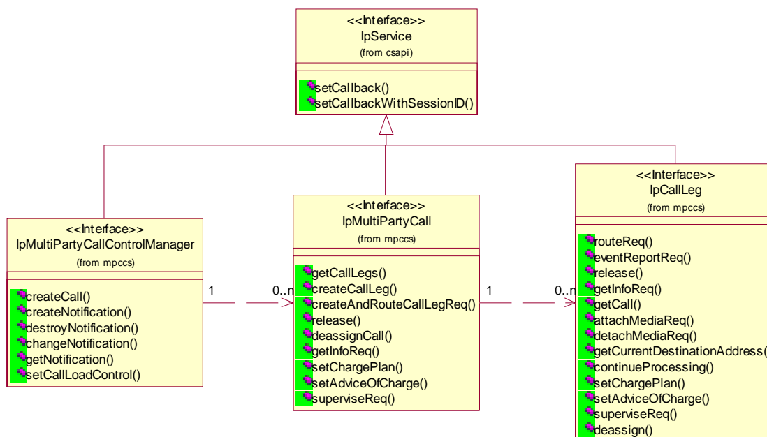
Figure 6: Service Interfaces
