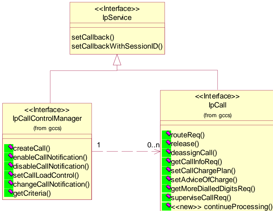
Figure 1: Service Interfaces
