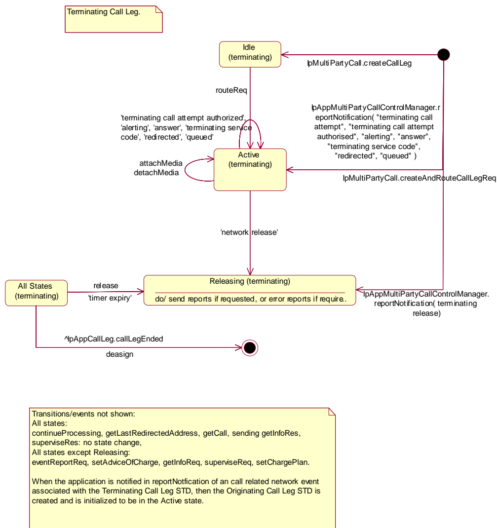
Figure 13: Terminating Leg
