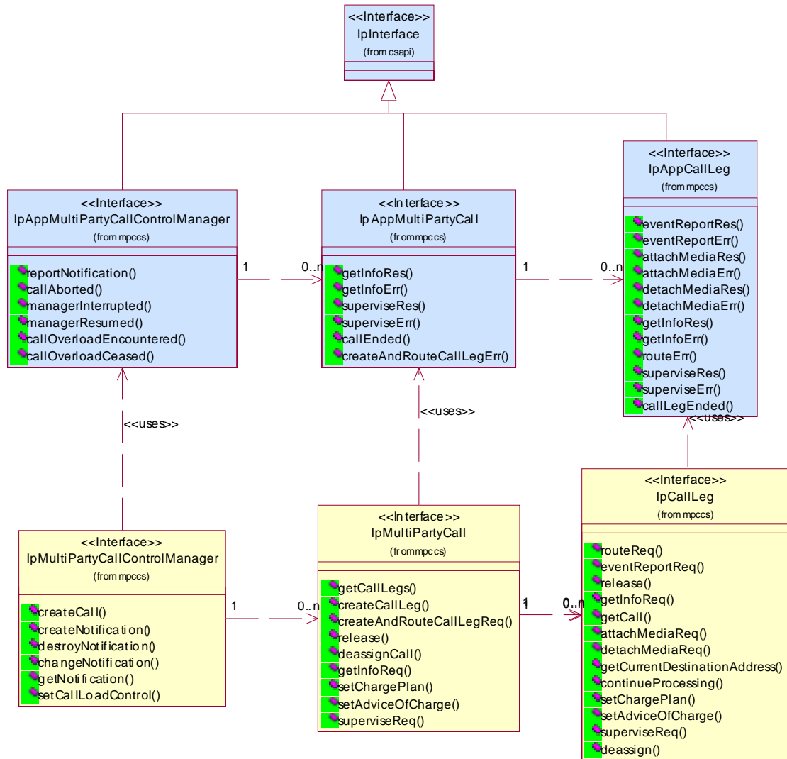
Figure 5: Application Interfaces
