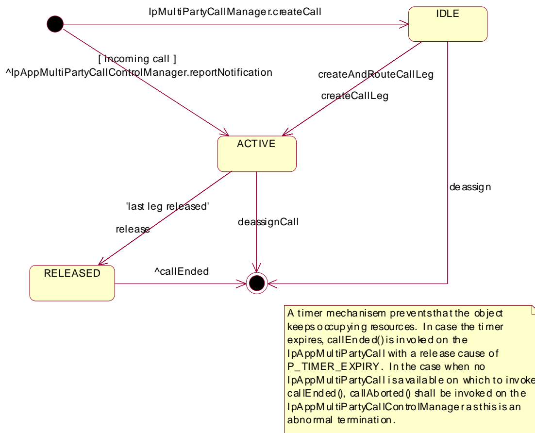
Figure 8: Application view on the MultiParty Call object
