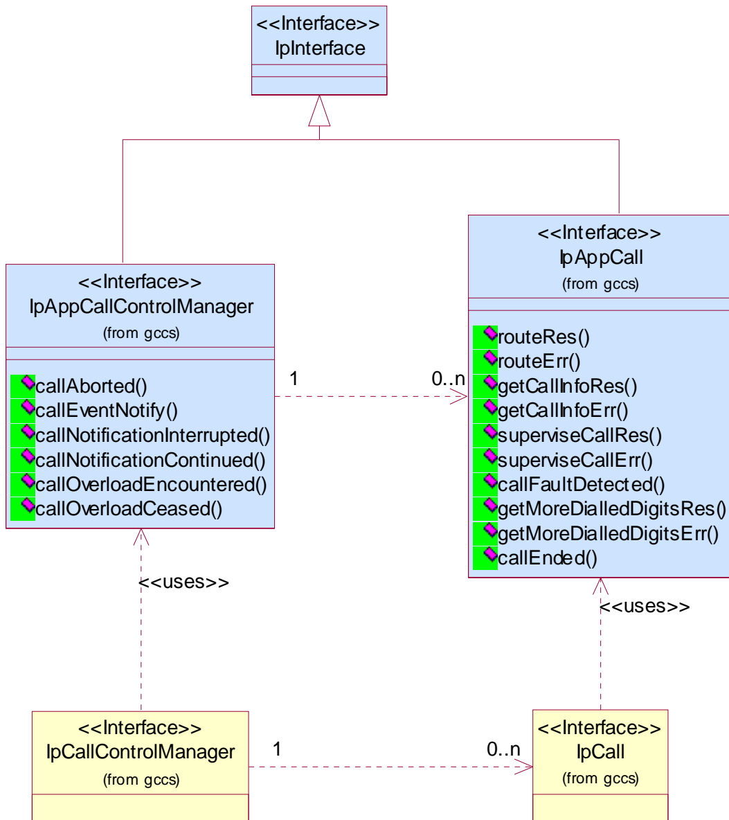
Figure 2: Application Interfaces
