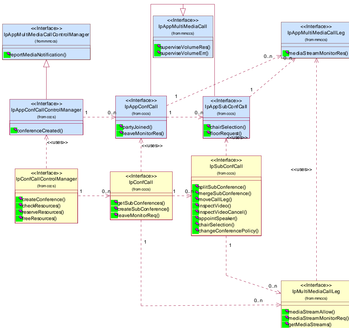
Figure 17: Application Interfaces
