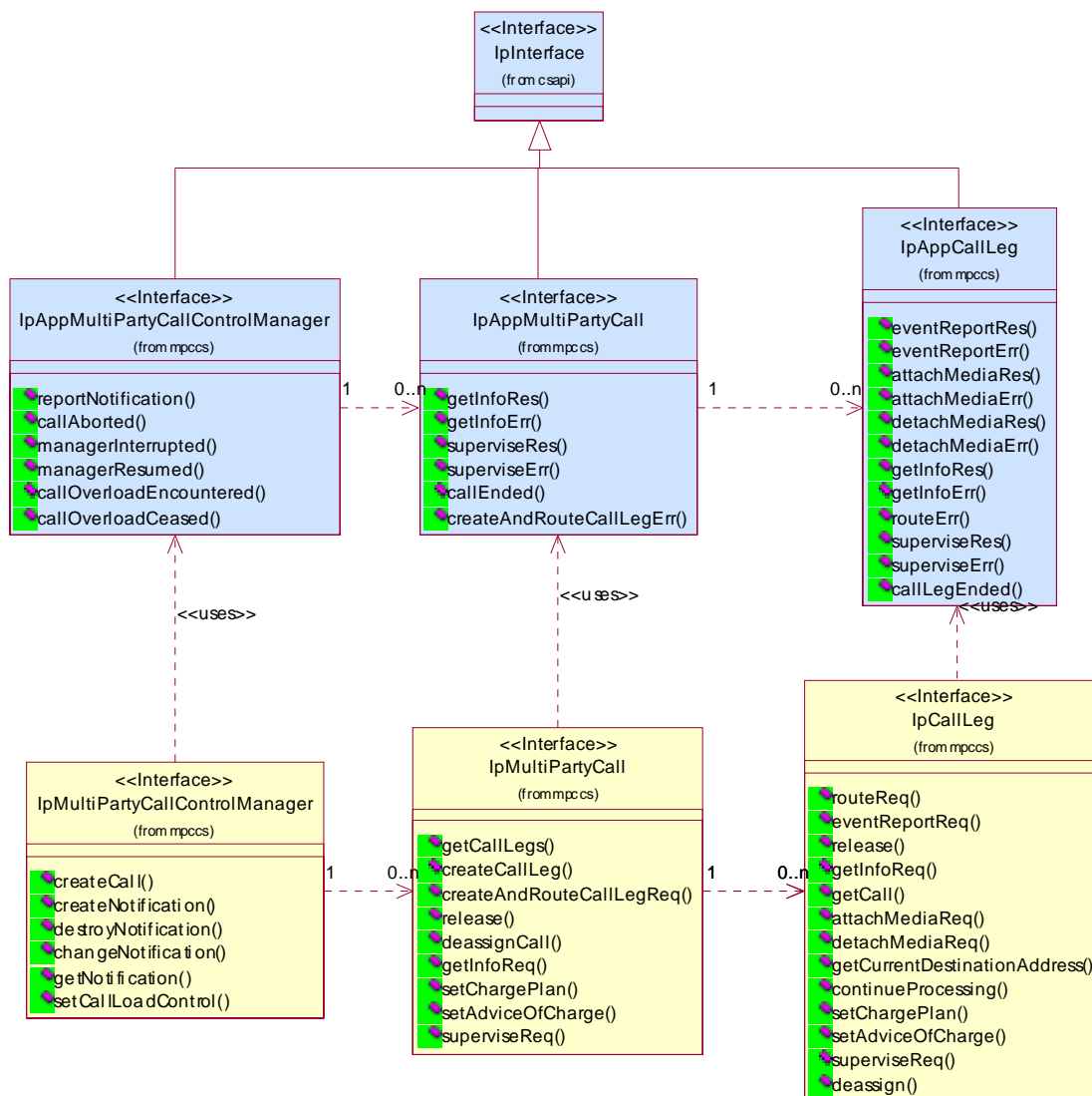
Figure 5: Application Interfaces
