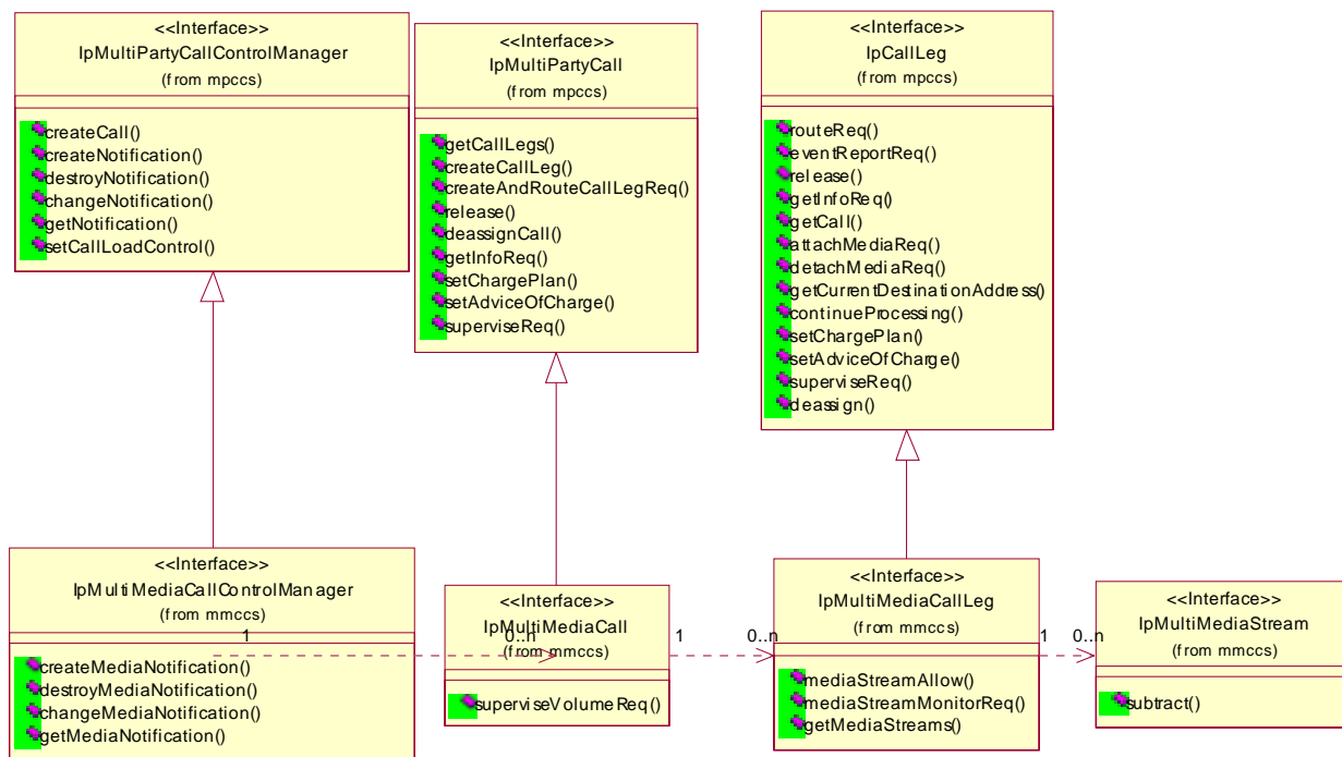
Figure 16: Service Interfaces
