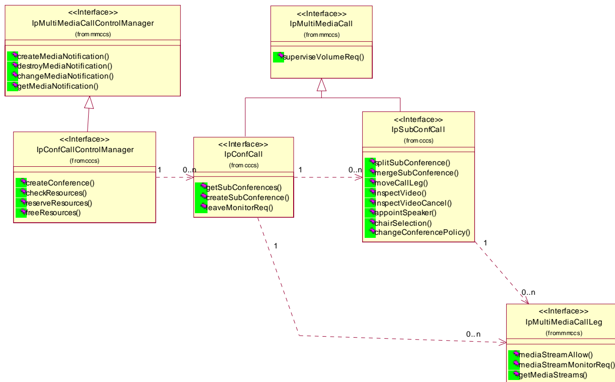
Figure 18: Service Interfaces
