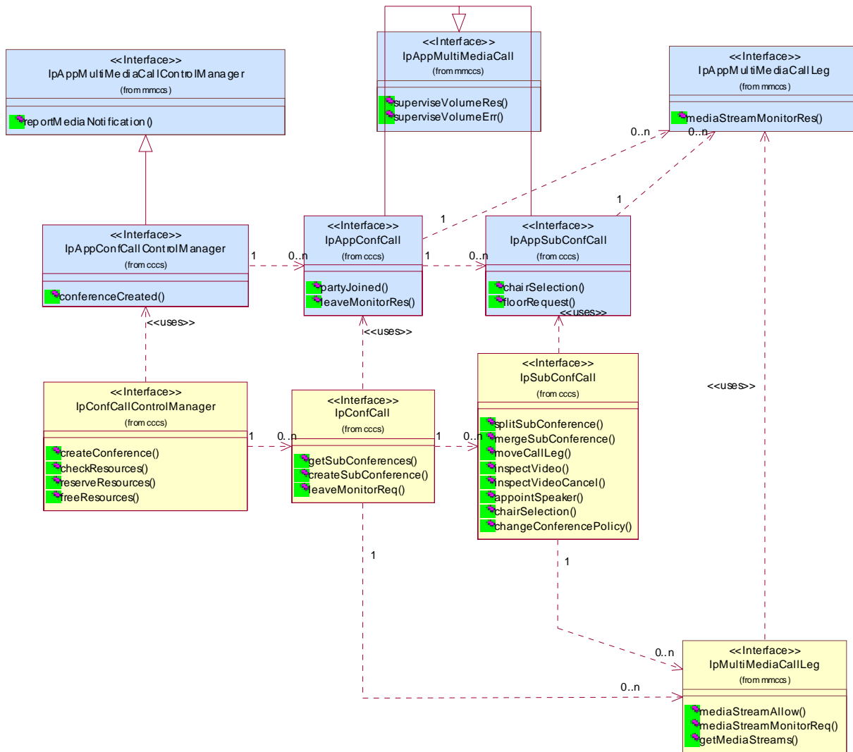
Figure 17: Application Interfaces
