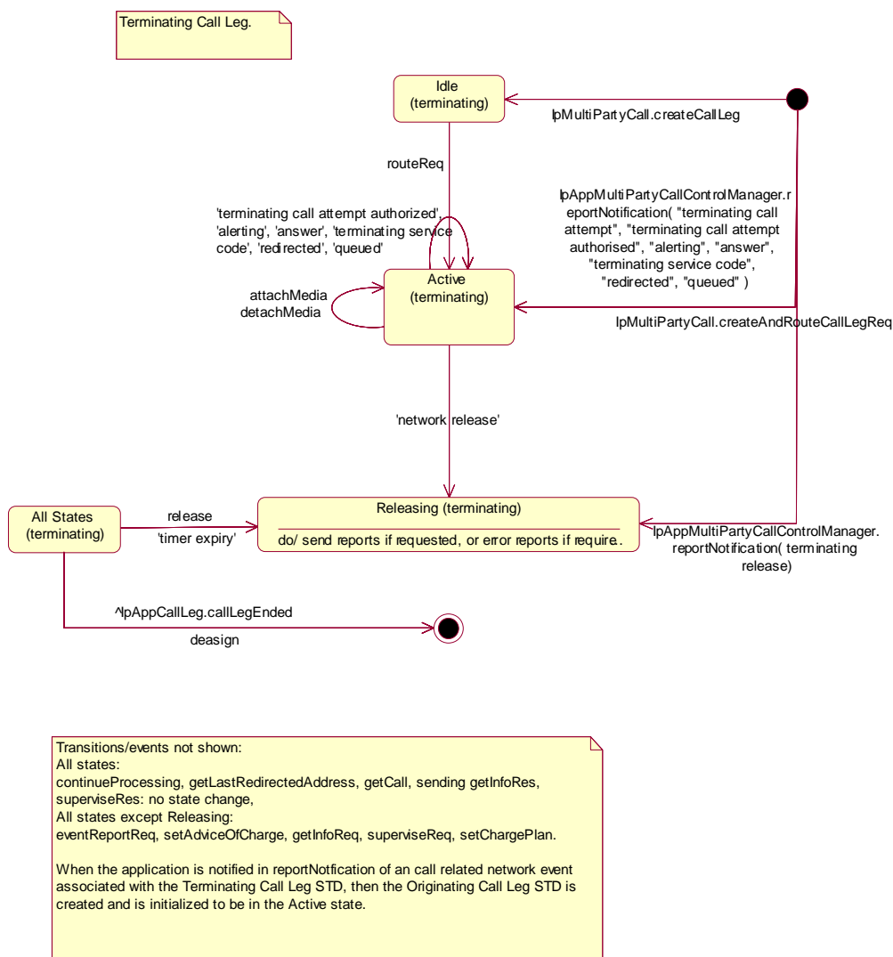
Figure 13: Terminating Leg
