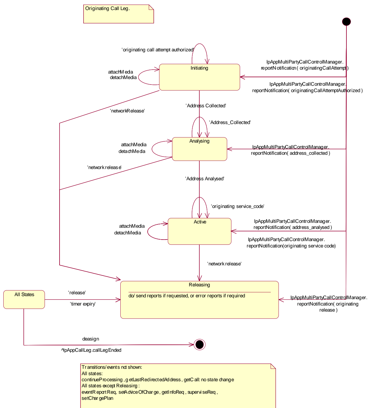
Figure 9: Originating Leg
