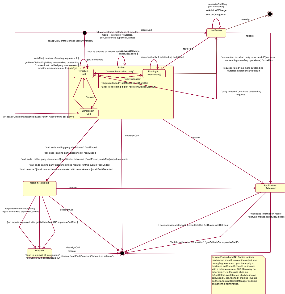
Figure 4: Application view on the IpCall object
