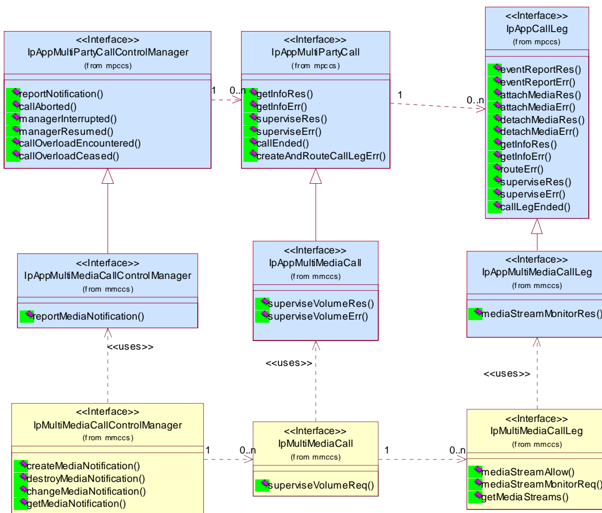
Figure 15: Application Interfaces
