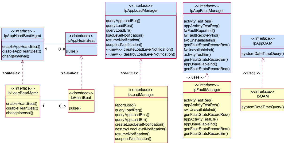
Figure 6: Integrity Management Package Overview
