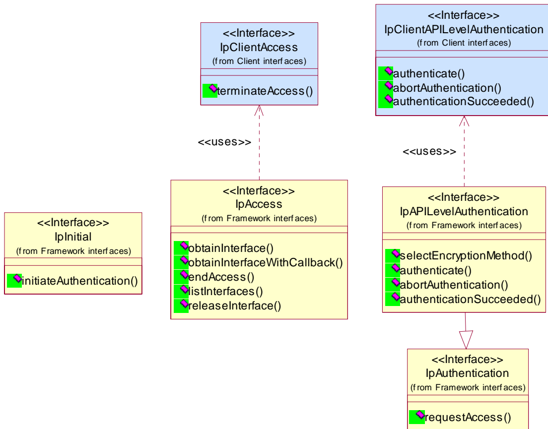
Figure 8: Trust and Security Management Package Overview
