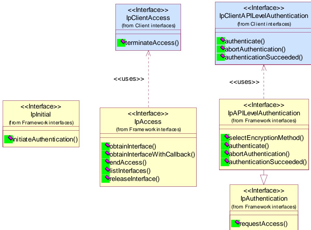
Figure 1: Trust and Security Management Package Overview
