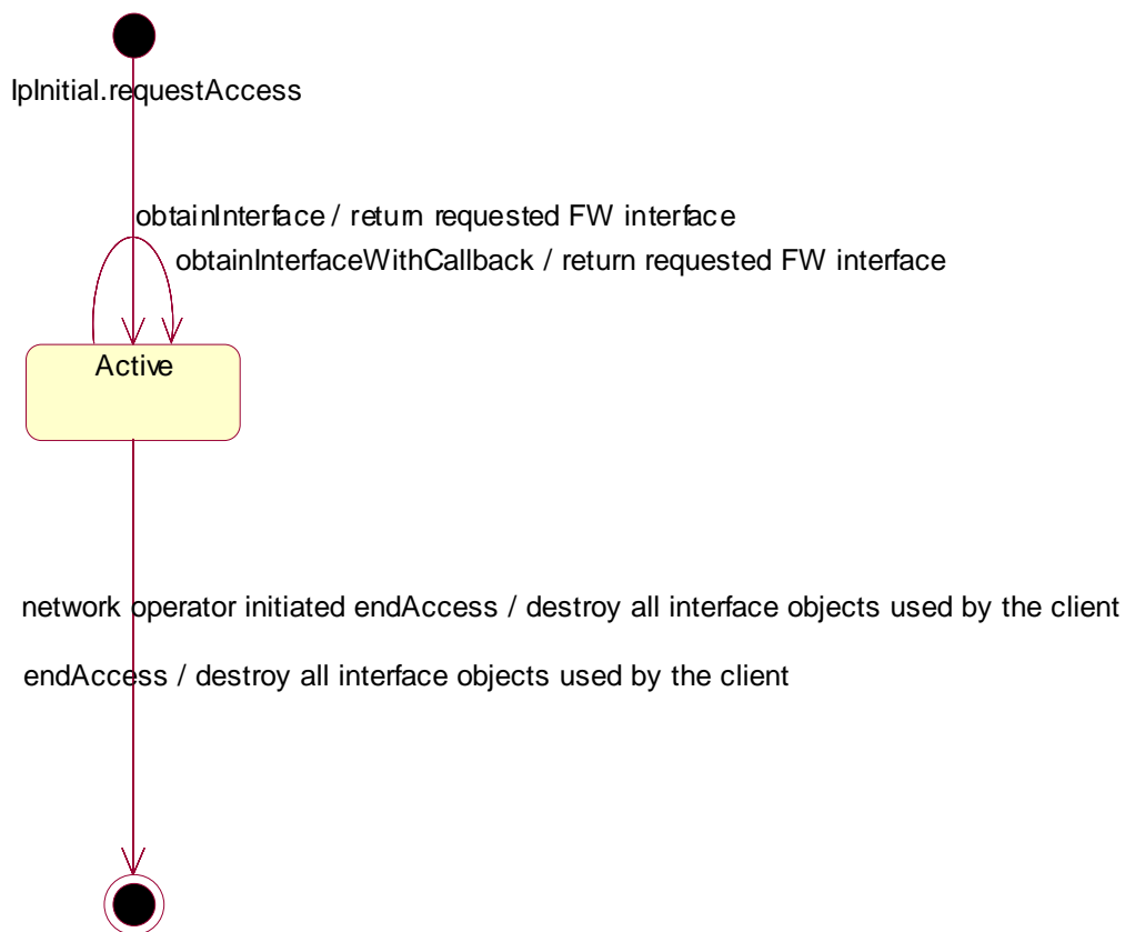
Figure 4: State Transition Diagram for IpAccess
