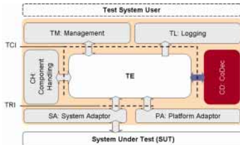
Figure 6: The TCI-CD interface
