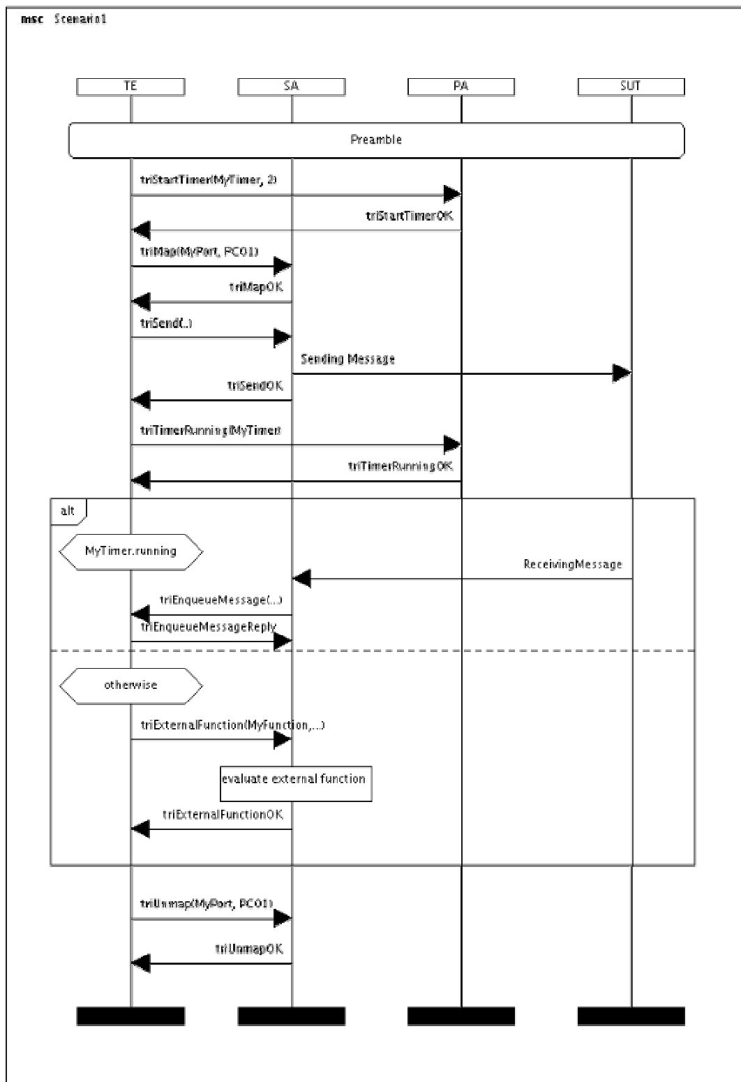
Figure 3: Use Scenario 1
