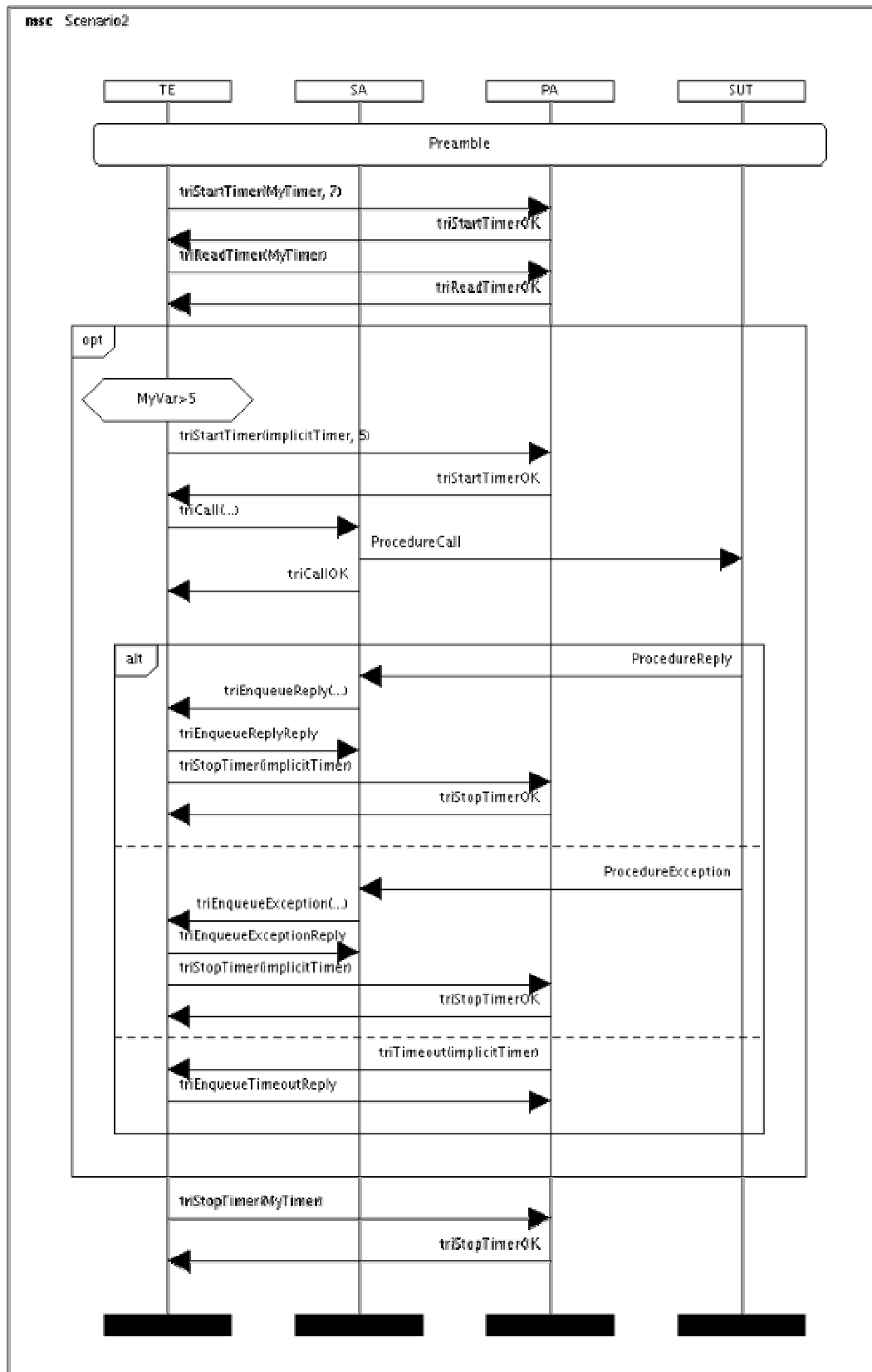
Figure 4: Use Scenario 2
