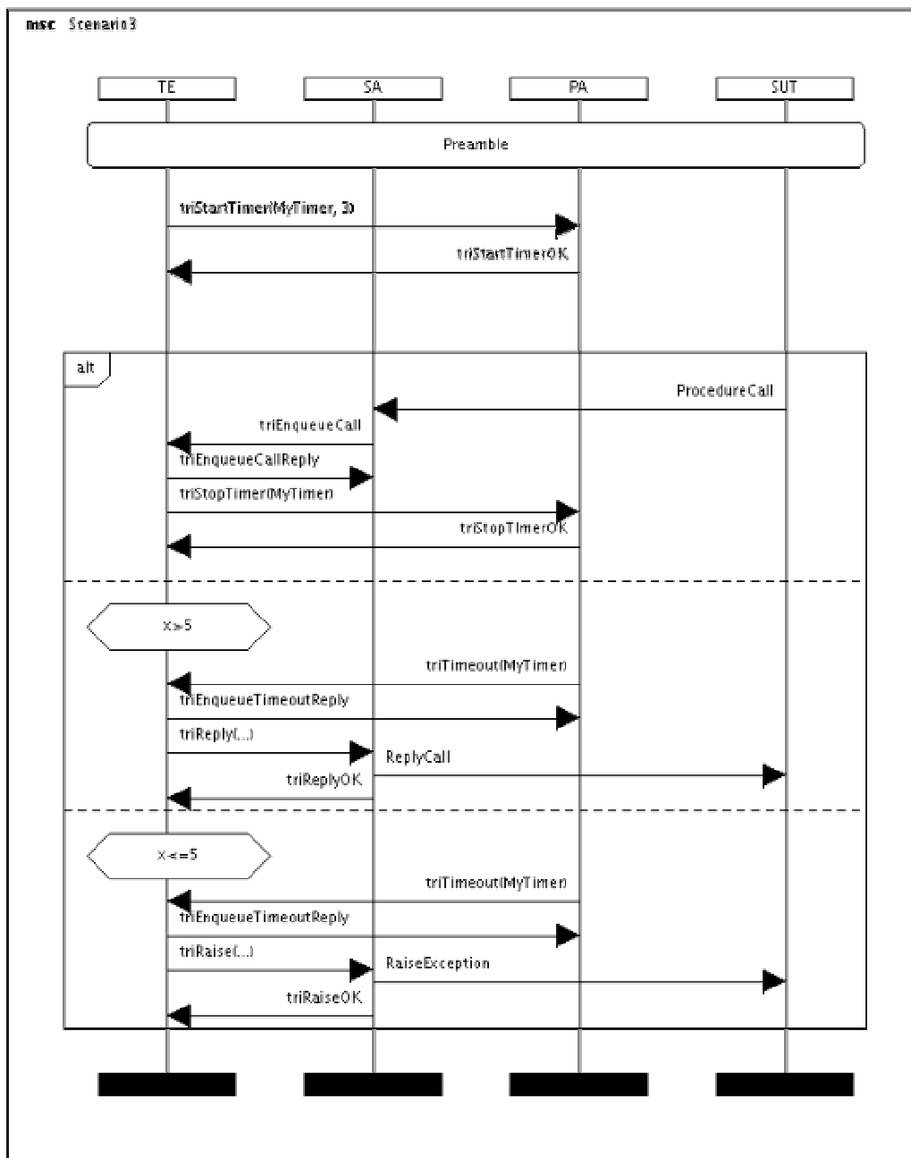
Figure 5: Use Scenario 3
