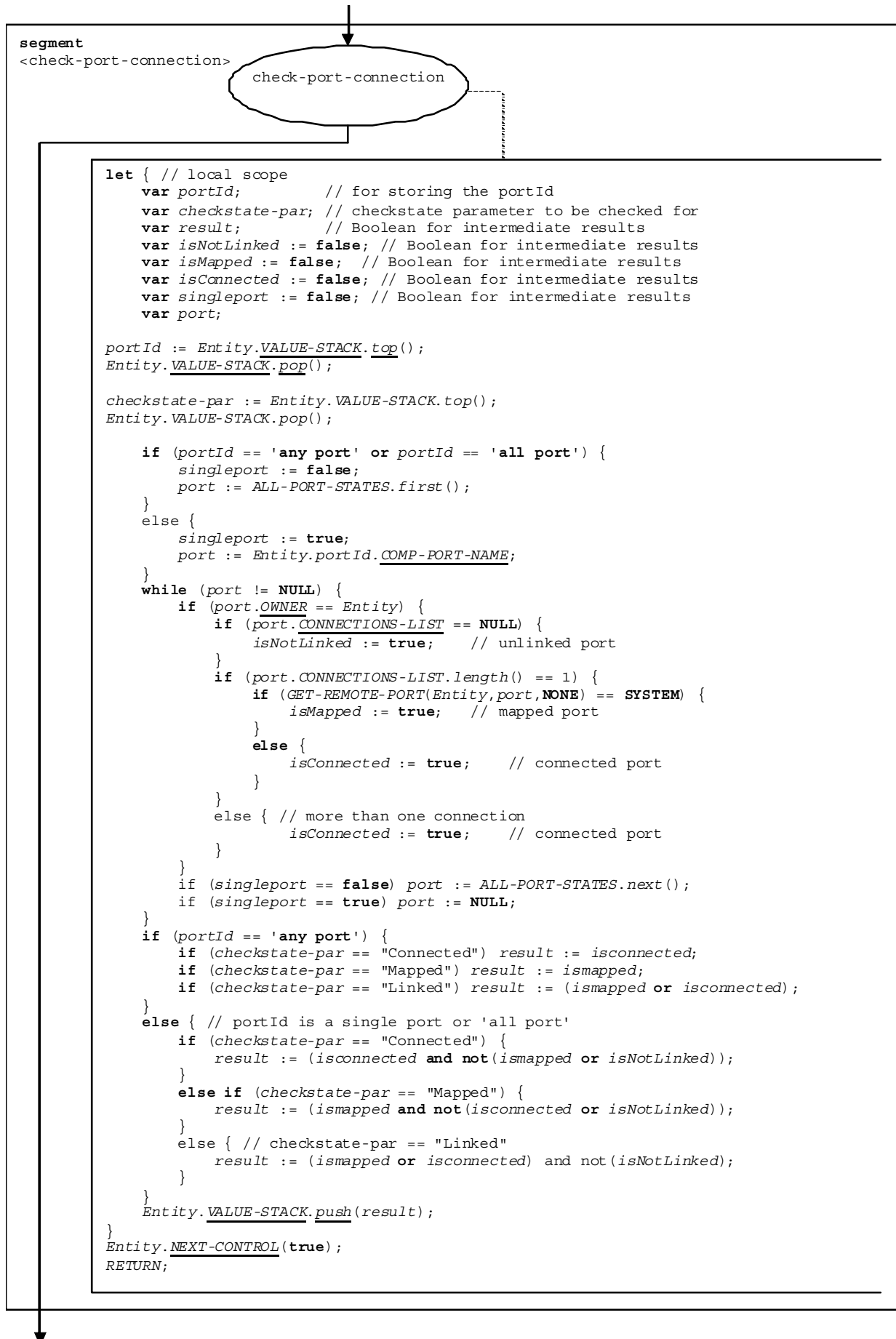
Figure 58c: Flow graph segment &lt;check-port-connection&gt;
