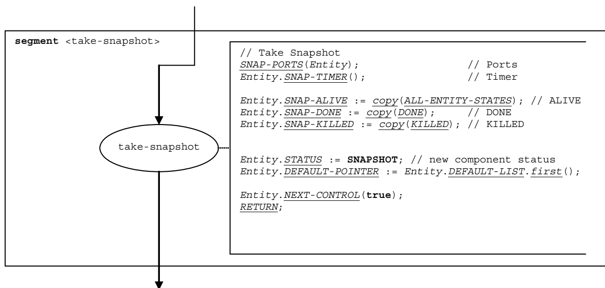
Figure 39: Flow graph segment <take-snapshot>
