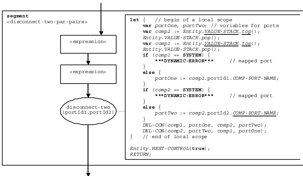
Figure 64e: Flow graph segment <disconnect-two-par-pairs>
