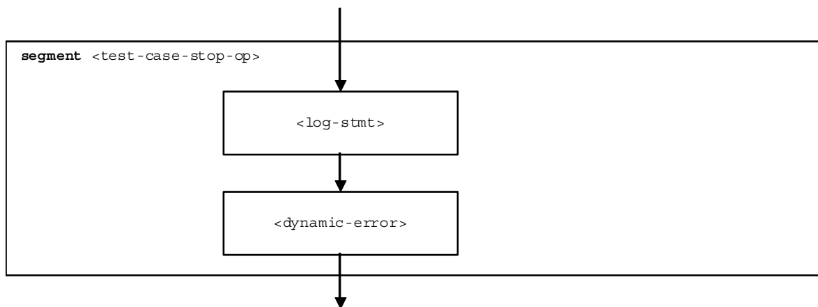
Figure 131a: Flow graph segment <test-case-stop-op>
