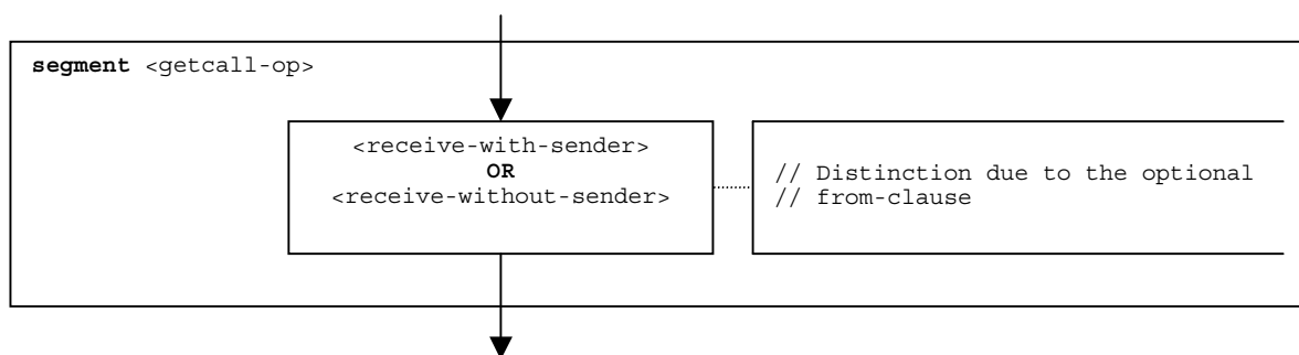
Figure 86: Flow graph segment <getcall-op>
