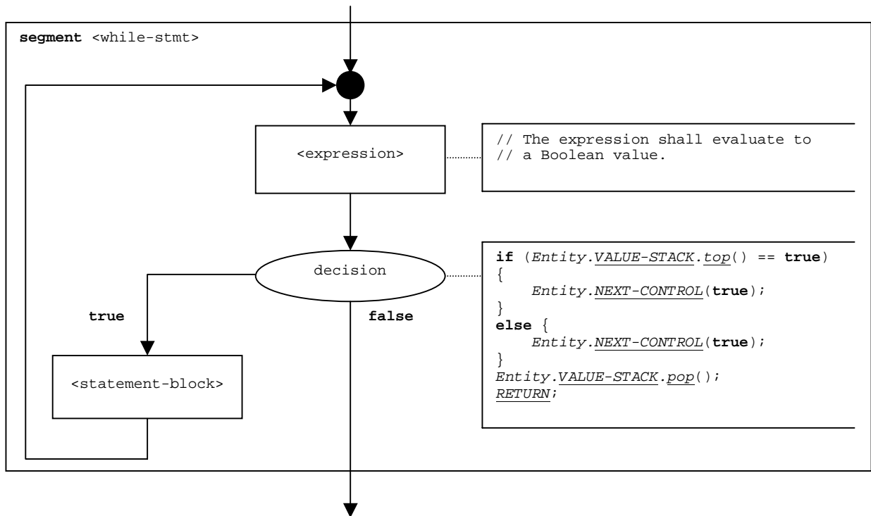
Figure 142: Flow graph segment <while-stmt>
