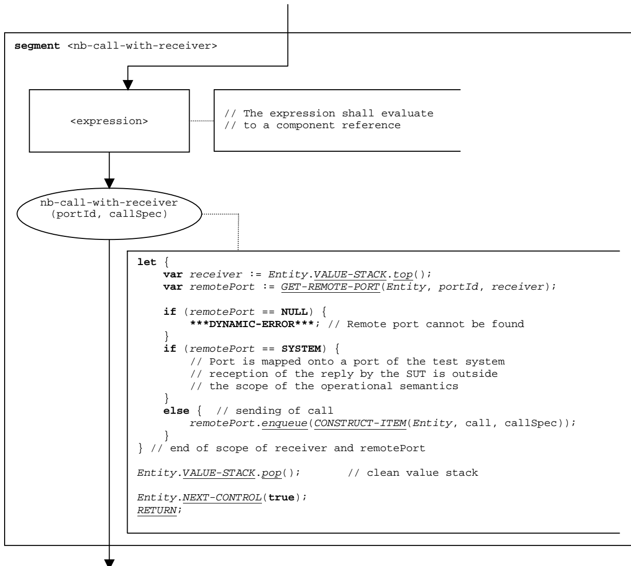
Figure 49: Flow graph segment <nb-call-with-receiver>
