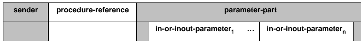
Figure 32: Structure of a procedure call
