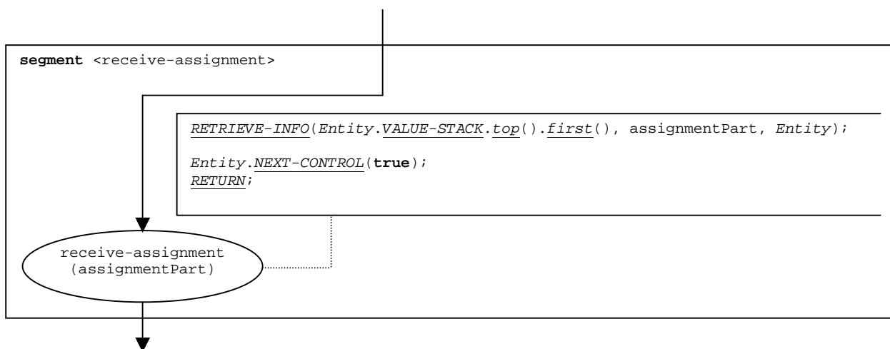
Figure 103: Flow graph segment <receive-assignment>
