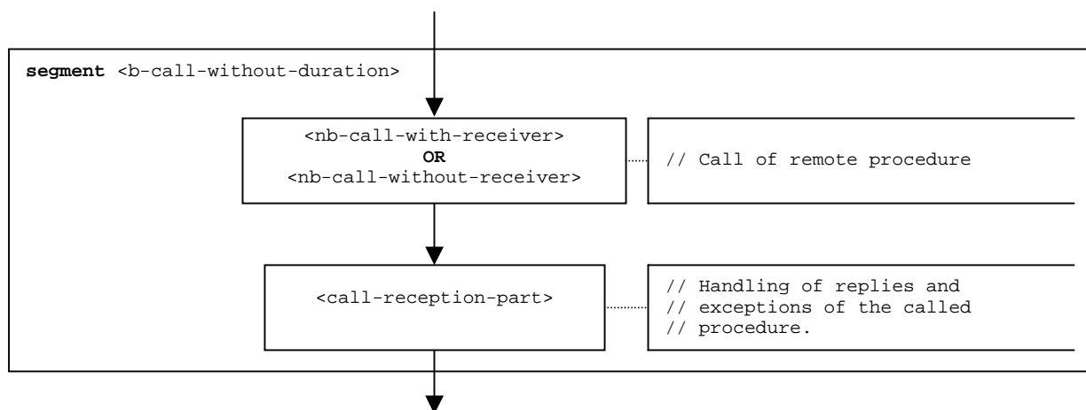
Figure 51: Flow graph segment <b-call-without-duration>
