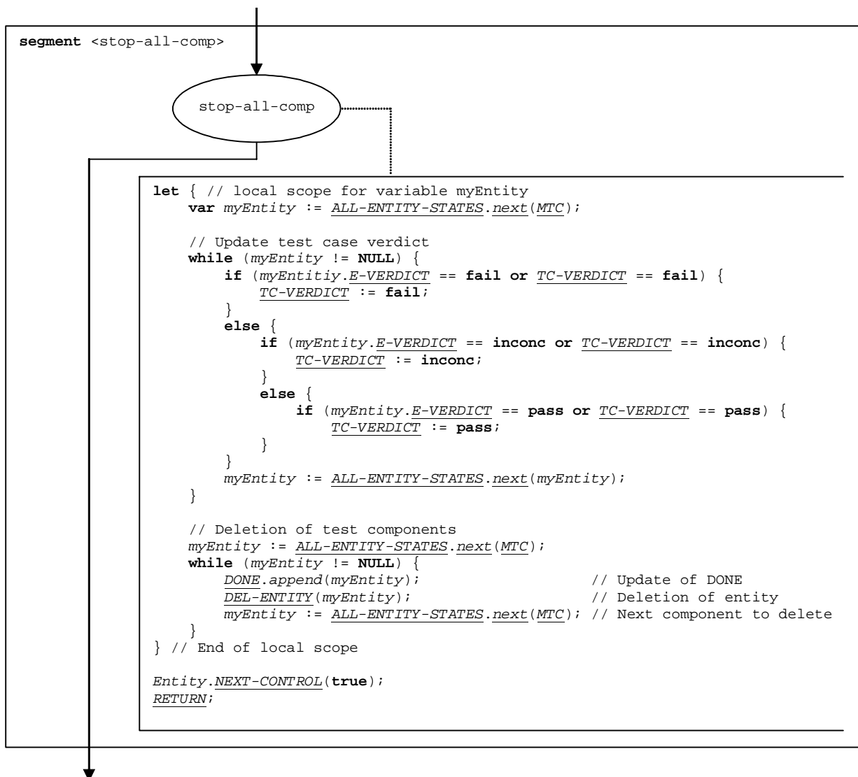
Figure 128: Flow graph segment <stop-all-comp>
