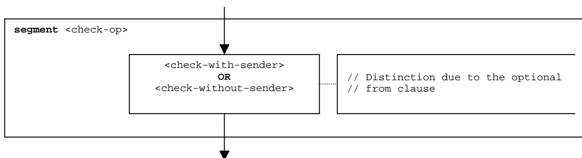
Figure 56: Flow graph segment <check-op>
