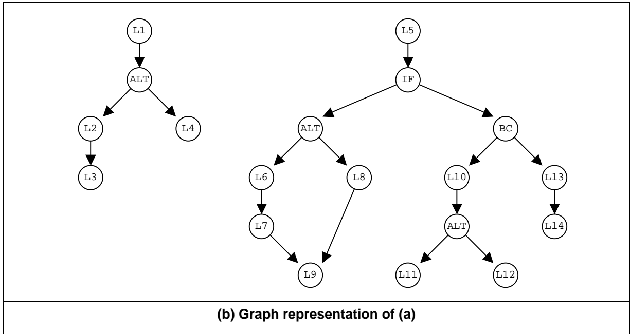
Figure 6: Graph representation of a TTCN-3 interleave statement
