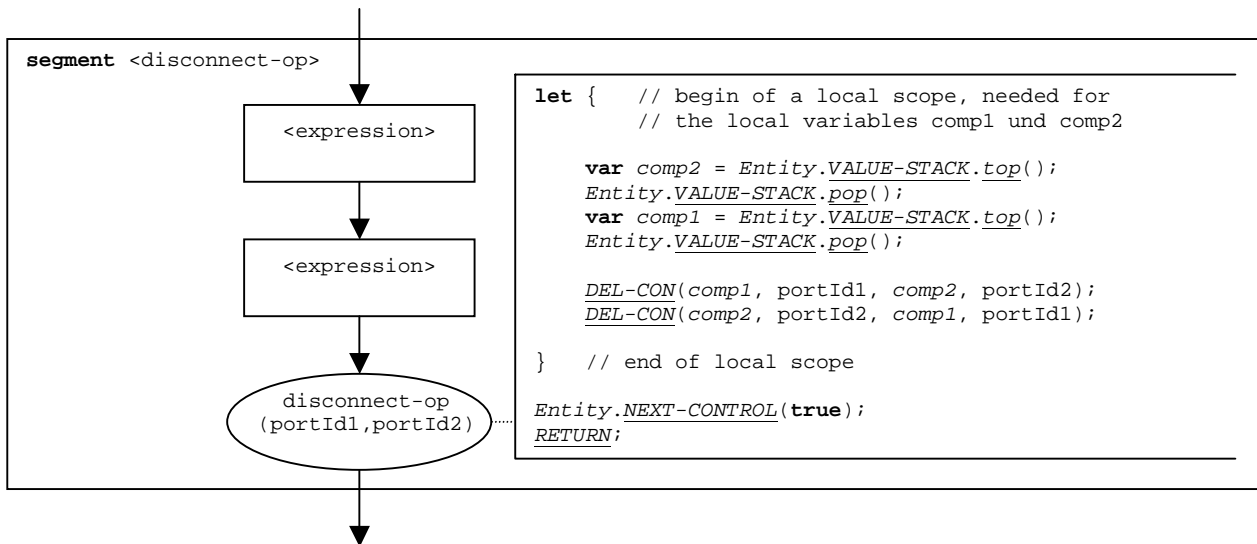
Figure 64: Flow graph segment &lt;disconnect-op&gt;
