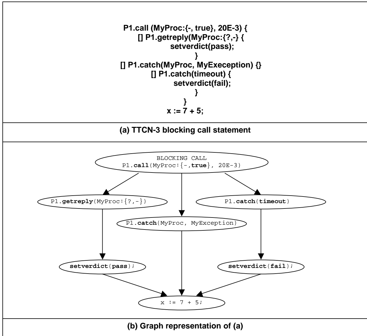
Figure 3: Graph representation of a TTCN-3 blocking call statement
