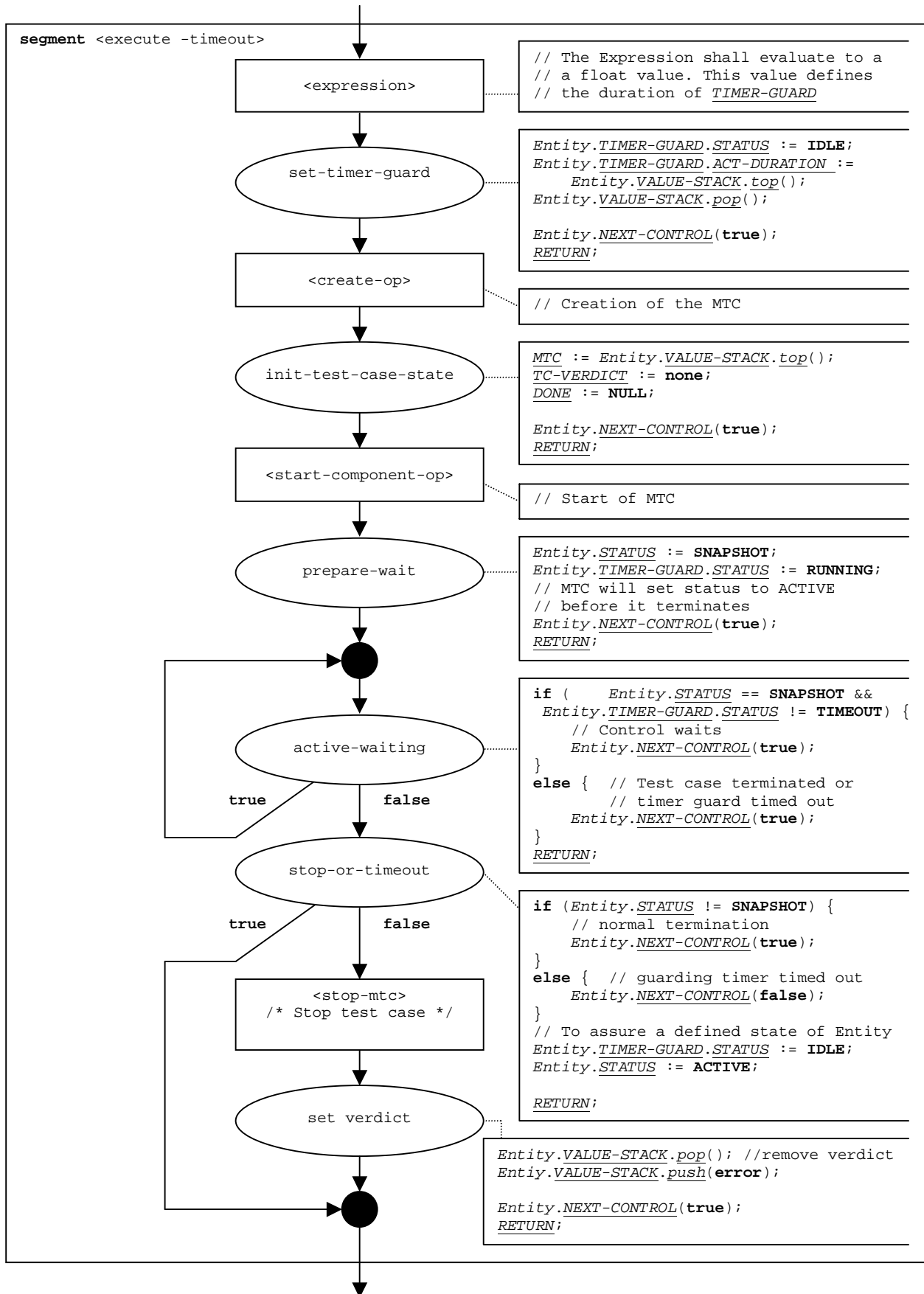
Figure 69: Flow graph segment &lt;execute-timeout&gt;
