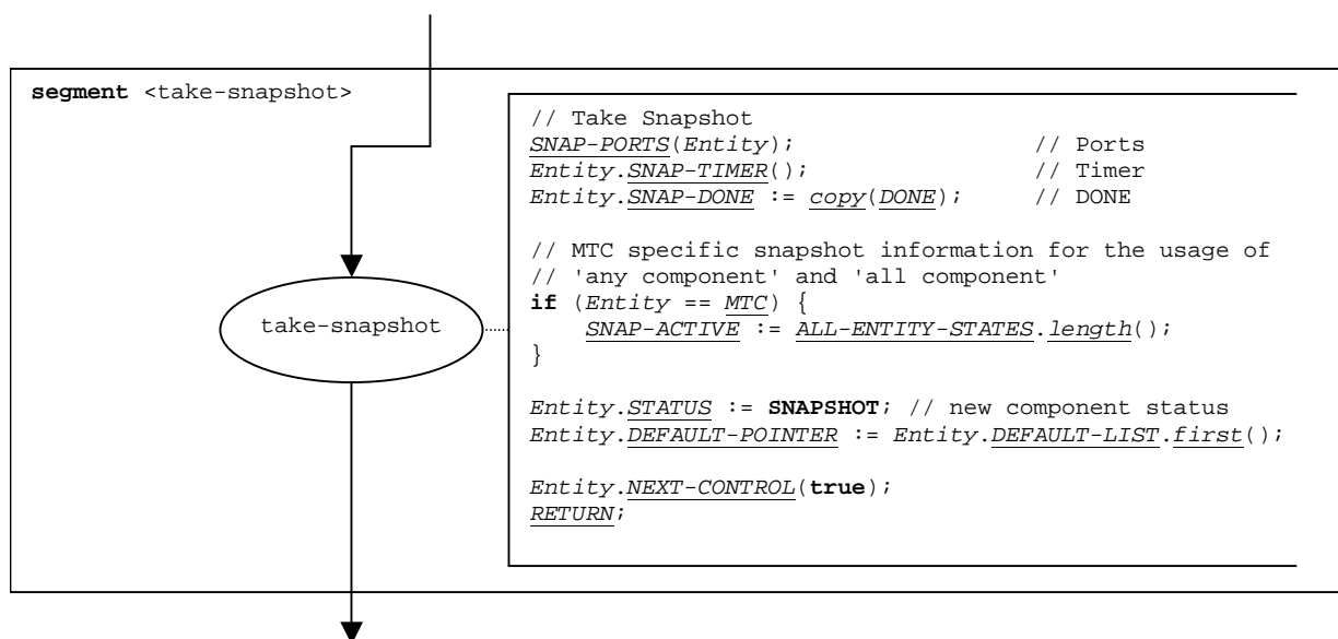
Figure 39: Flow graph segment &lt;take-snapshot&gt;
