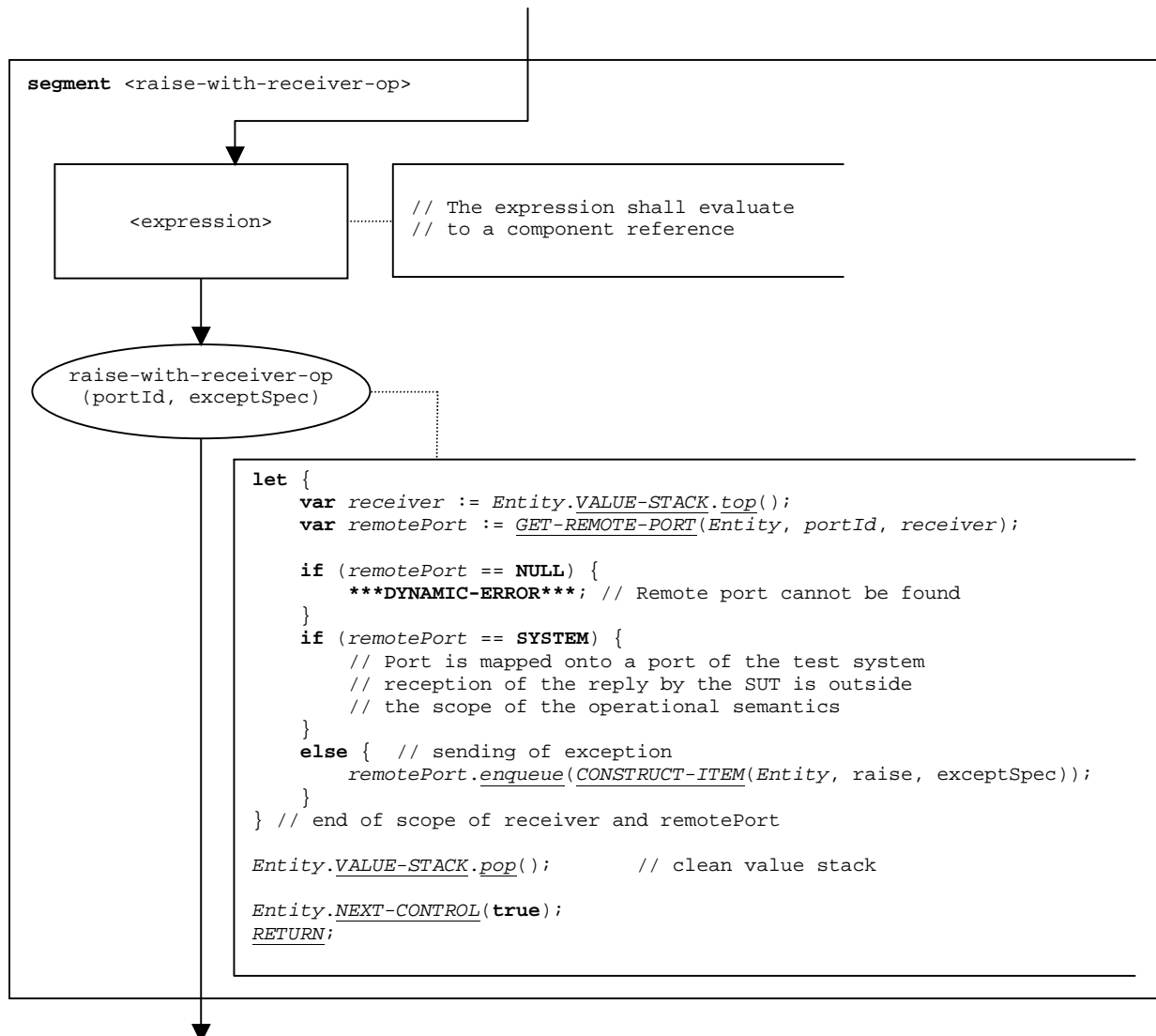
Figure 97: Flow graph segment <raise-with-receiver-op>
