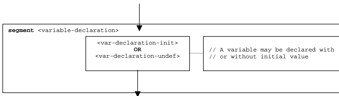
Figure 139: Flow graph segment <variable-declaration>
