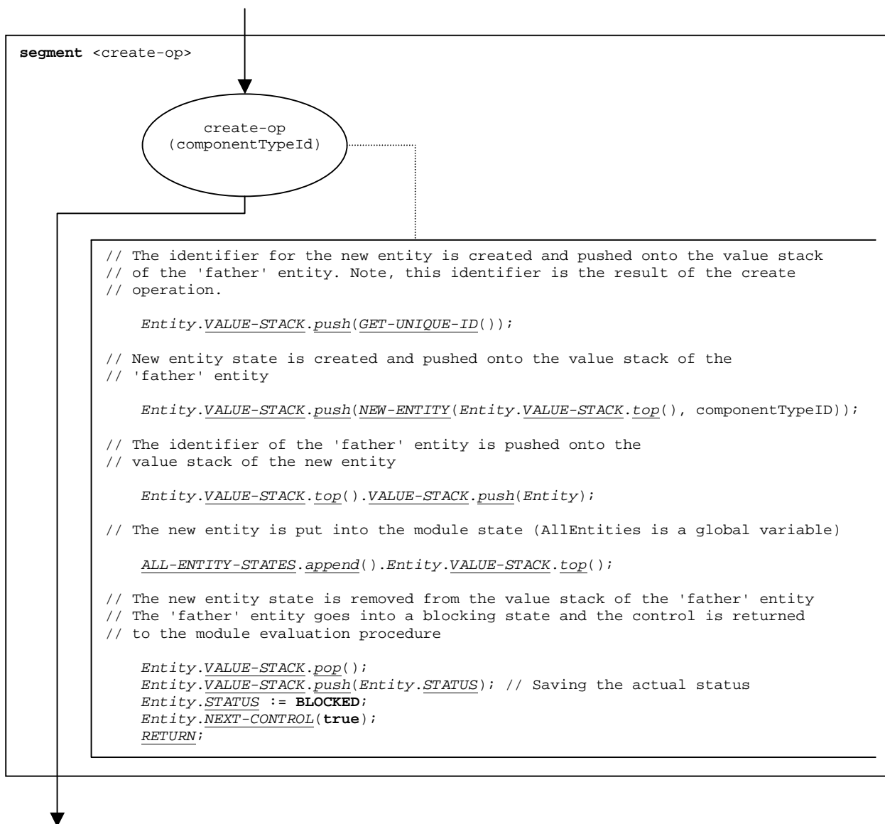
Figure 62: Flow graph segment <create-op>
