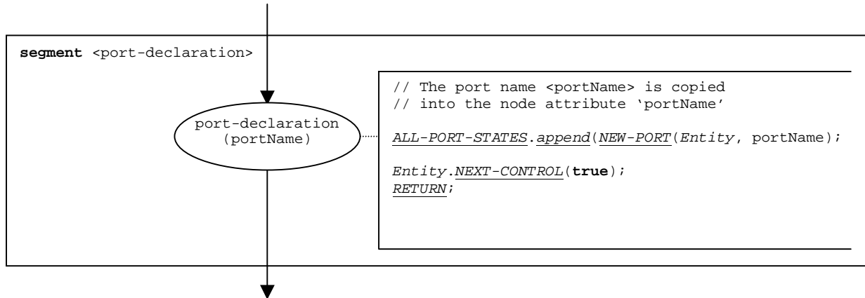
Figure 95: Flow graph segment <port-declaration>
