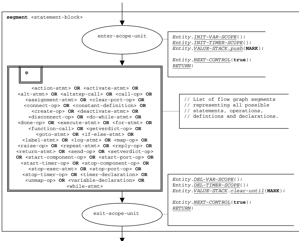
Figure 78: Flow graph segment <statement-block>
