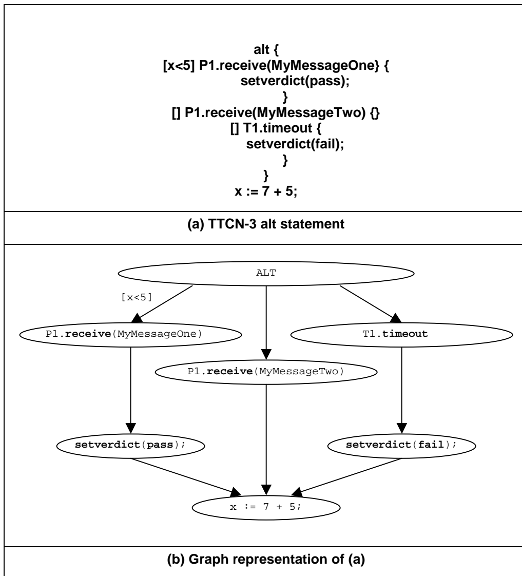
Figure 4: Graph representation of a TTCN-3 alt statement
