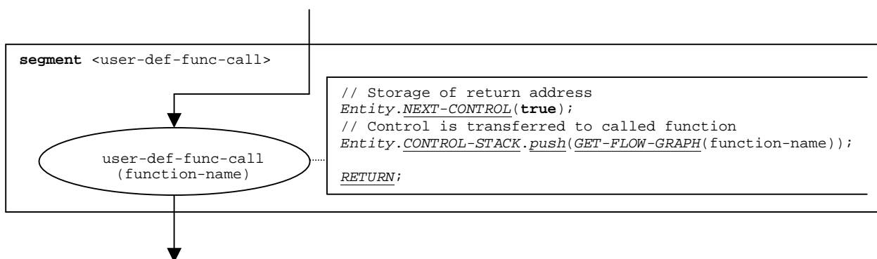
Figure 84: Flow graph segment <user-def-func-call>
