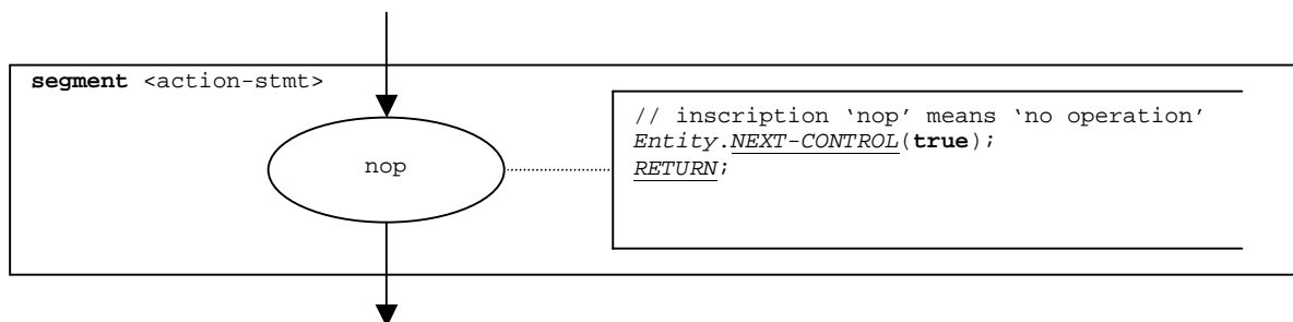
Figure 36: Flow graph segment <action-stmt>
