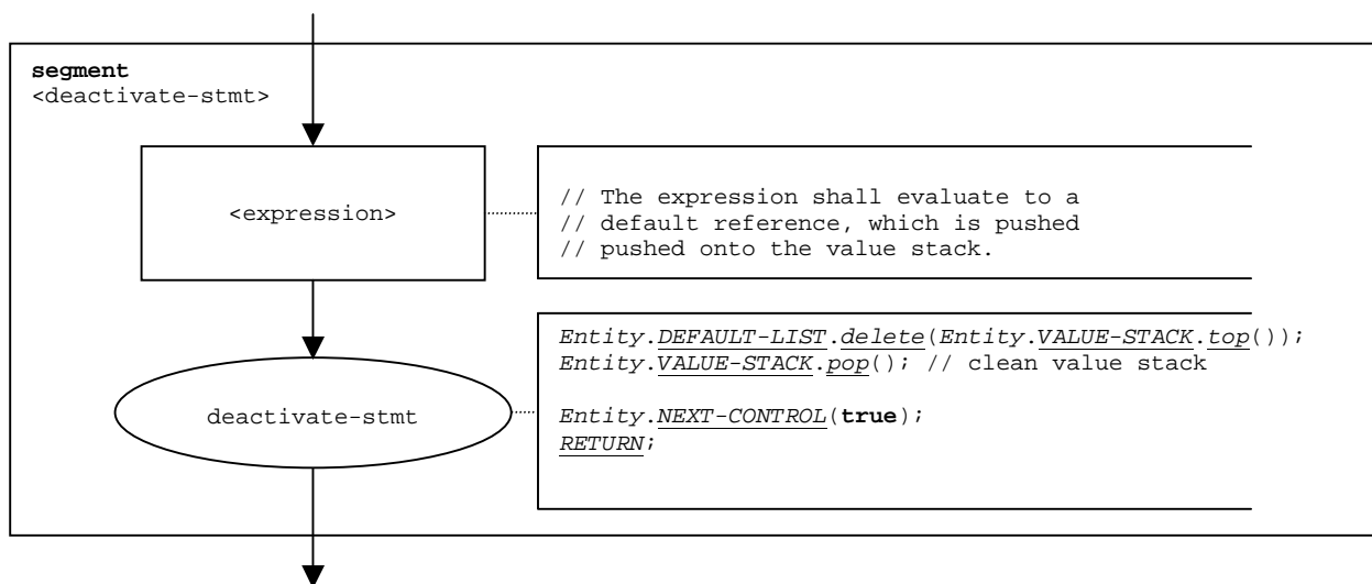
Figure 63: Flow graph segment <deactivate-stmt>
