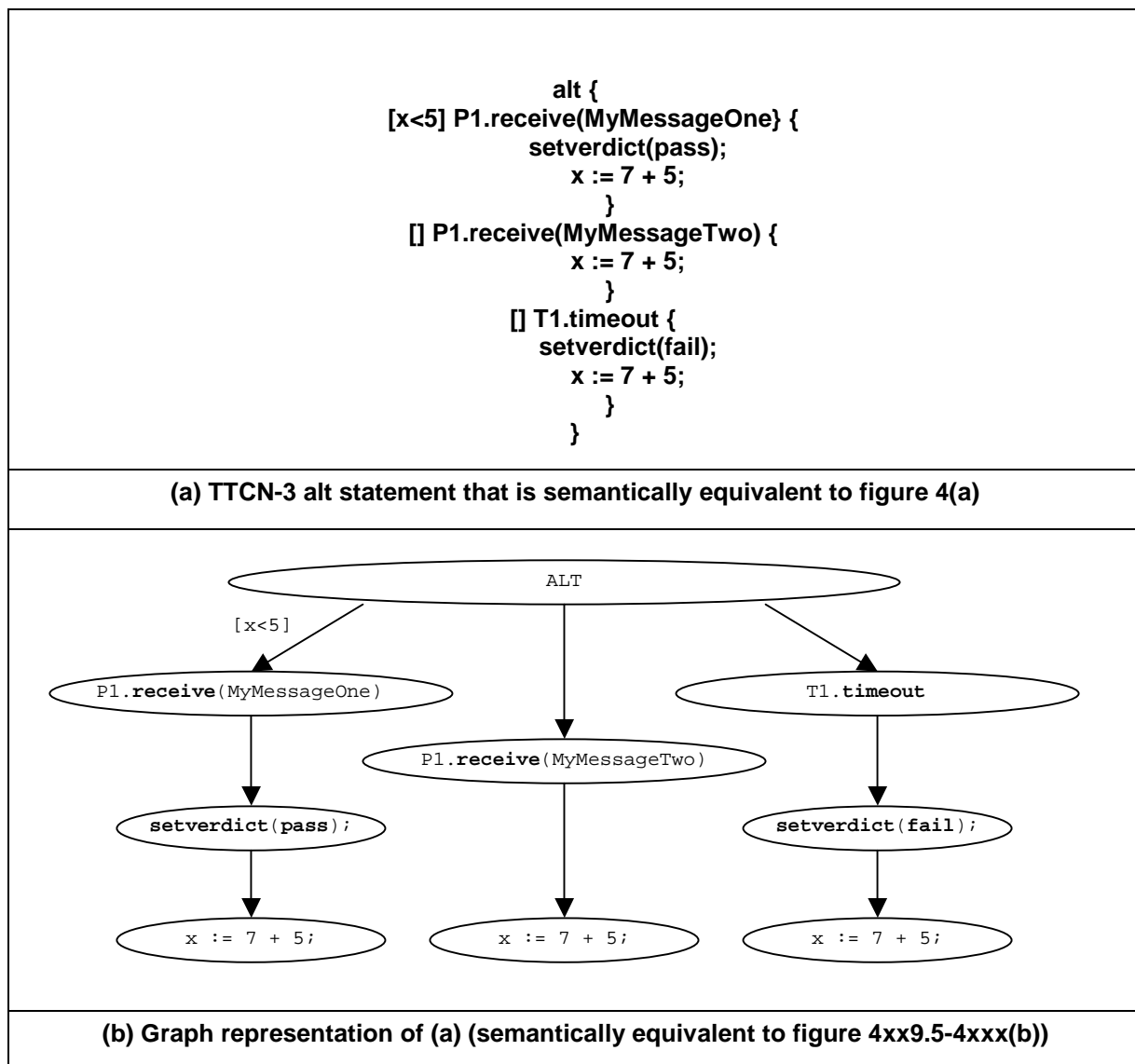
Figure 5: Graph representation of a TTCN-3 alt statement
