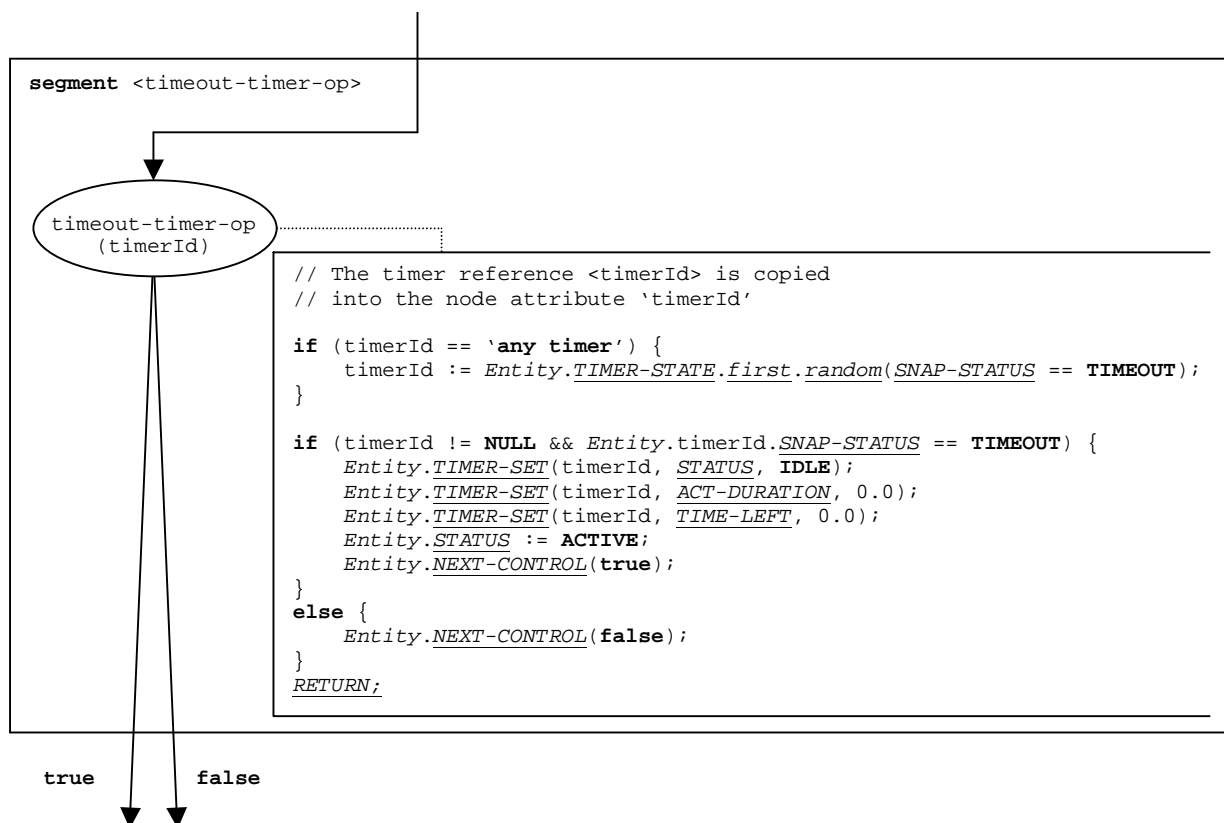
Figure 137: Flow graph segment <timeout-timer-op>
