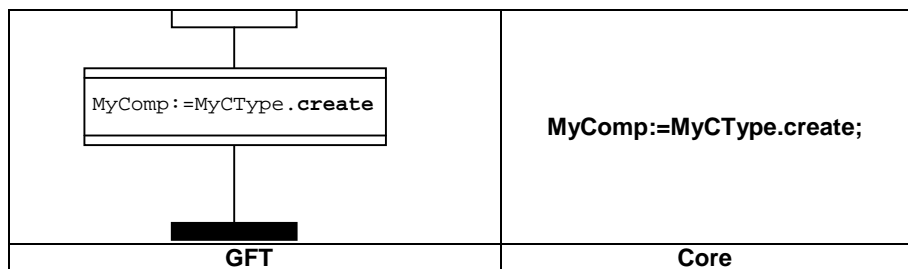
Figure 41: Create operation
