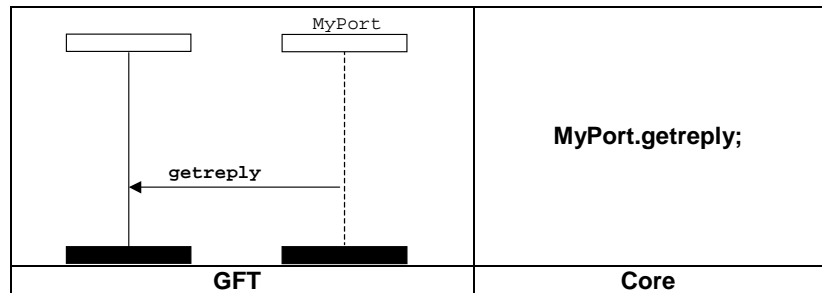
Figure 79: Getreply from any call (outside a call symbol)
