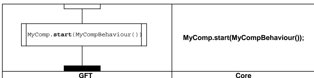
Figure 44: Start operation
