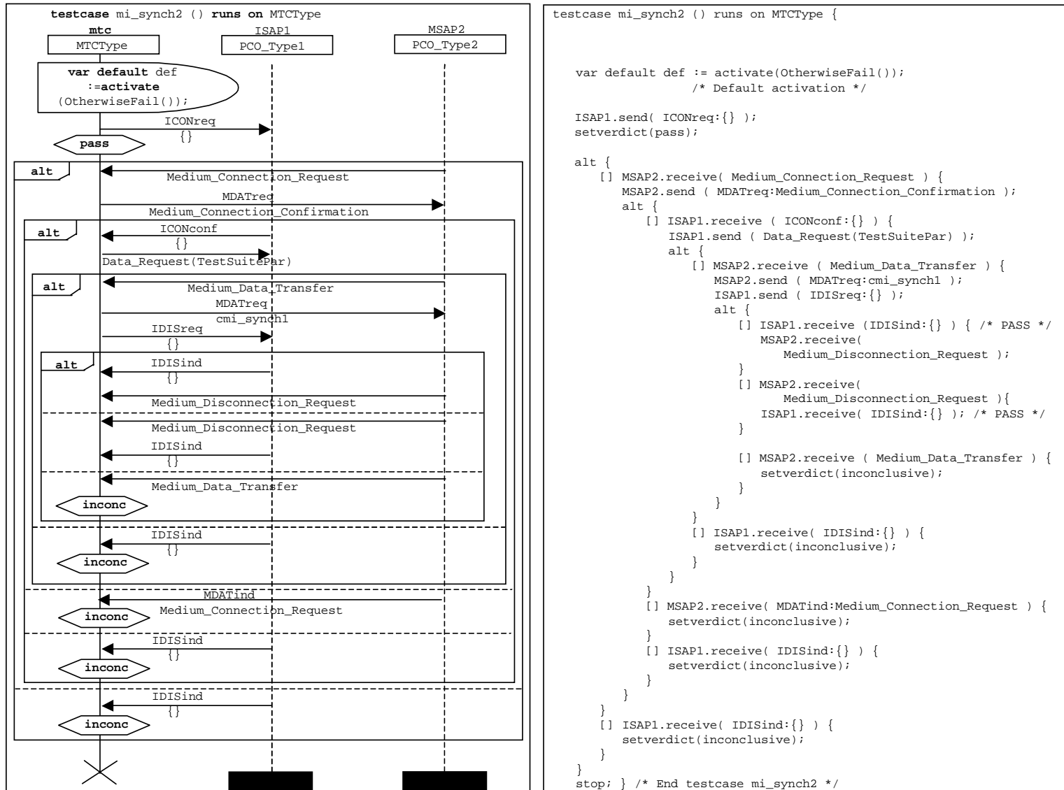
Figure C.12: INRES example - mi_synch2 test case
