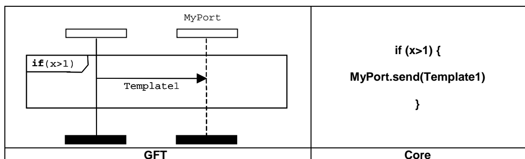
Figure 24: If-Statement
