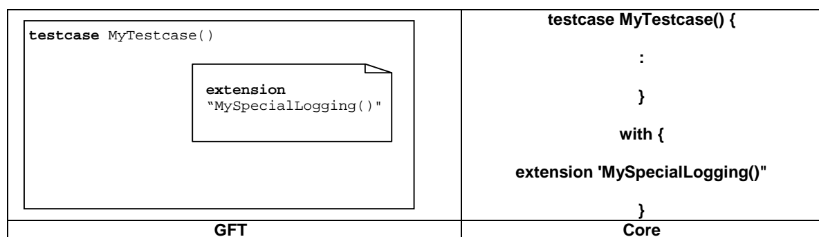
Figure 112: Specifying attributes
