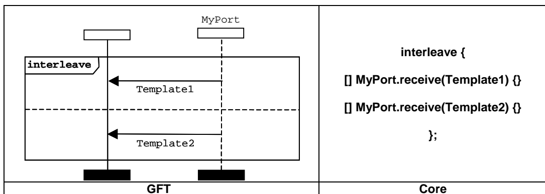
Figure 36: Interleave statement
