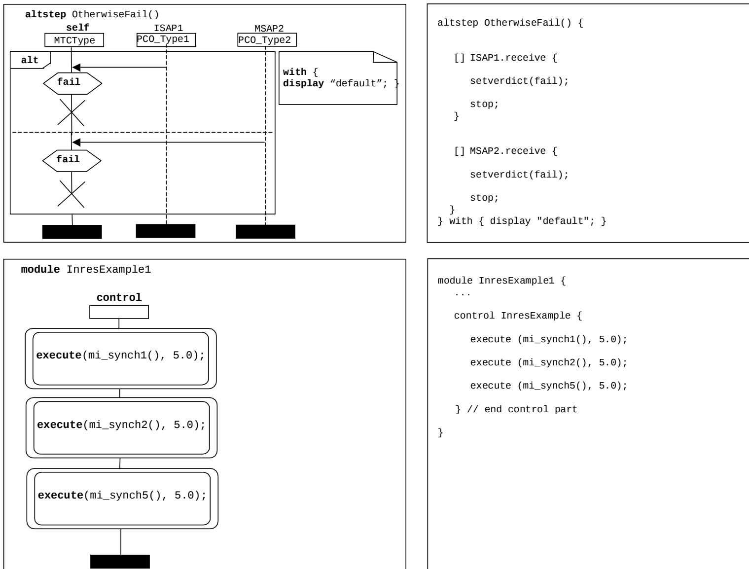
Figure E.15: INRES example - OtherwiseFail altstep and InresExample1 module definitions
