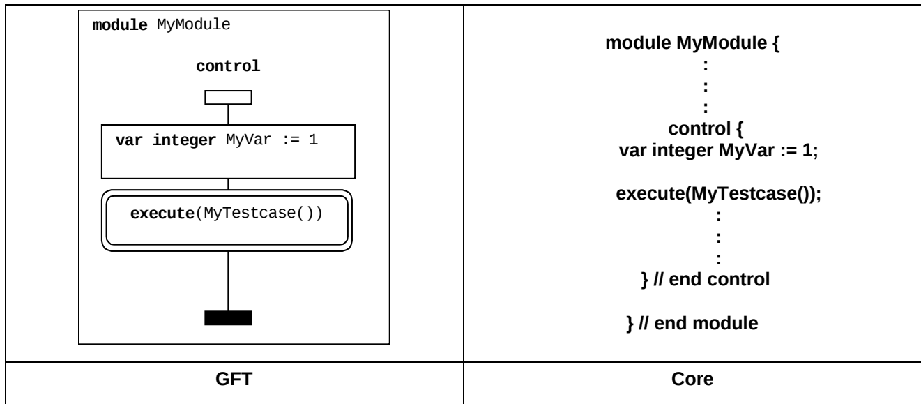
Figure 9: Principle shape of a GFT control diagram and corresponding core language
