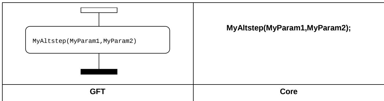
Figure 19: Altstep invocation
