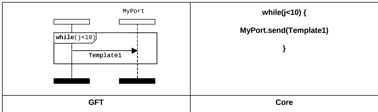
Figure 27: While Statement
