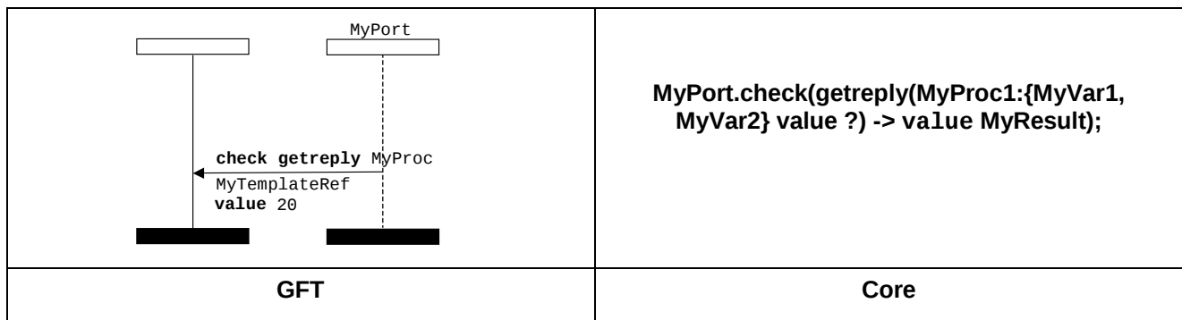
Figure 95: Check a getreply (outside a call symbol)
