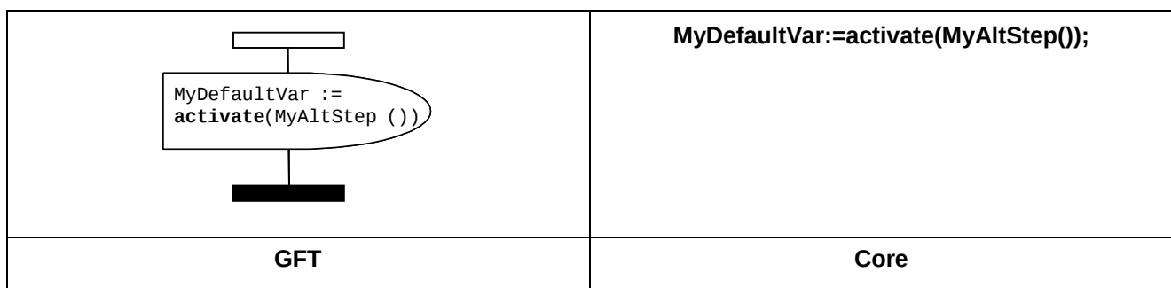
Figure 39: Default activation
