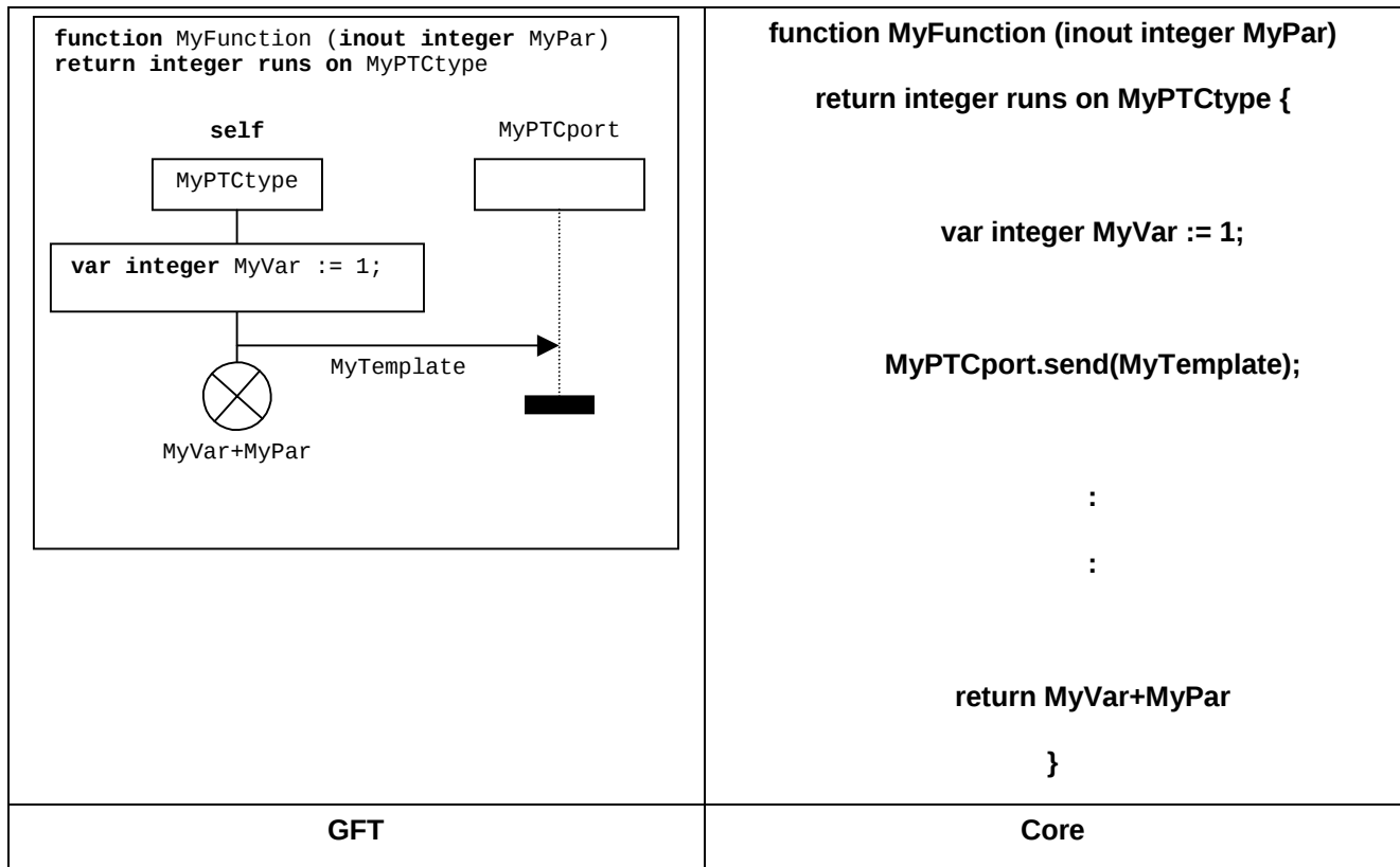
Figure 11: Principle shape of a GFT function diagram and corresponding core language
