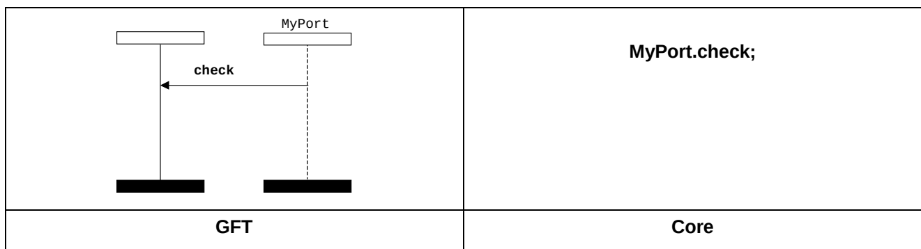
Figure 96: Check any operation
