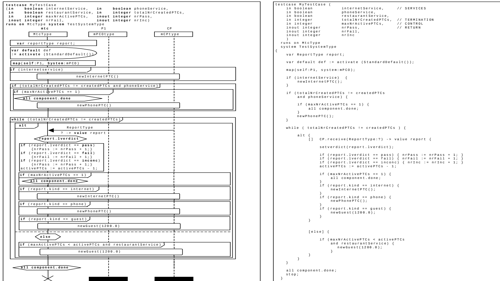
Figure E.1: Restaurant example – MyTestCase test case
