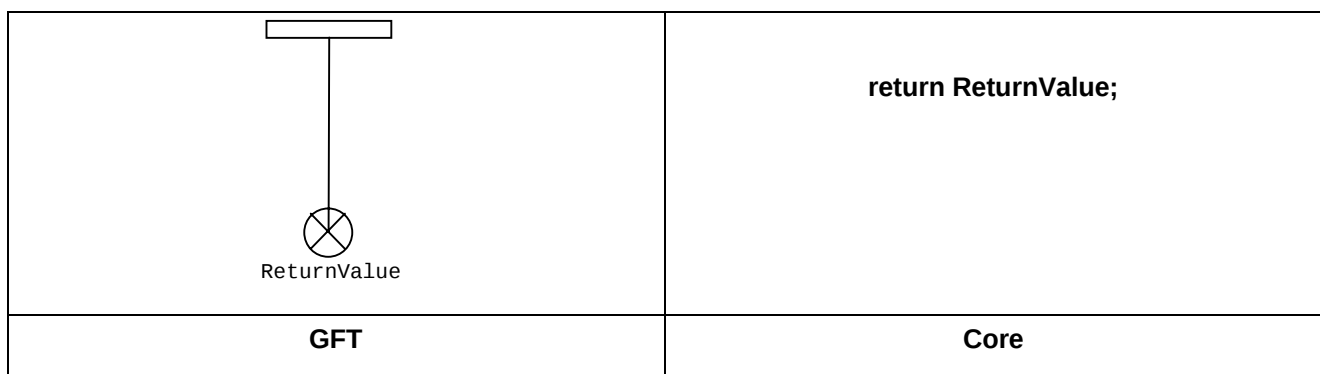
Figure 38: Return symbol with a return value
