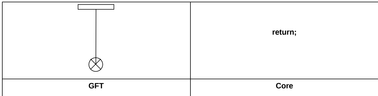
Figure 37: Return symbol without a return value
