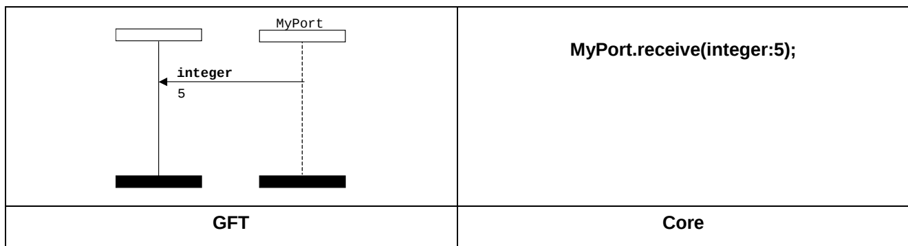
Figure 55: Receive operation with inline template
