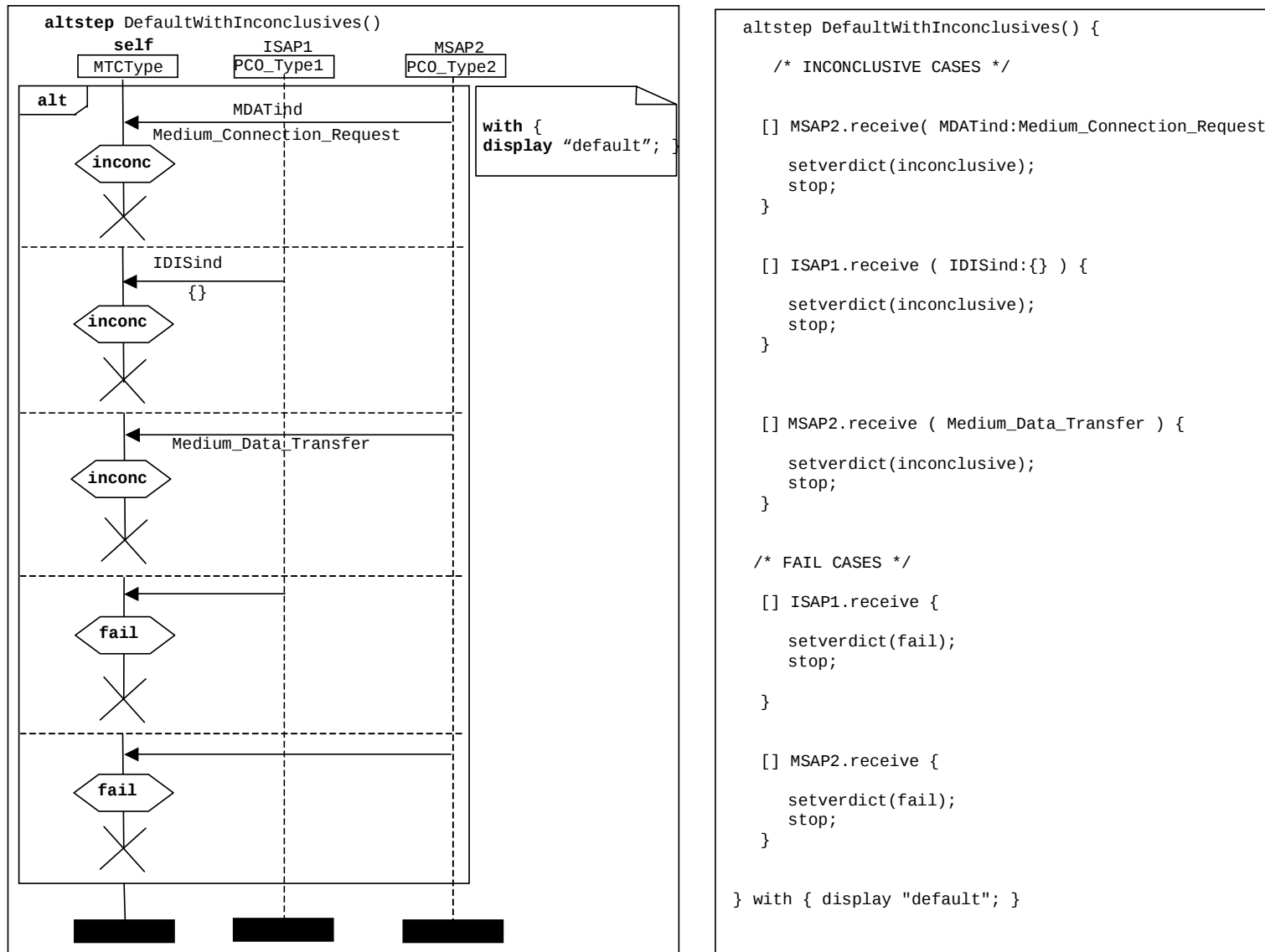
Figure E.14: INRES example - DefaultWithInconclusives altstep
