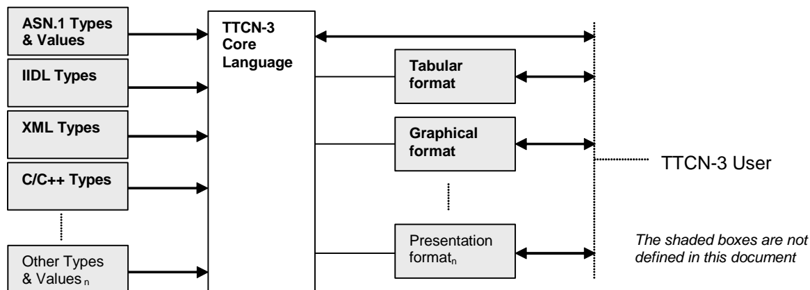
Figure 1: User's view of the core language and the various presentation formats
