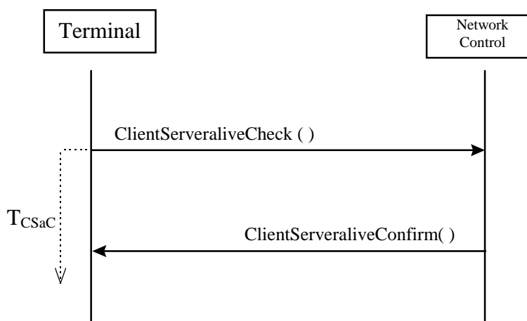
Figure 8: Client initiated alive check sequence
