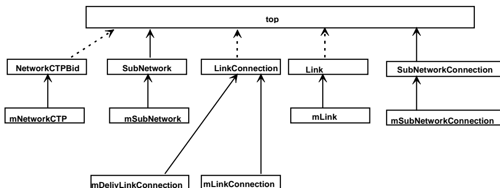
Figure 29: Inheritance tree
