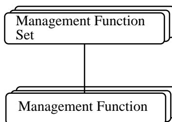
Figure 12: Decomposition hierarchy
