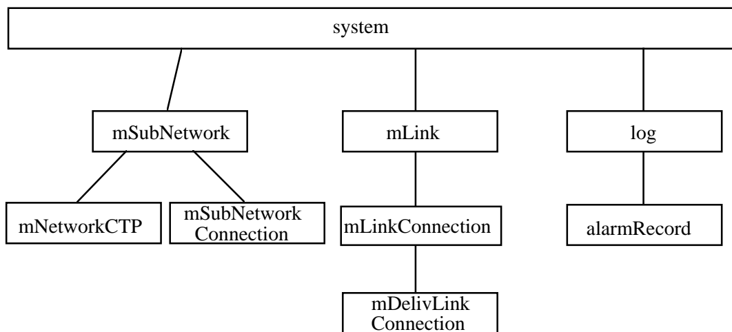
Figure 28: Naming tree
