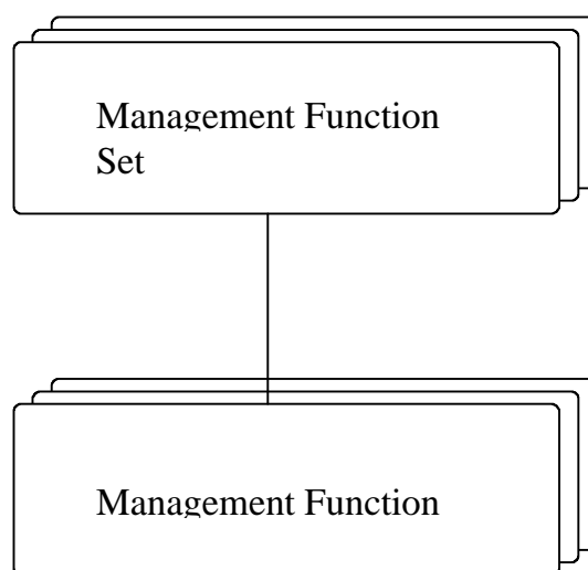
Figure 21: Decomposition hierarchy
