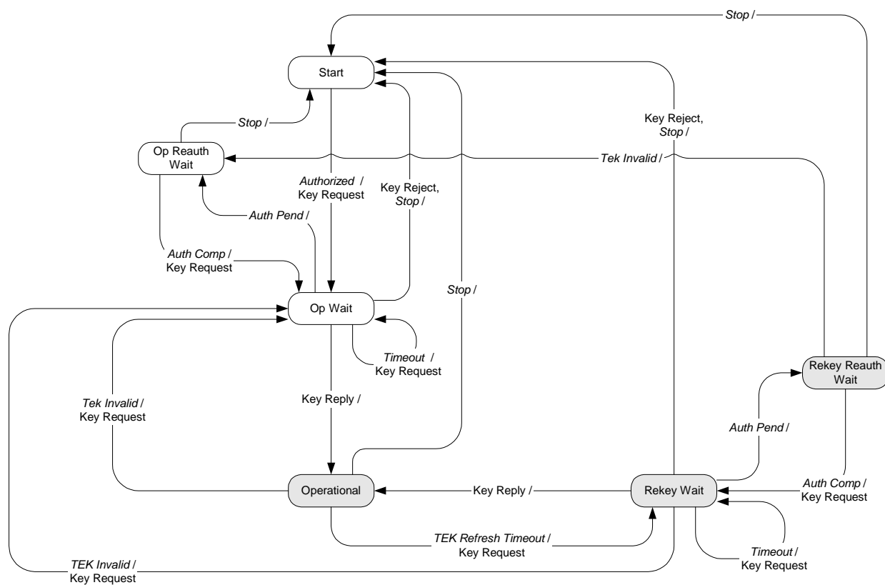
Figure 7.2: TEK state machine flow diagram
