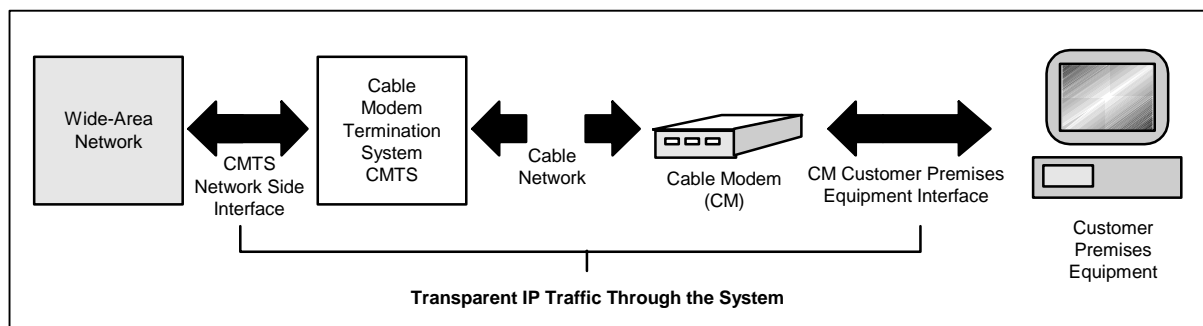
Figure 4.1: Transparent IP traffic through the Data Over Cable system
