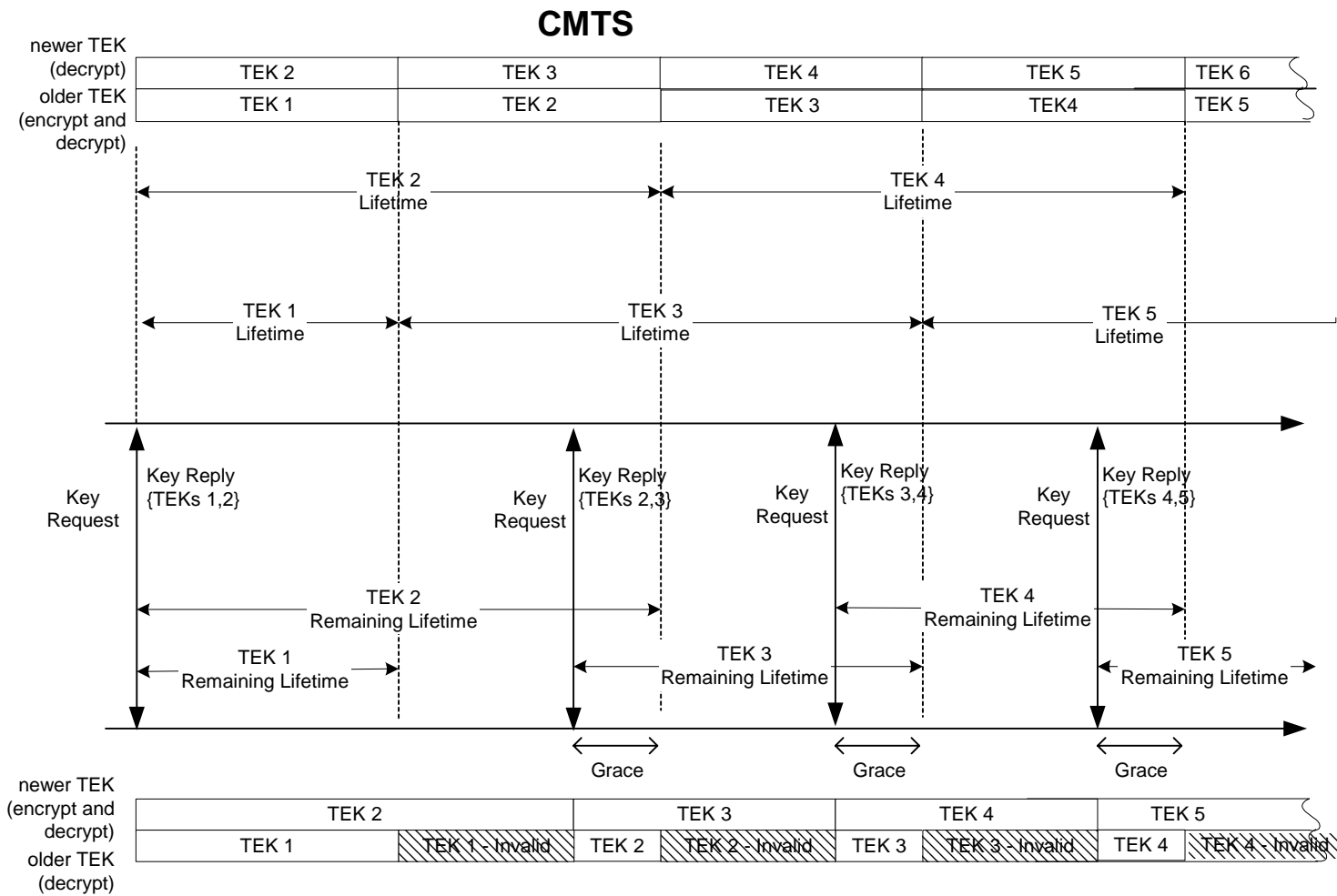
Figure 9-2: TEK Management in CMTS and CM
