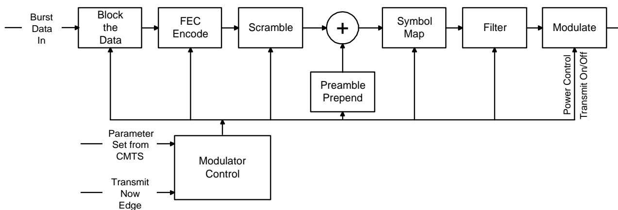
Figure 6.9: Signal-processing sequence
