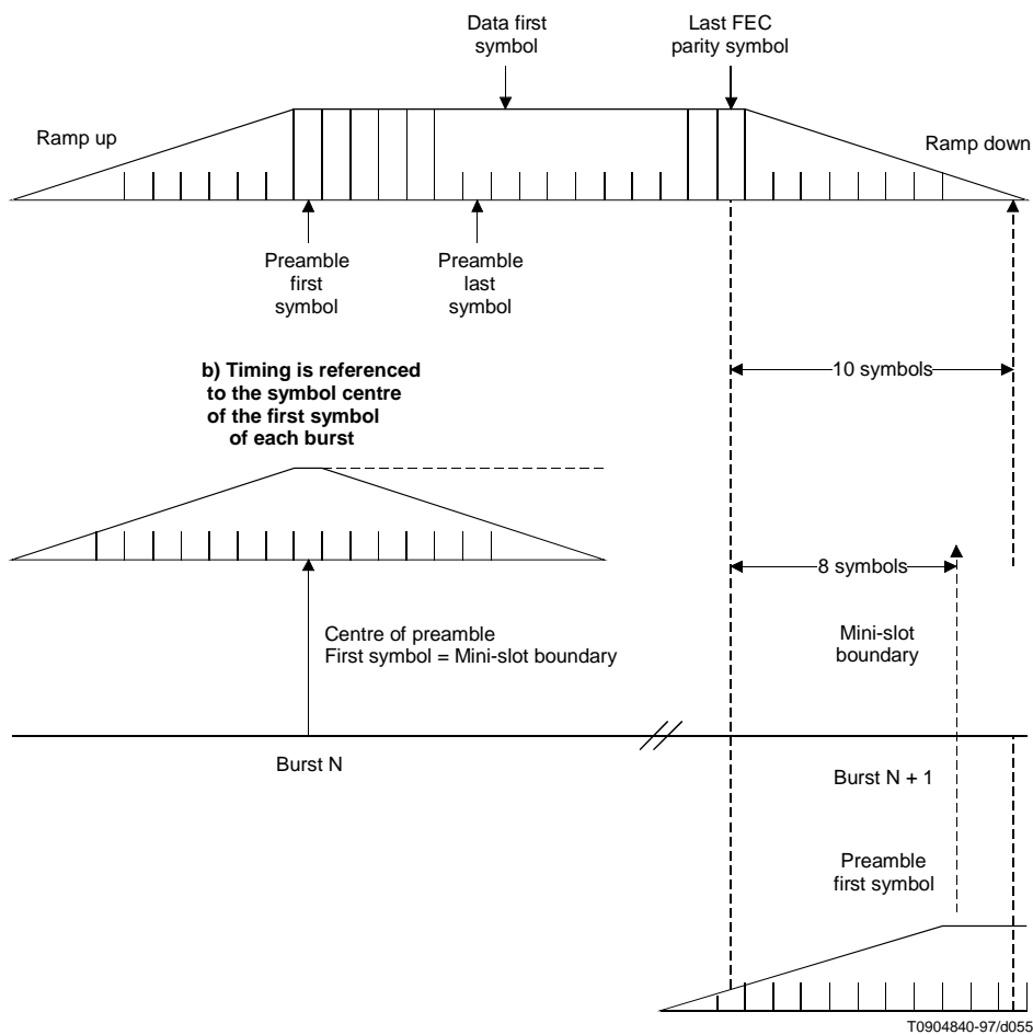
Figure N.6: Nominal burst timing
