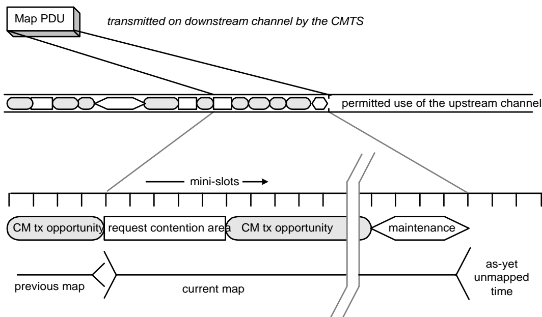
Figure 9.1: Allocation map
