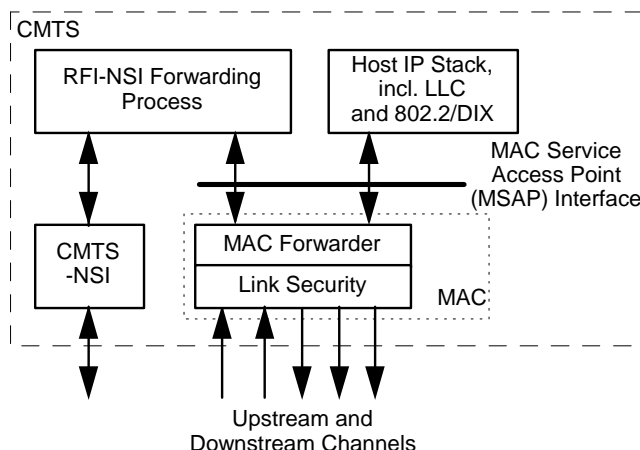
Figure 5.4: MAC forwarder
