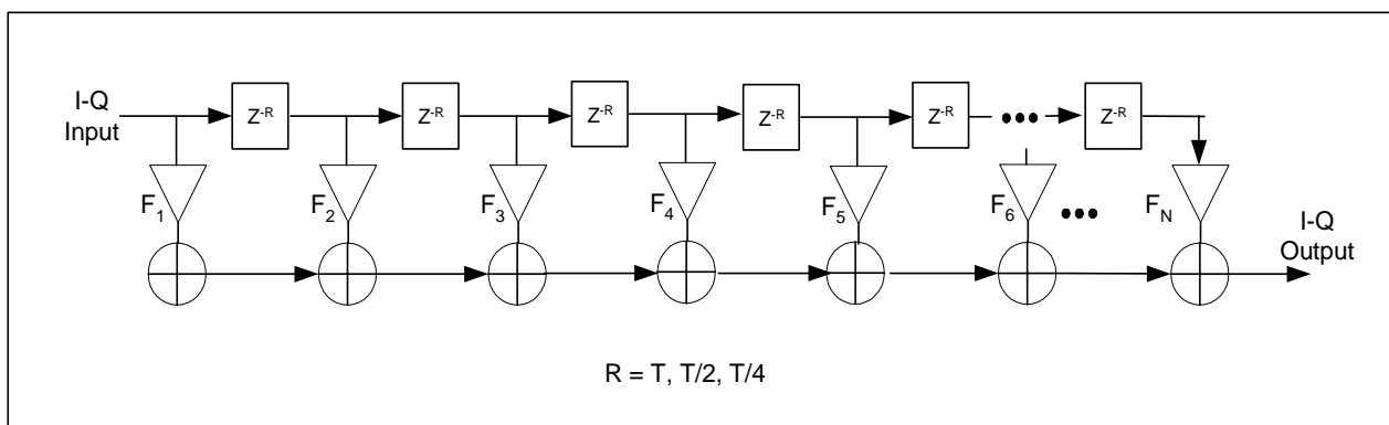
Figure 6.5: Transmit pre-equalizer structure
