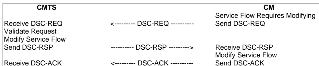
Figure 11.39: CM-initiated DSC
