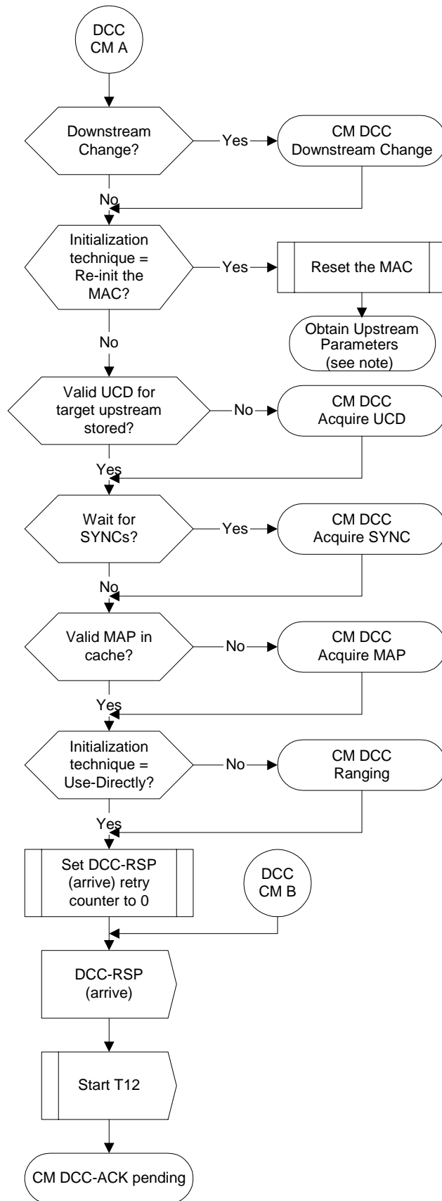
Figure 11.63: Dynamically changing channels: CM view part 2
