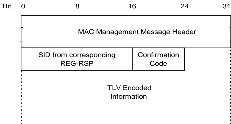
Figure 8.28: Registration - Acknowledgment
