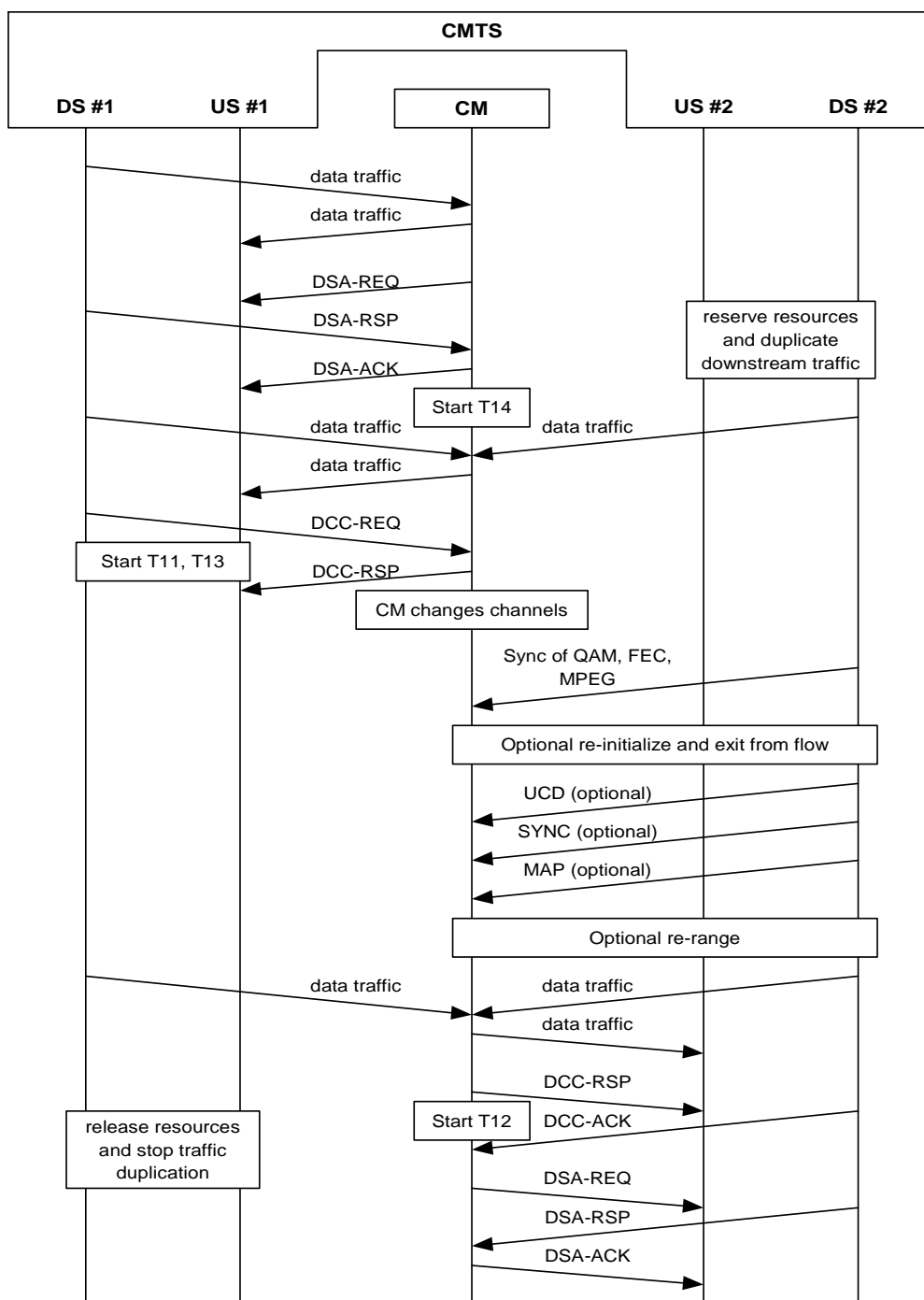
Figure 11.57: DCC example operational flow
