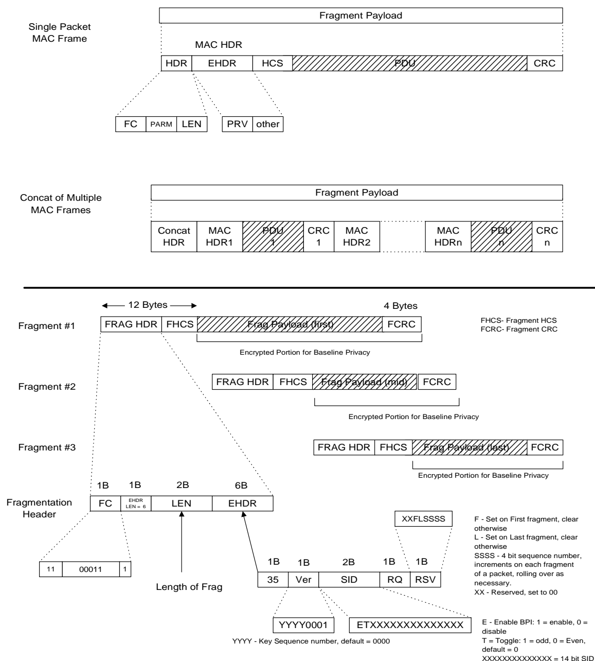
Figure 8.13: Fragmentation details
