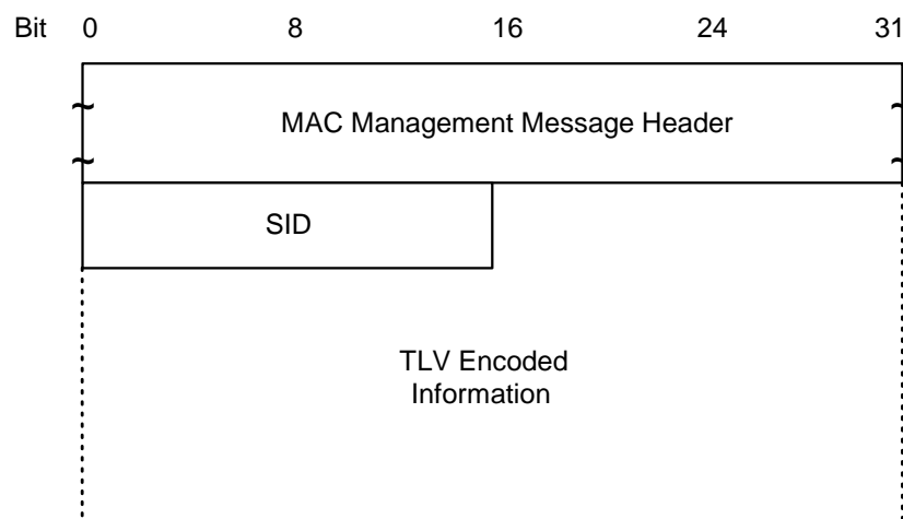
Figure 8.26: Registration - Request
