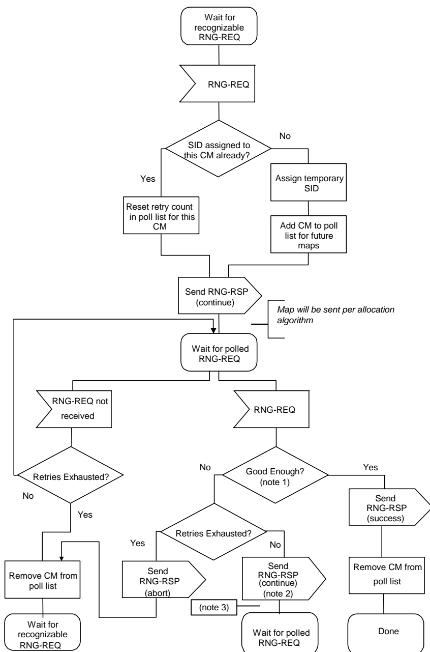
Figure 11.8: Initial ranging - CMTS
