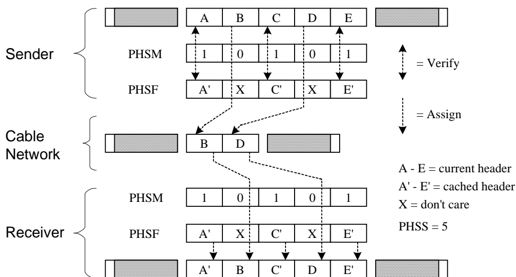
Figure 10.12: Payload Header Suppression with masking
