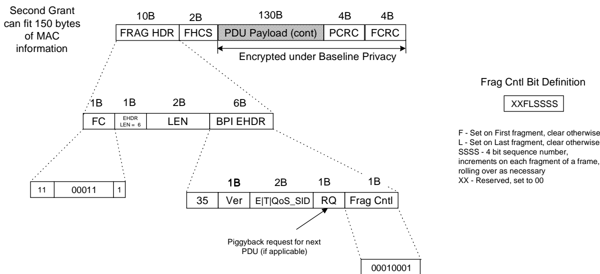
Figure 10.9: Example of fragmenting a single packet
