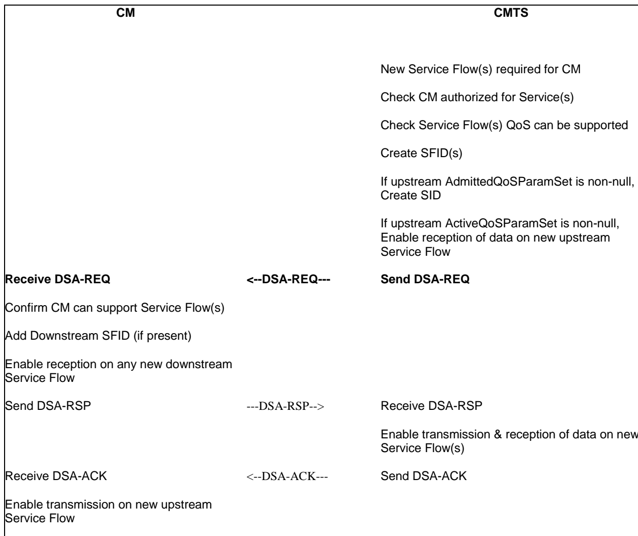
Figure 11-29: Dynamic Service Addition Initiated from CMTS
