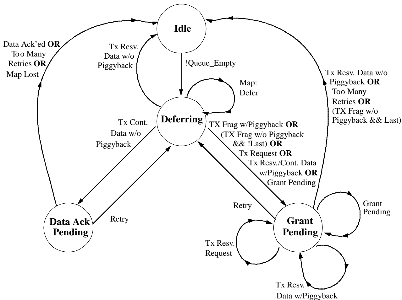
Figure K-1: Transmission & Deference State Transition Diagram
