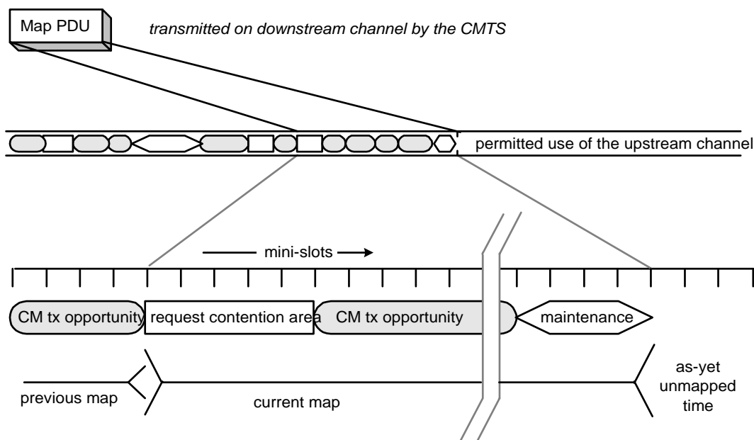
Figure 9-1: Allocation Map
