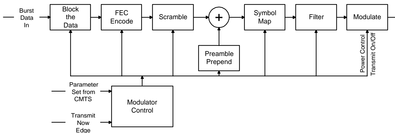
Figure N-9: Signal-processing sequence
