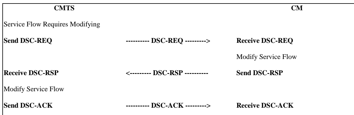
Figure 11-40: CMTS-Initiated DSC
