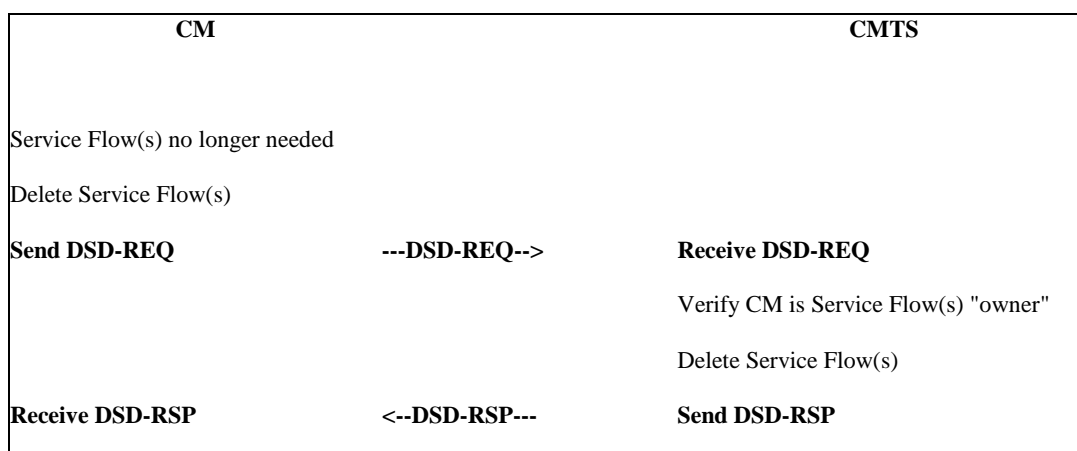
Figure 11-50: Dynamic Service Deletion Initiated from CM
