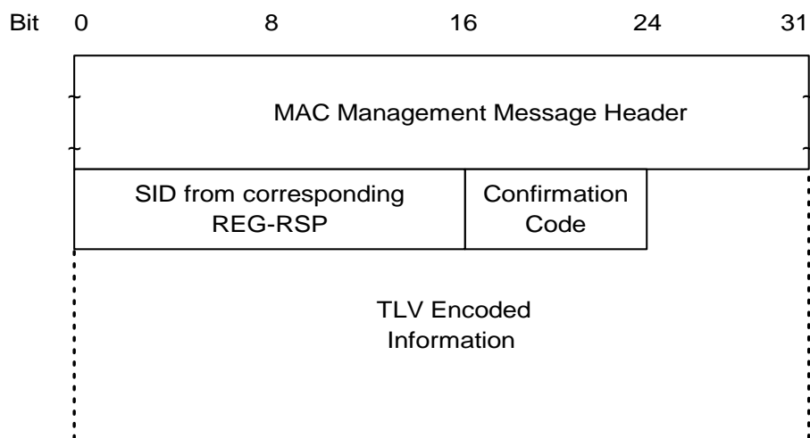
Figure 8-28: Registration Acknowledgment
