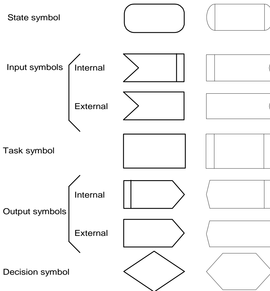
Figure 11-2: SDL Notation
