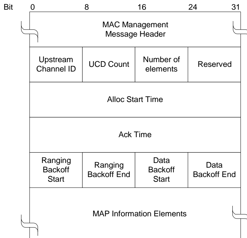
Figure 8-19: MAP Format
