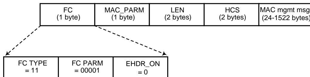
Figure 8-7: Management MAC Header
