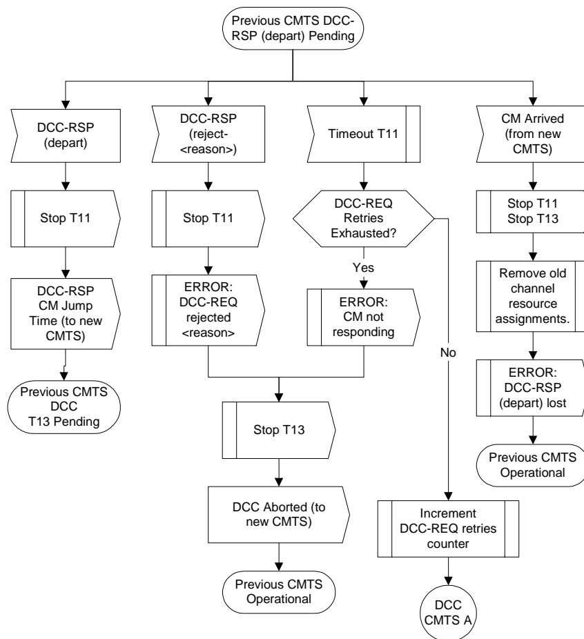
Figure 11-59: Dynamically Changing Channels: CMTS View Part 2
