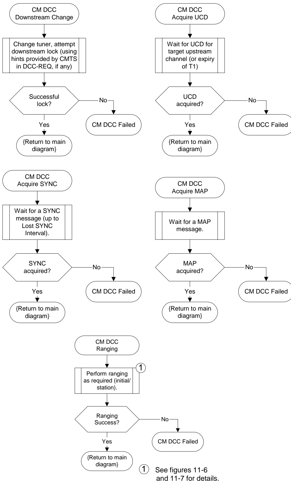
Figure 11-64: Dynamically Changing Channels: CM View Part 3
