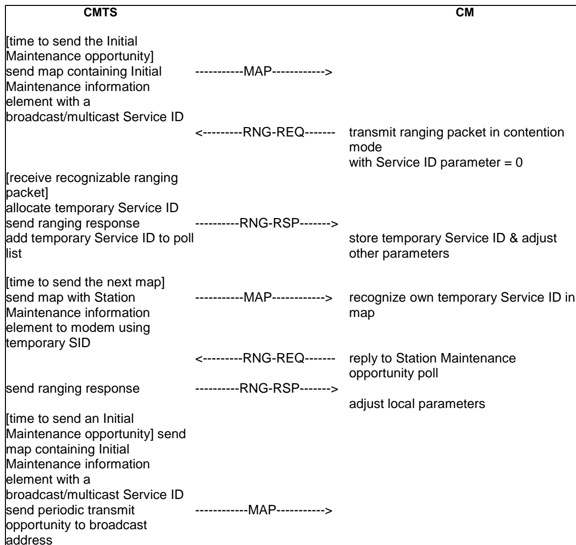
Figure 11-5: Ranging and Automatic Adjustments Procedure
