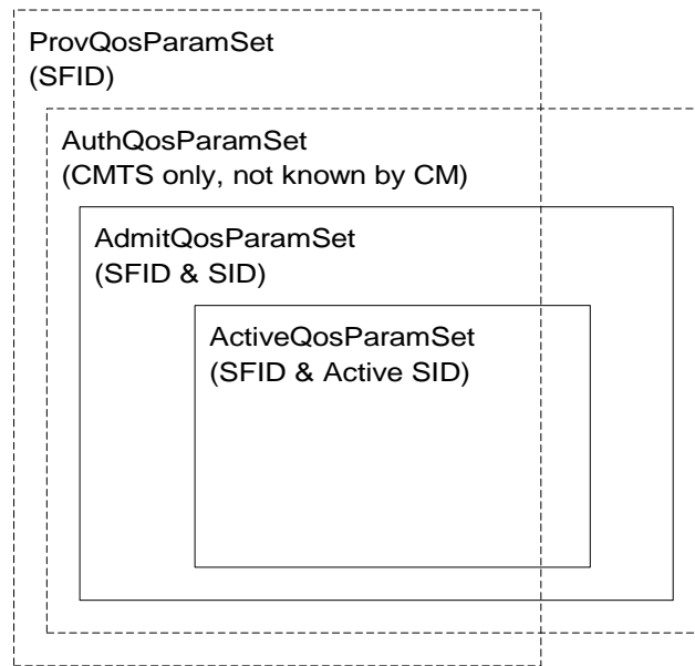
Figure 10-2: Dynamic Authorization Model 'Envelopes'
