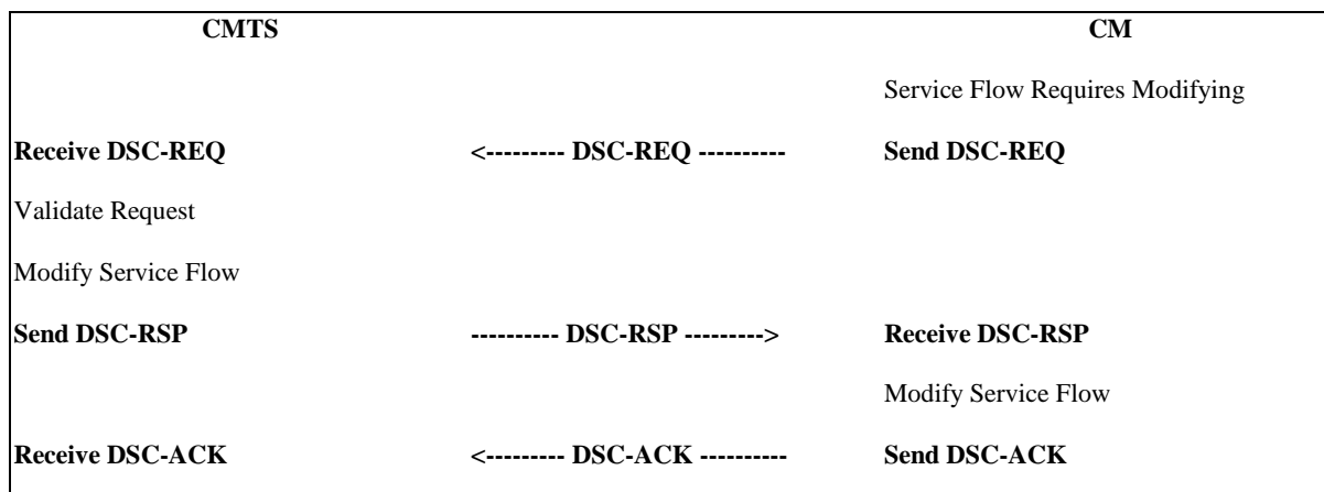
Figure 11-39: CM-Initiated DSC
