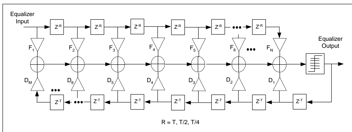
Figure 8-24: Generalized Equalizer Tap Location Definition
