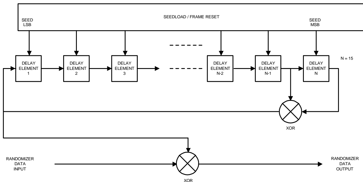
Figure N-4: Scrambler Structure
