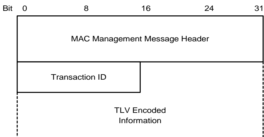
Figure 8-39: Dynamic Channel Change Request
