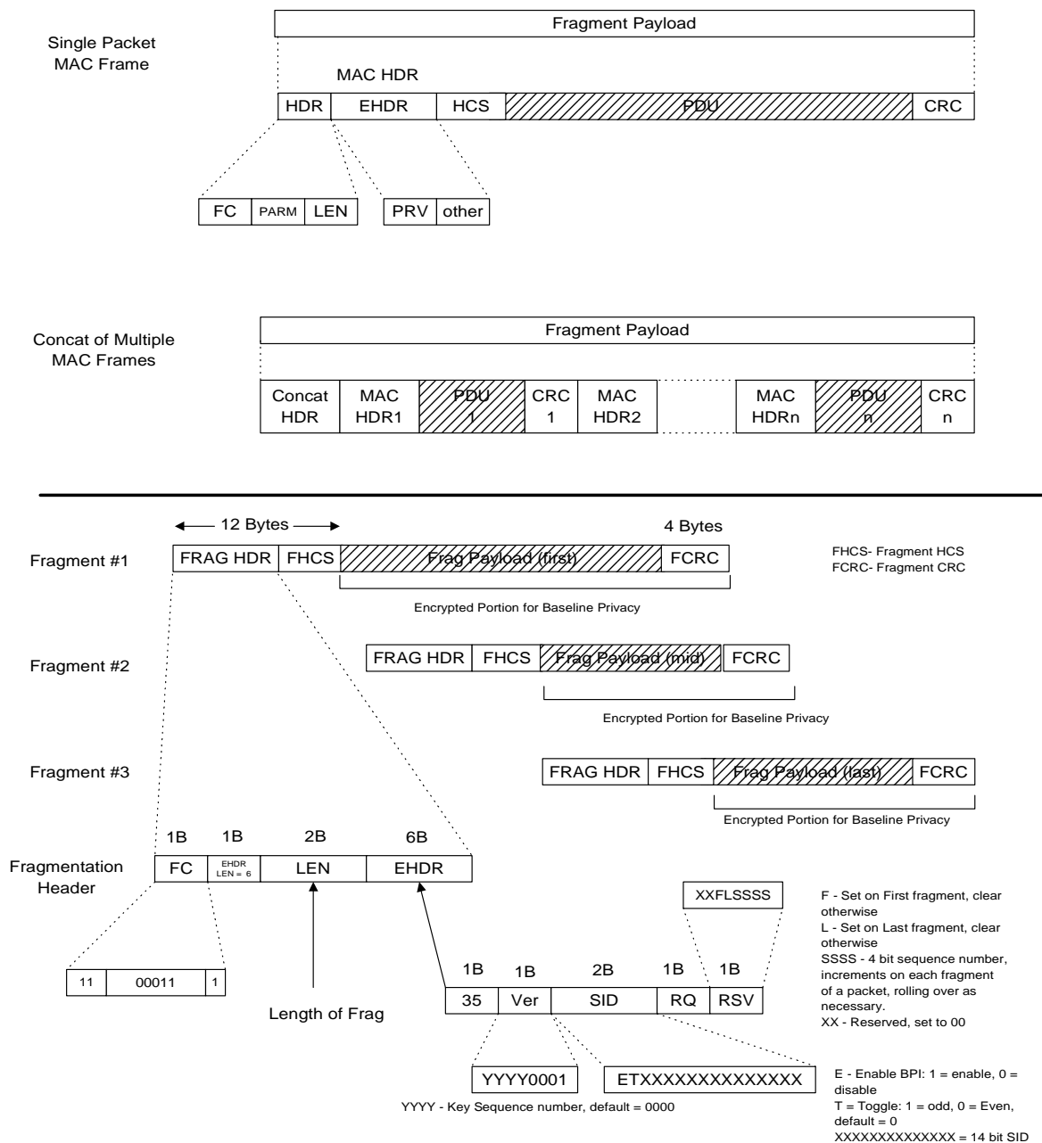
Figure 8-13: Fragmentation Details
