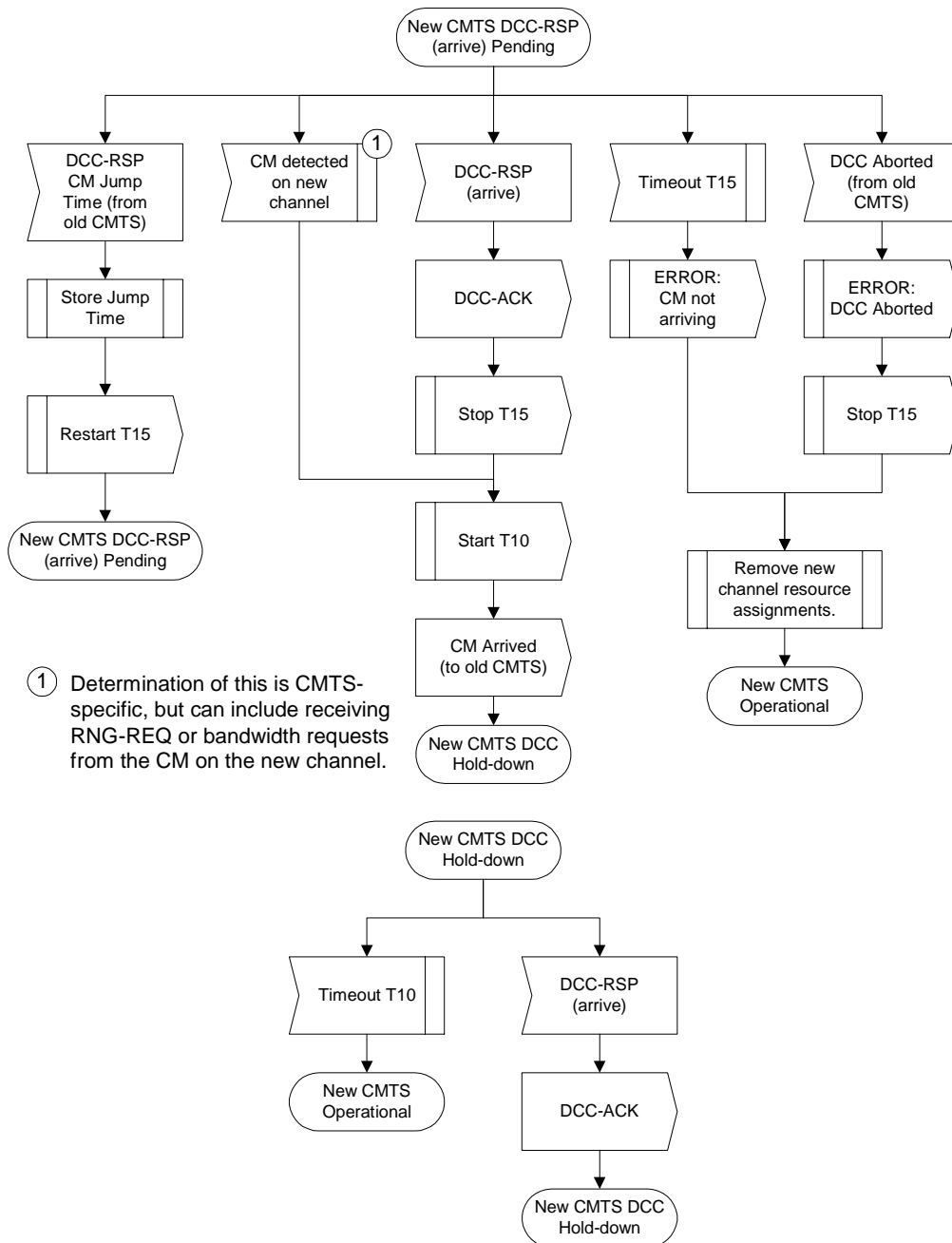
Figure 11-61: Dynamically Changing Channels: CMTS View Part 4
