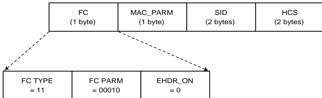
Figure 8-8: Request Frame Format
