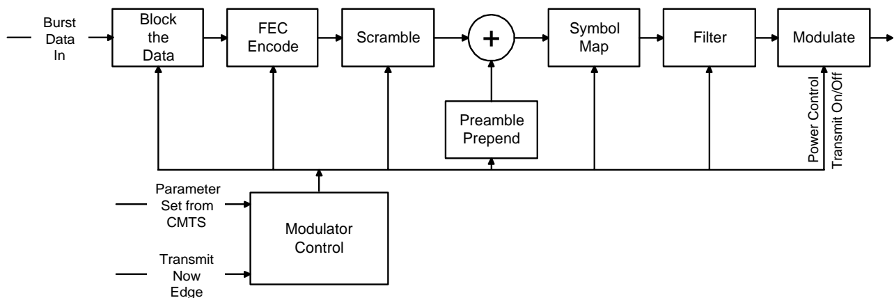
Figure 6-9: Signal-Processing Sequence
