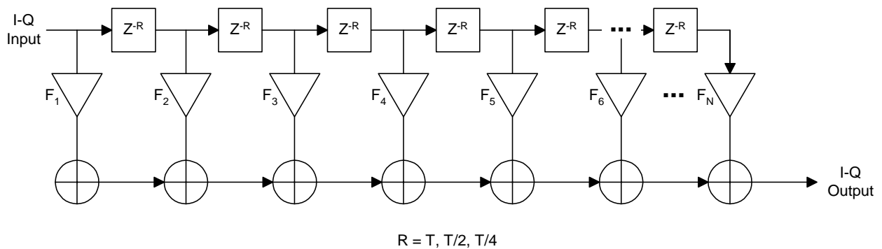
Figure N-5: Transmit Pre-Equalizer Structure
