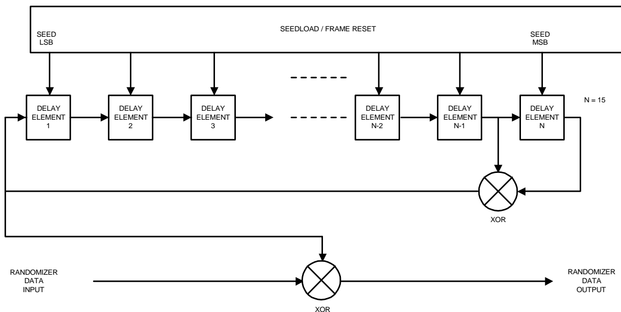
Figure 6-4: Scrambler Structure
