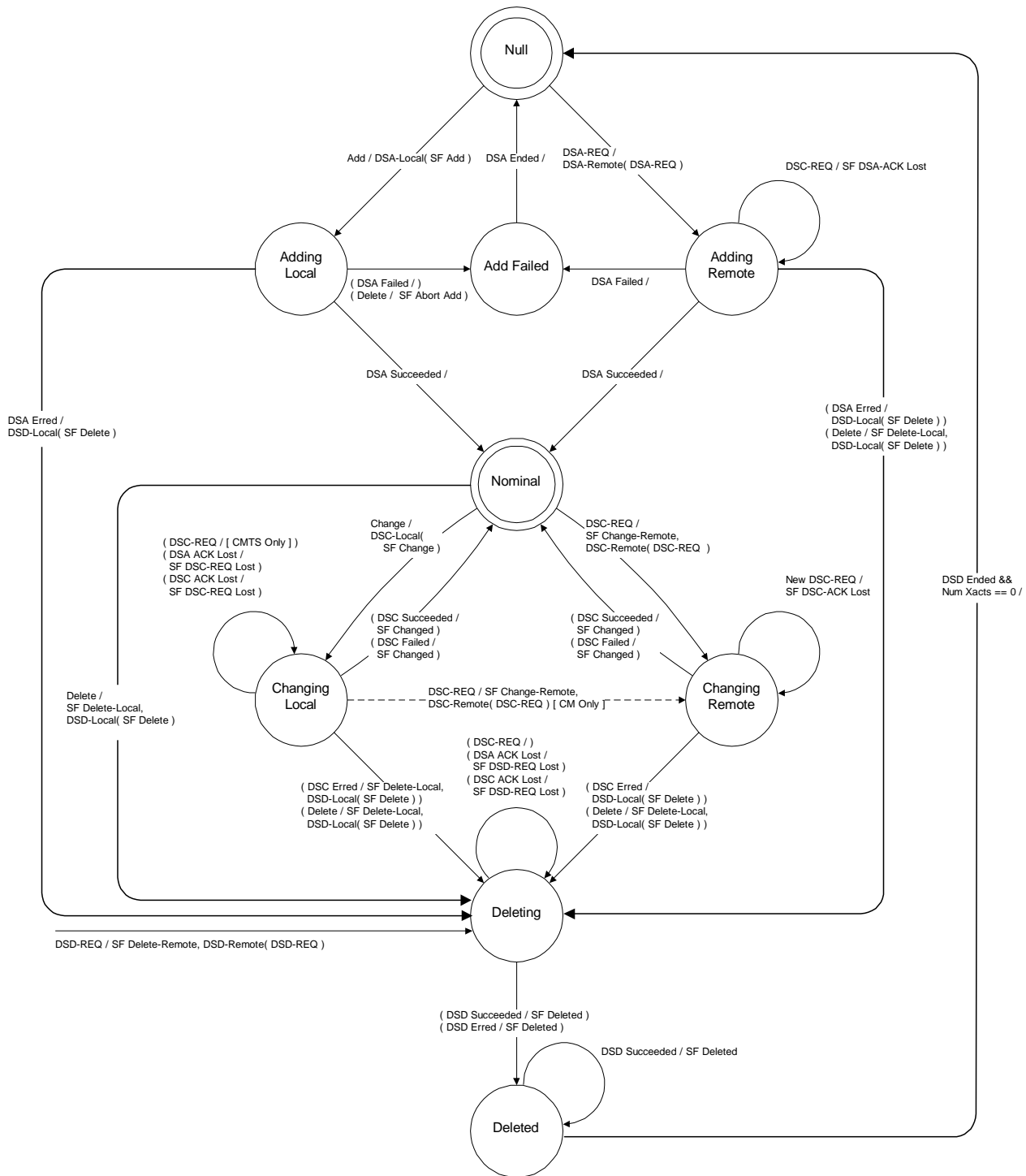
Figure 11–21: Dynamic Service Flow State Transition Diagram
