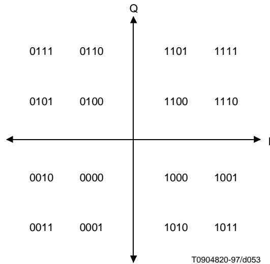
Figure N-3: 16QAM differential-coded symbol mapping
