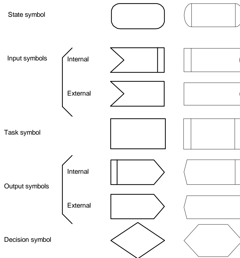
Figure 11-2: SDL Notation
