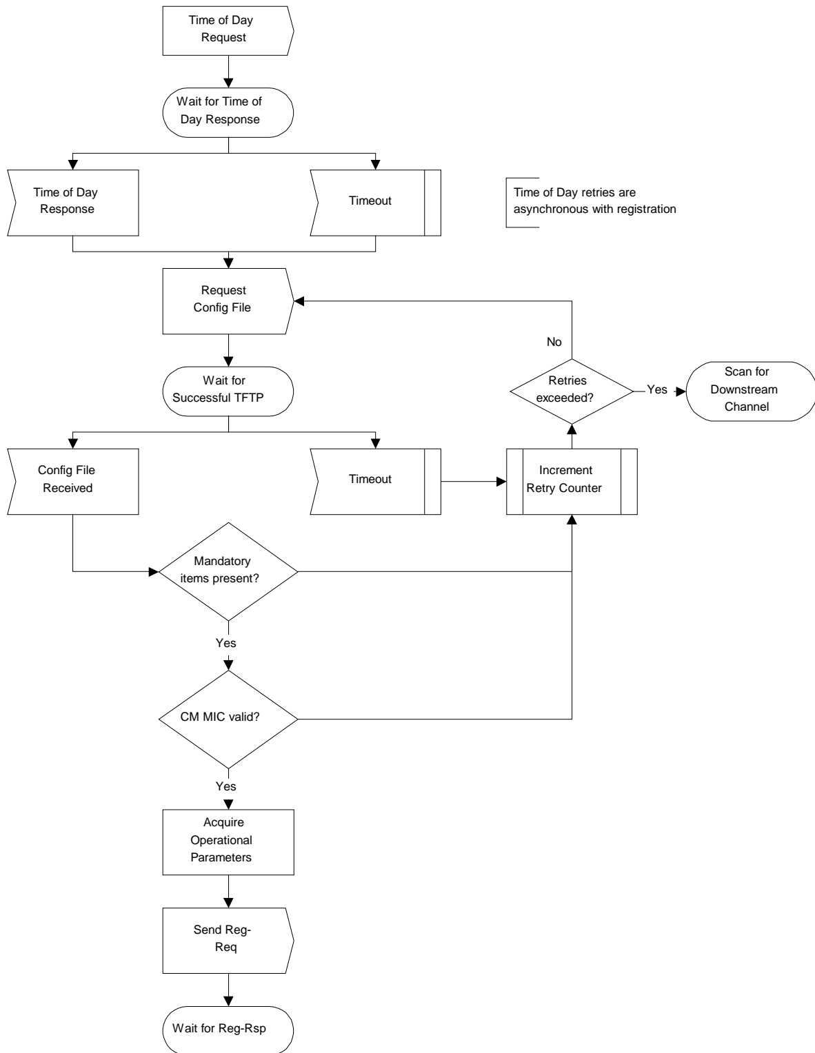
Figure 11-12: Registration - CM
