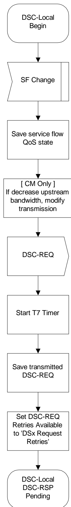
Figure 11–41: DSC - Locally Initiated Transaction Begin State Flow Diagram
