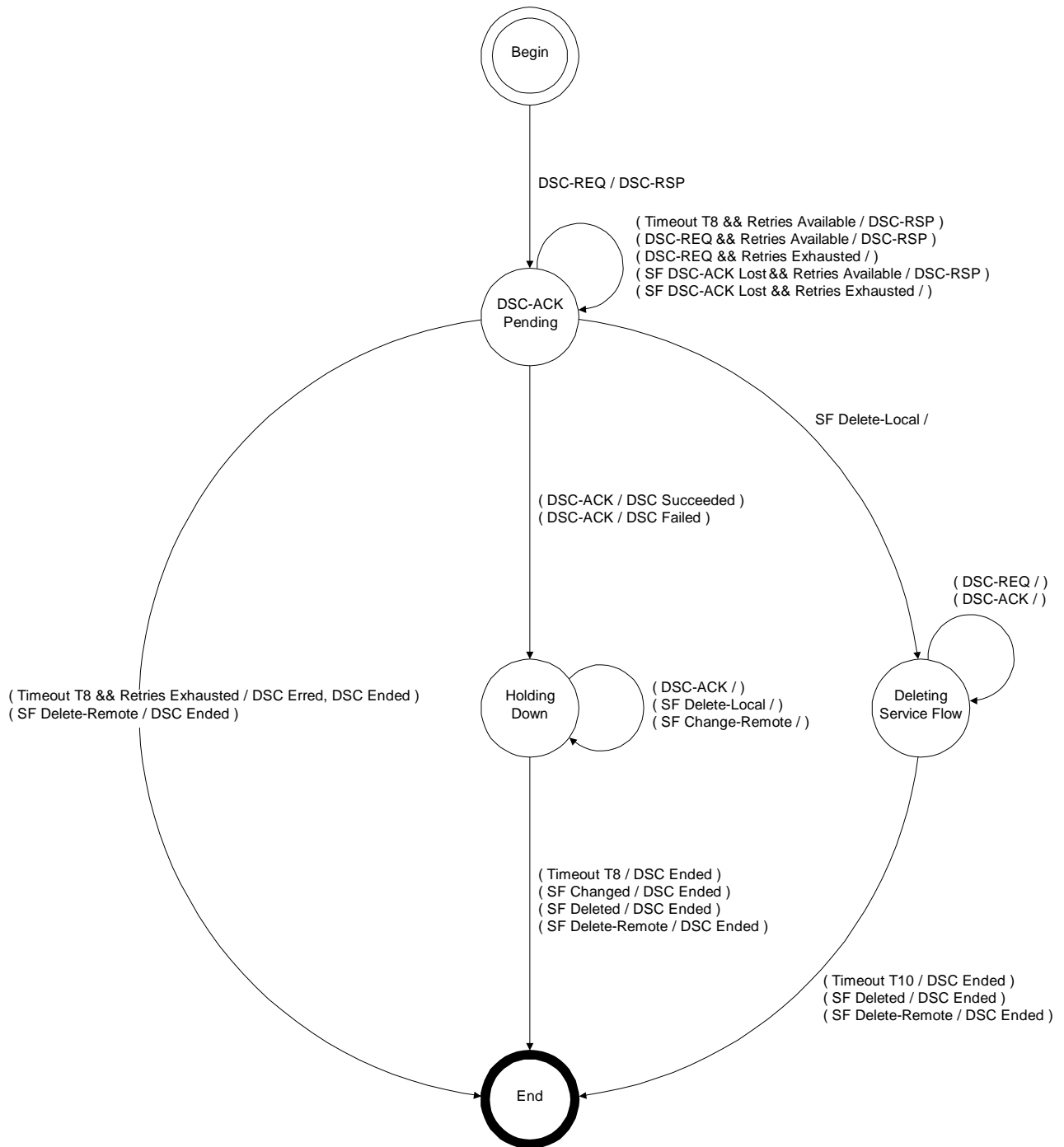
Figure 11–25: DSC - Remotely Initiated Transaction State Transition Diagram
