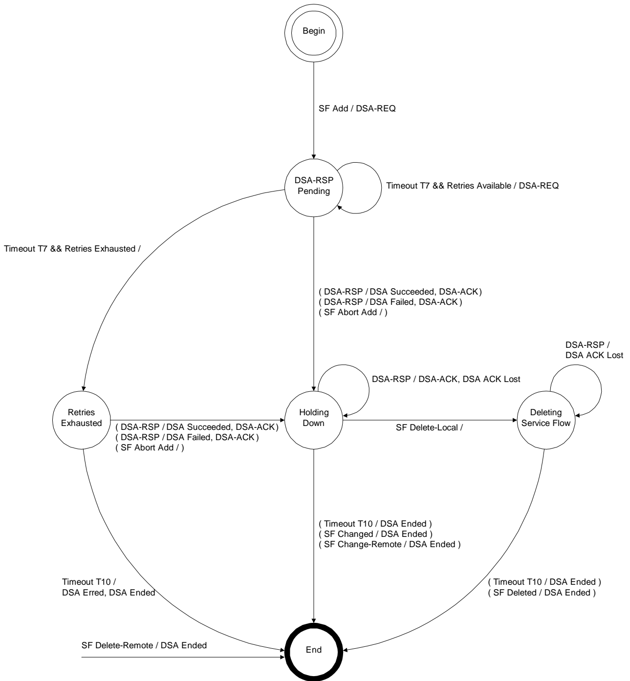
Figure 11–22: DSA - Locally Initiated Transaction State Transition Diagram
