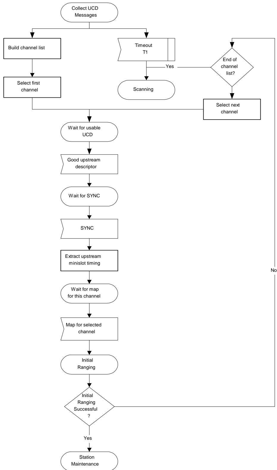
Figure 11–3: Obtaining Upstream Parameters
