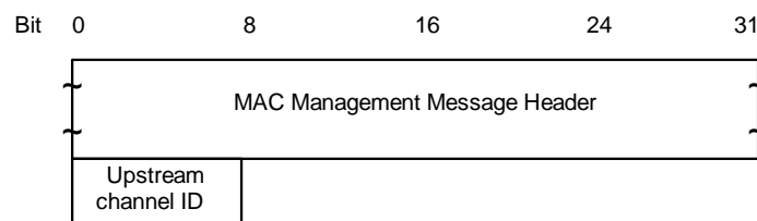
Figure 8-30: Upstream Channel Change Response
