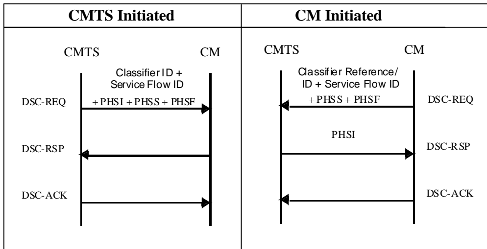
Figure 10–13: Payload Header Suppression Signaling Example
