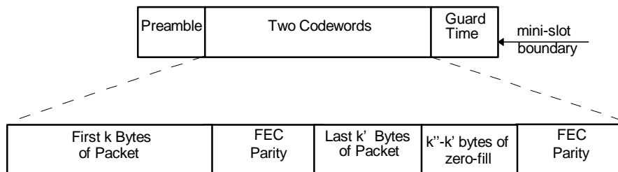
Figure 6-8: Example Frame Structures with Flexible Burst Length Mode
