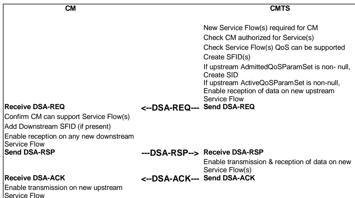
Figure 11–29: Dynamic Service Addition Initiated from CMTS
