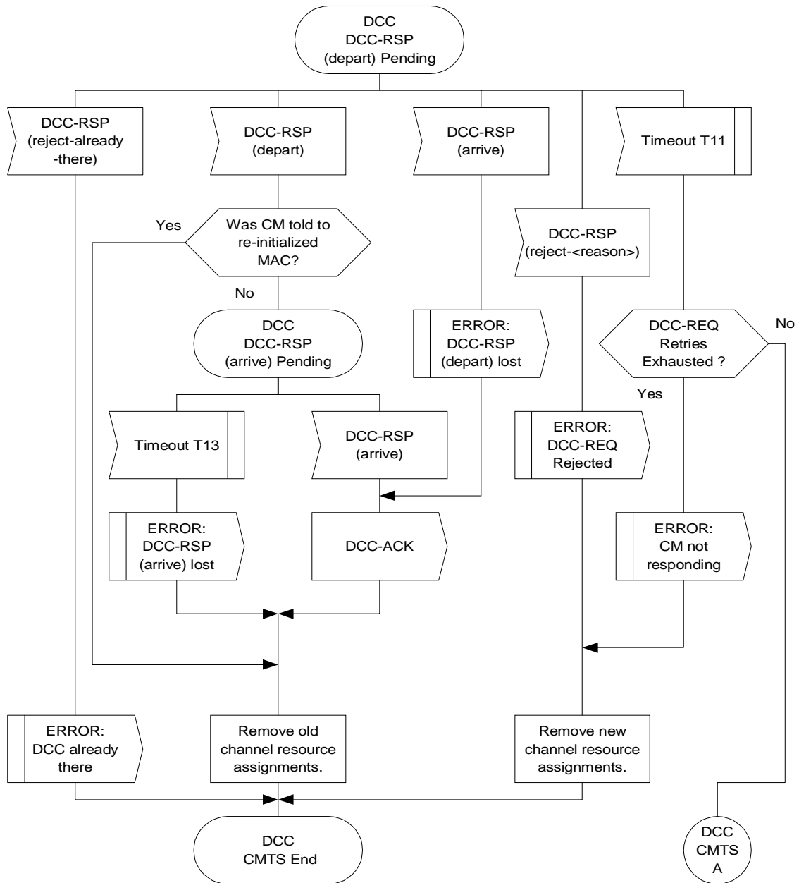
Figure 11-59: Dynamically Changing Channels: CMTS View Part 2
