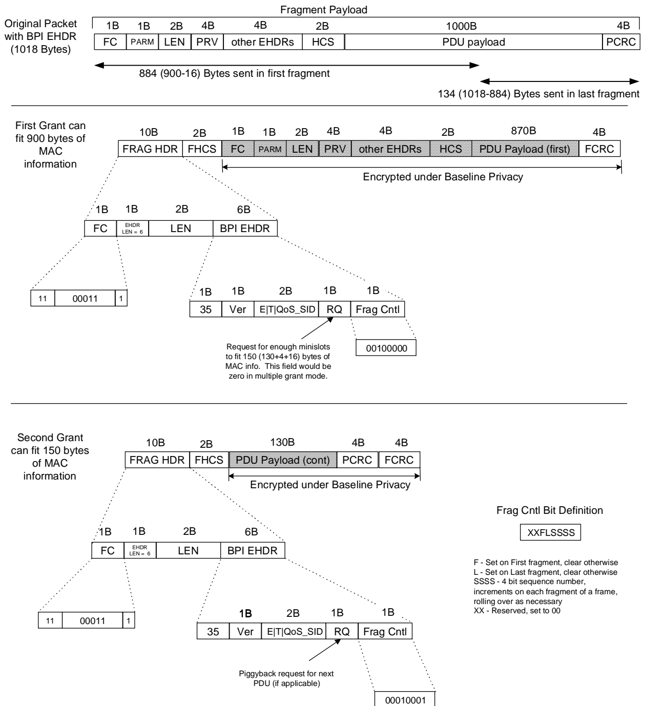
Figure 10-9: Example of Fragmenting a Single Packed
