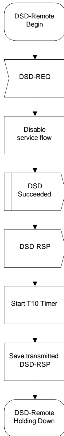
Figure 11–55: DSD - Remotely Initiated Transaction Begin State Flow Diagram
