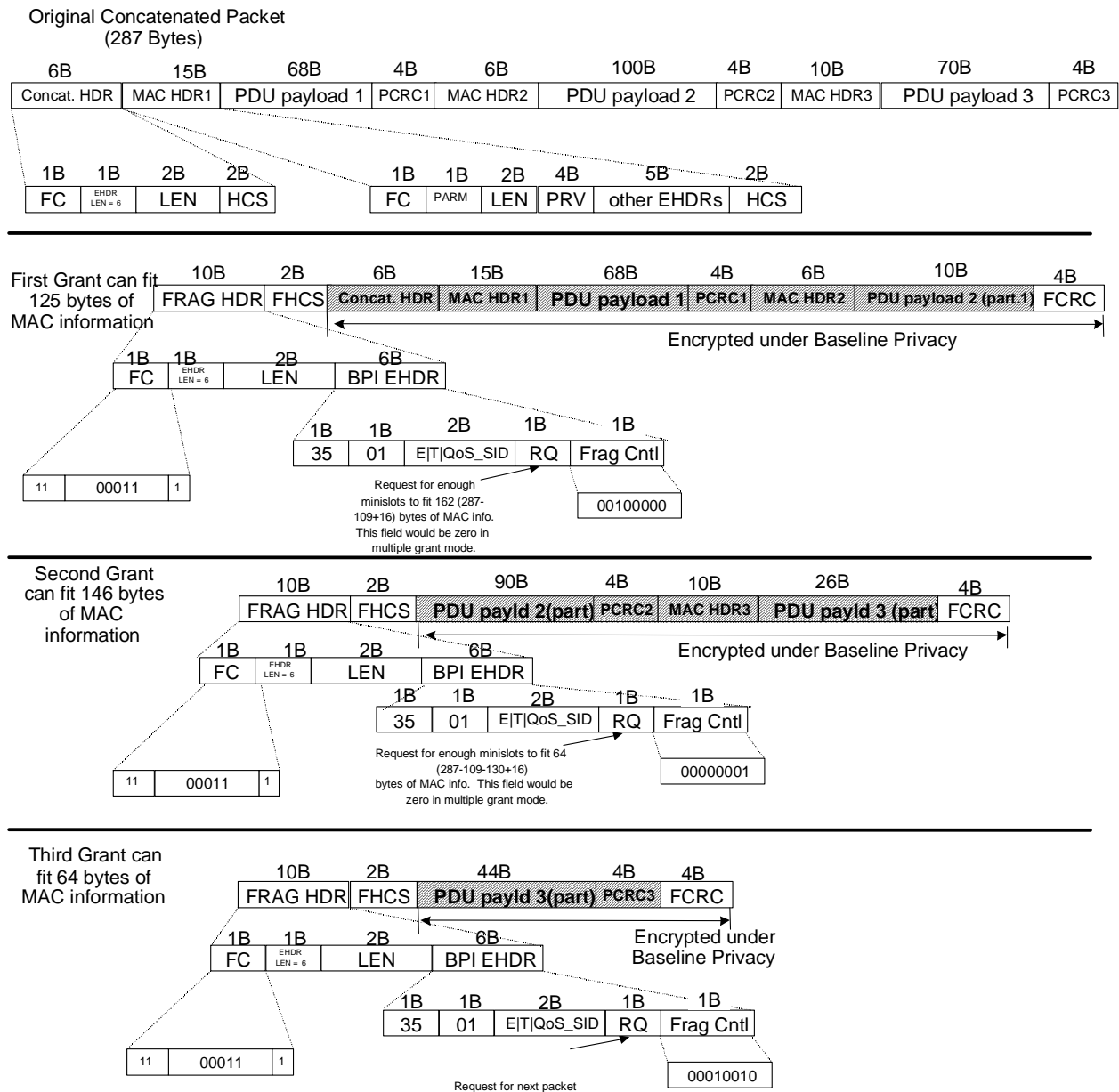
Figure 10–10: Fragmented Concatenated Packet Example
