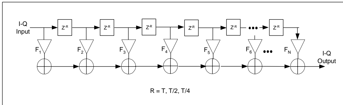
Figure N-5: Transmit Pre-Equalizer Structure
