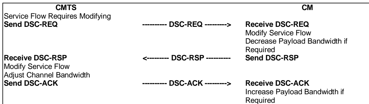
Figure 11–40: CMTS-Initiated DSC
