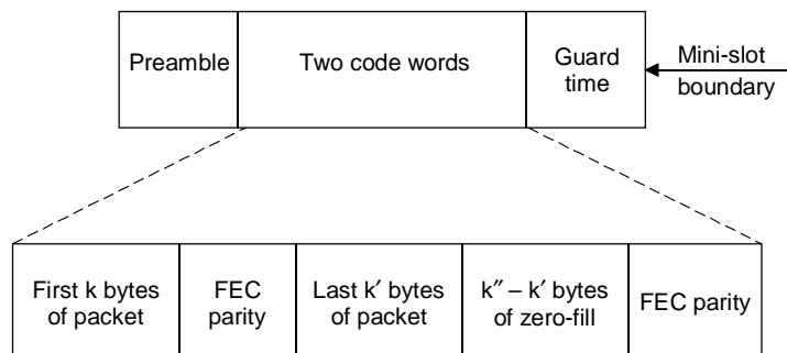
Example 2 – Packet length = k + remaining information bytes in 2^{\text{nd}} code word = k' \leq k + k'' \leq 2k bytes
