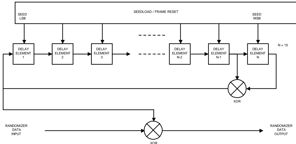
Figure 6-4: Scrambler Structure
