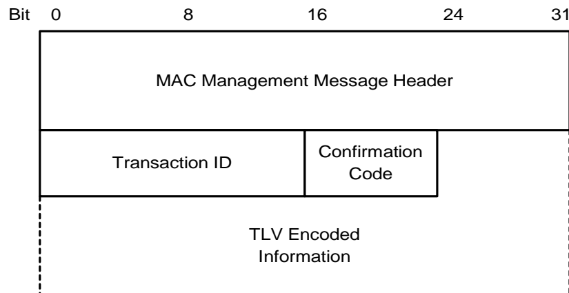
Figure 8-40: Dynamic Channel Change Acknowledge
