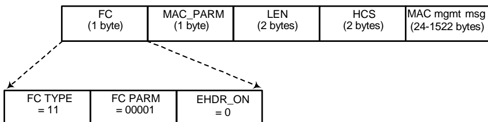
Figure 8-7: Management MAC Header
