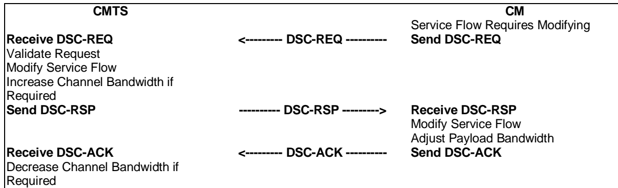
Figure 11–39: CM-Initiated DSC
