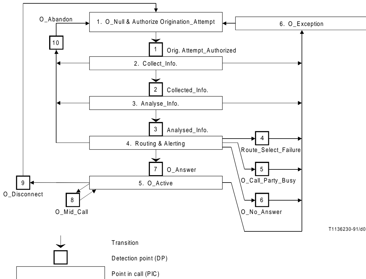
Figure B.1: Originating BCSM for CS-1 (figure 4-3 from ITU-T Recommendation Q.1214)
