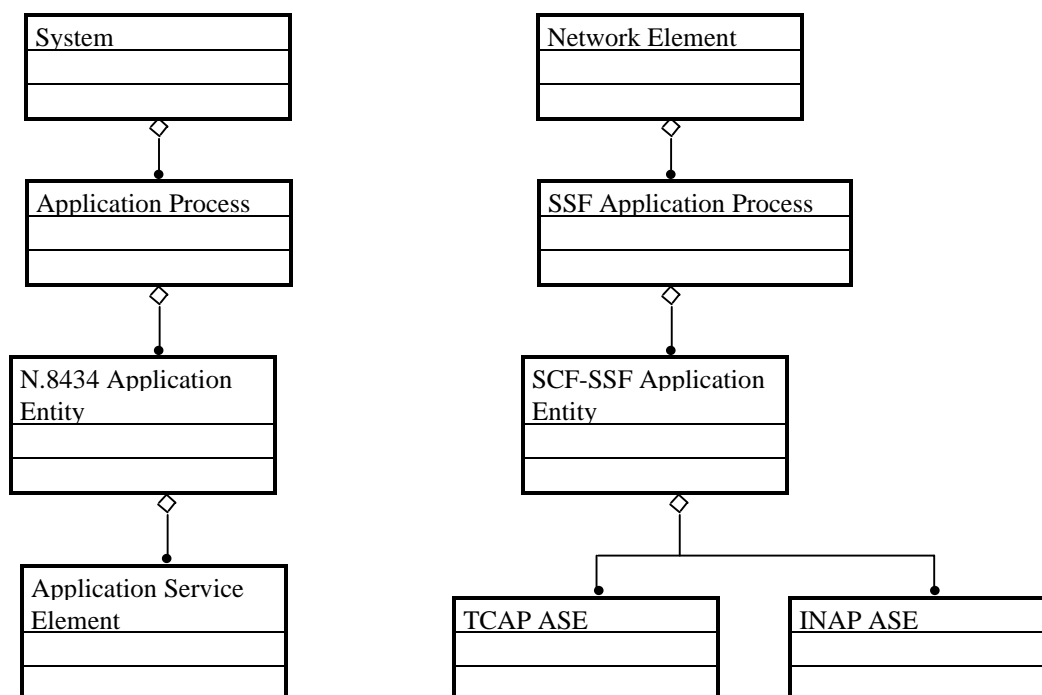
Figure 9.2.2: Comparison of managed objects for OSI upper layers with IN managed objects
