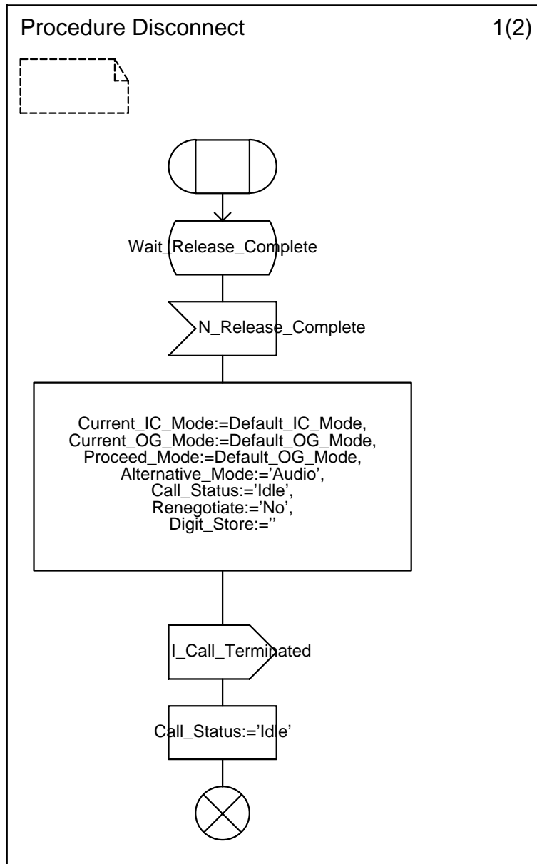
Figure 10: Disconnect procedure
