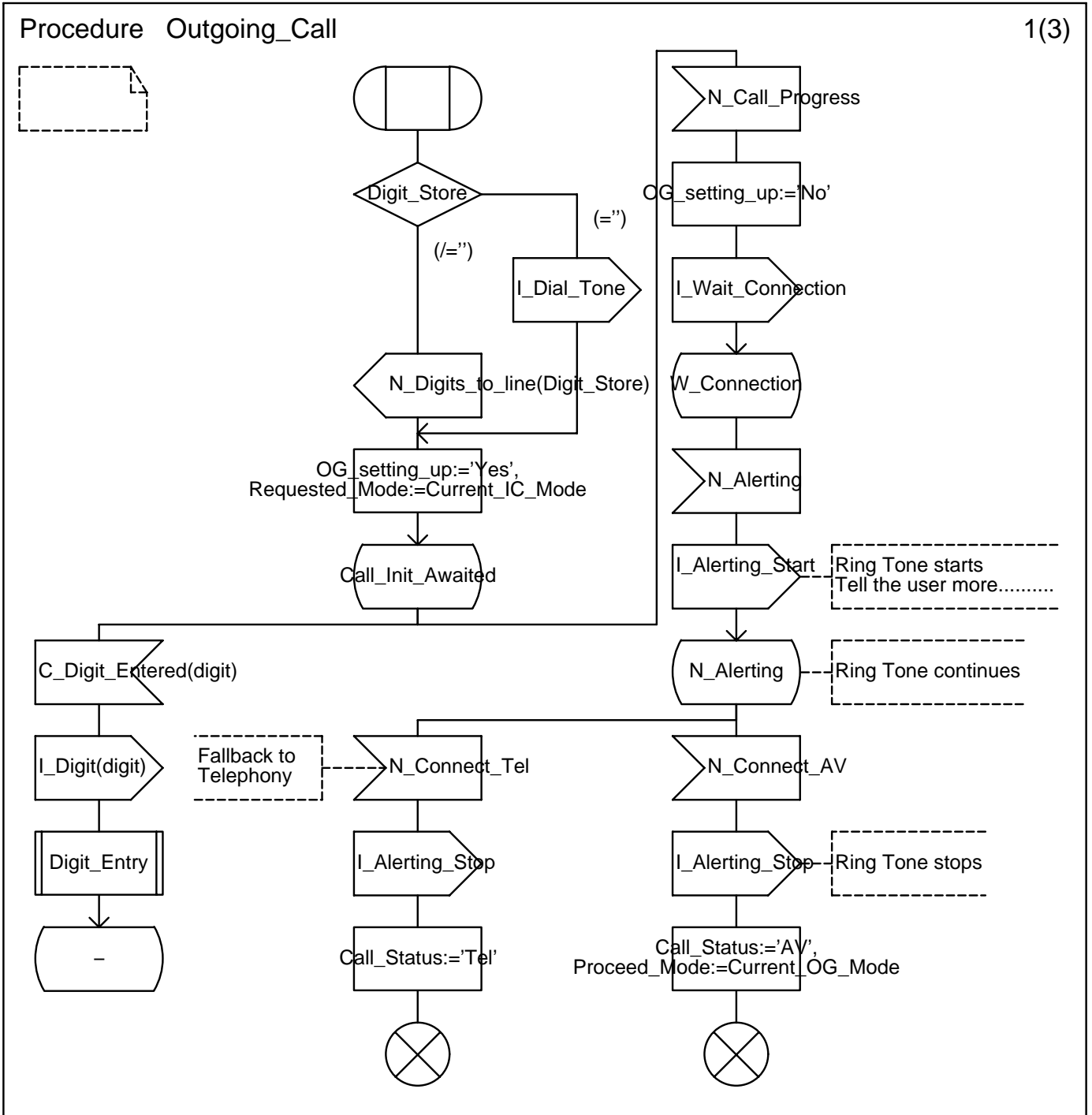
Figure 6: Outgoing_Call procedure
