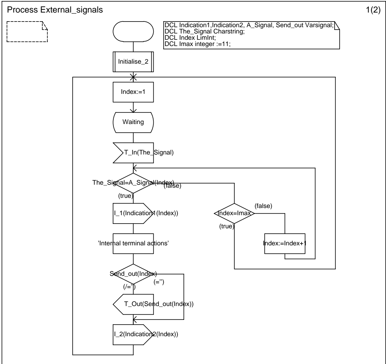
Figure 16: External Signals process
