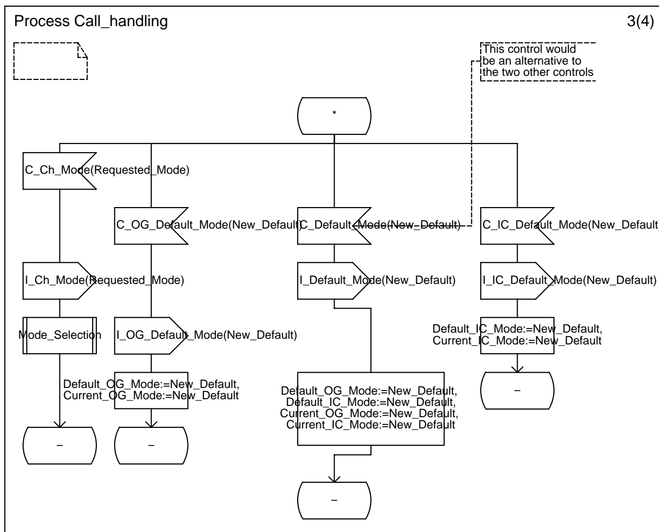
Figure 11: Mode change part of Call handling process
