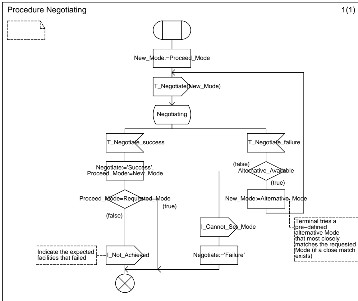
Figure 14: Negotiating procedure
