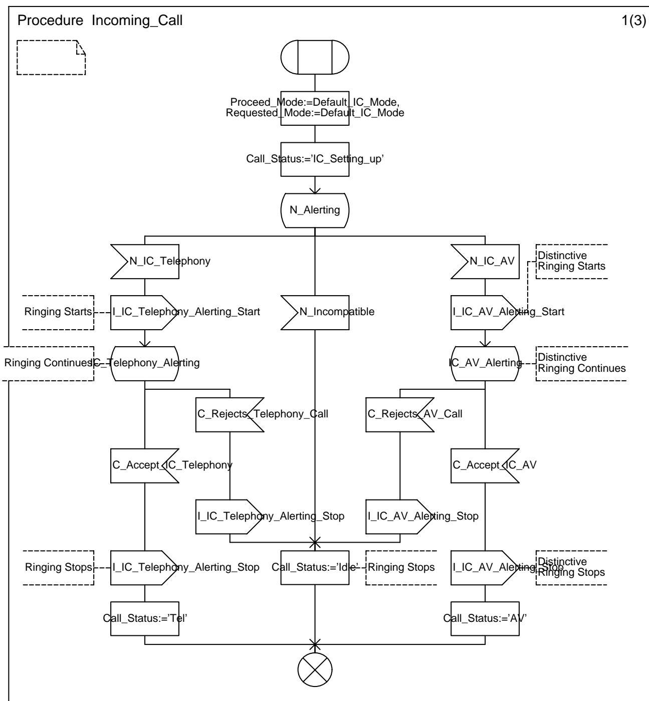
Figure 7: Incoming_Call procedure
