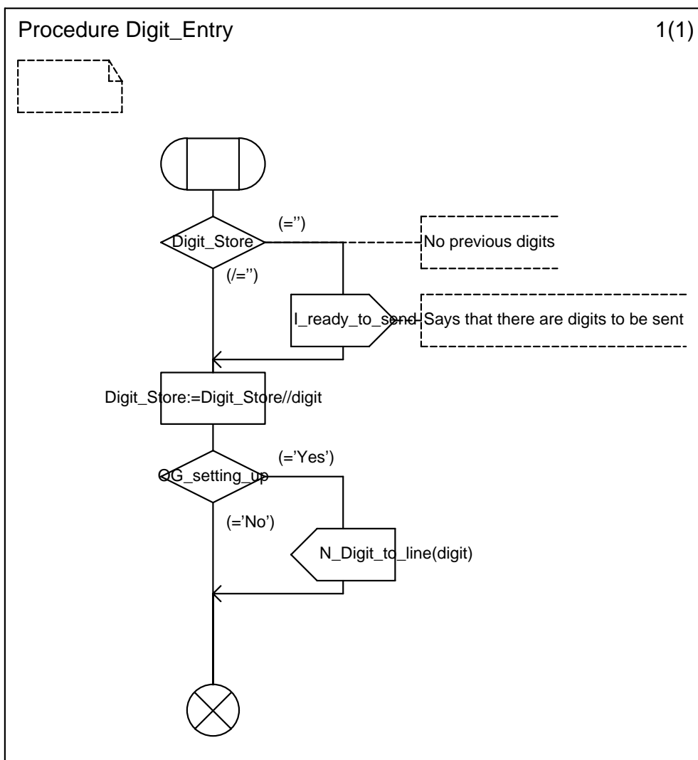
Figure 8: Digit_Entry procedure
