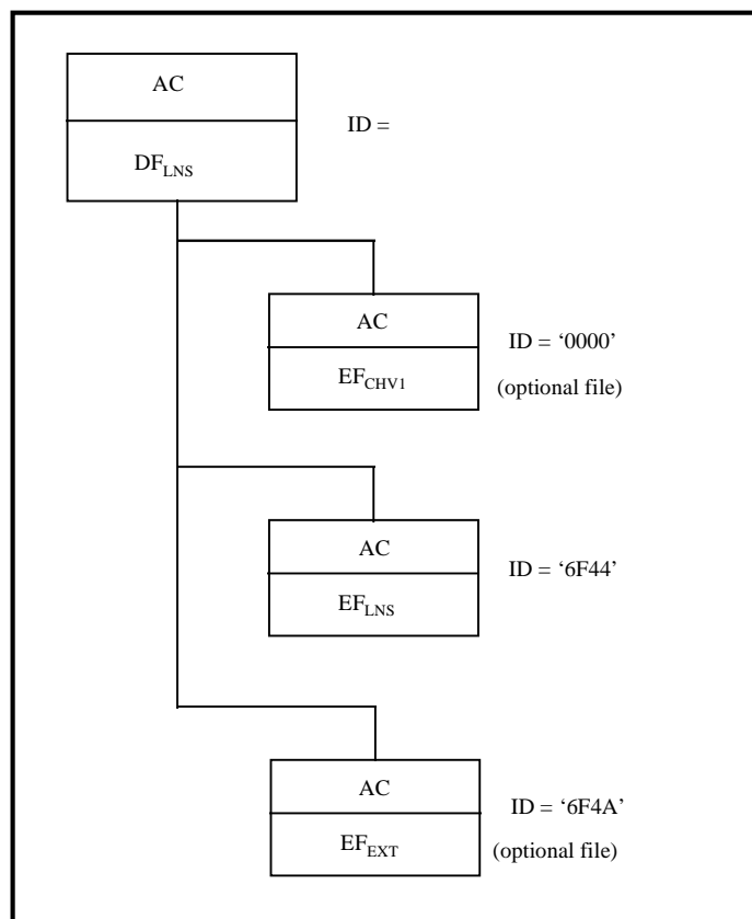
Figure 17: File structure for the Last Numbers Storage (LNS)
