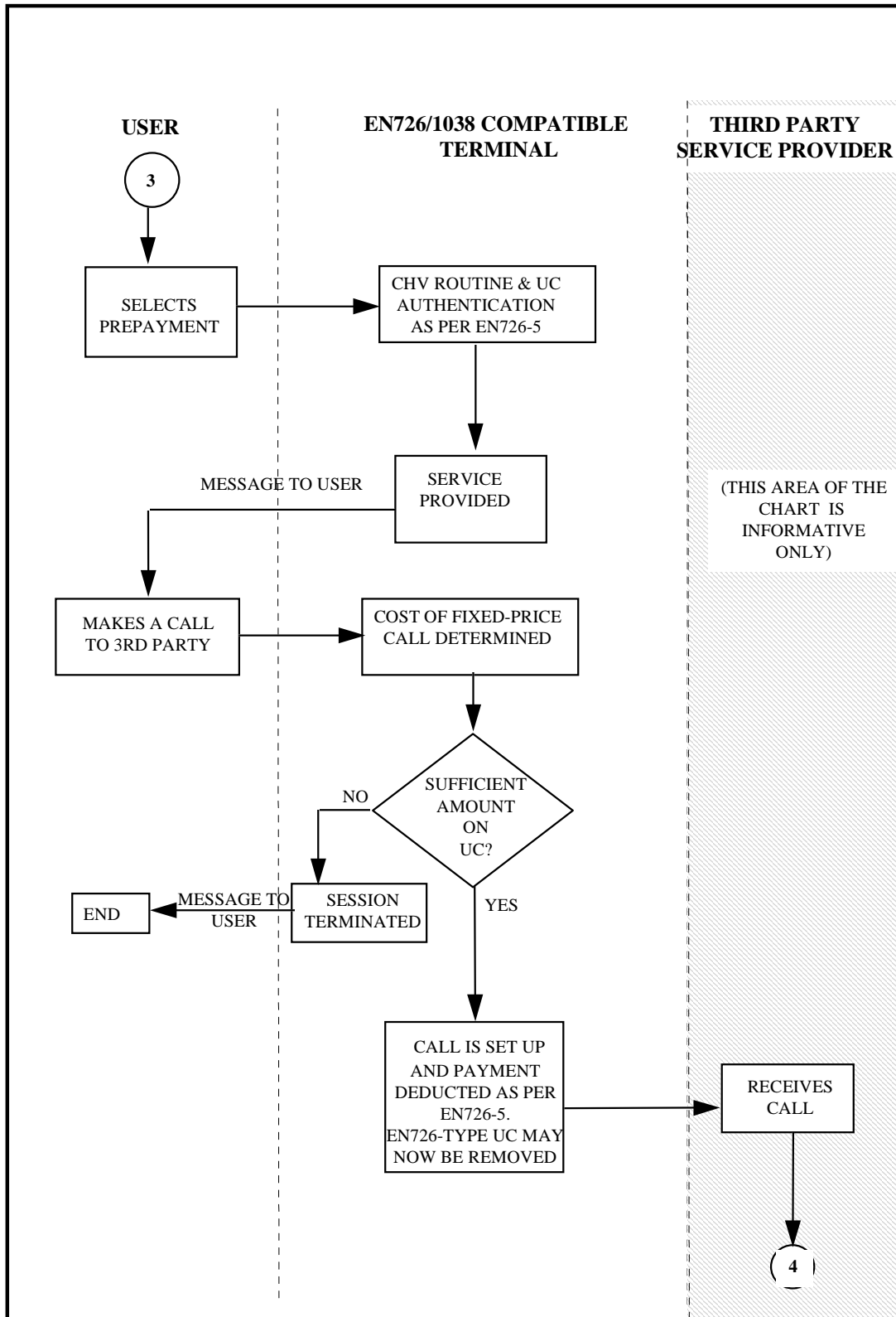
Figure 15: Scenario for the use of third party cards ATF with the EN 726-5 [4] prepayment application
