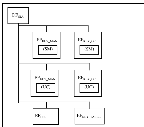
Figure 11: Data structure of application on Security Module (SM)
