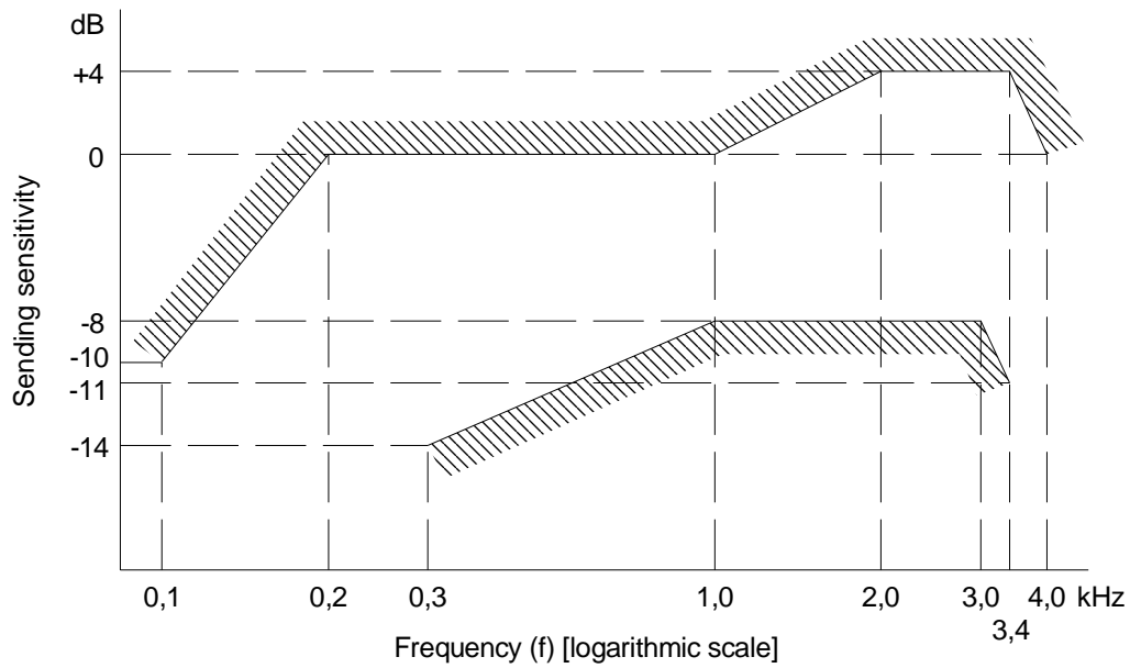
Figure 14: Send sensitivity/frequency mask
