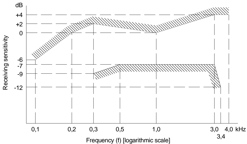
Figure 15: Receive sensitivity/frequency mask
