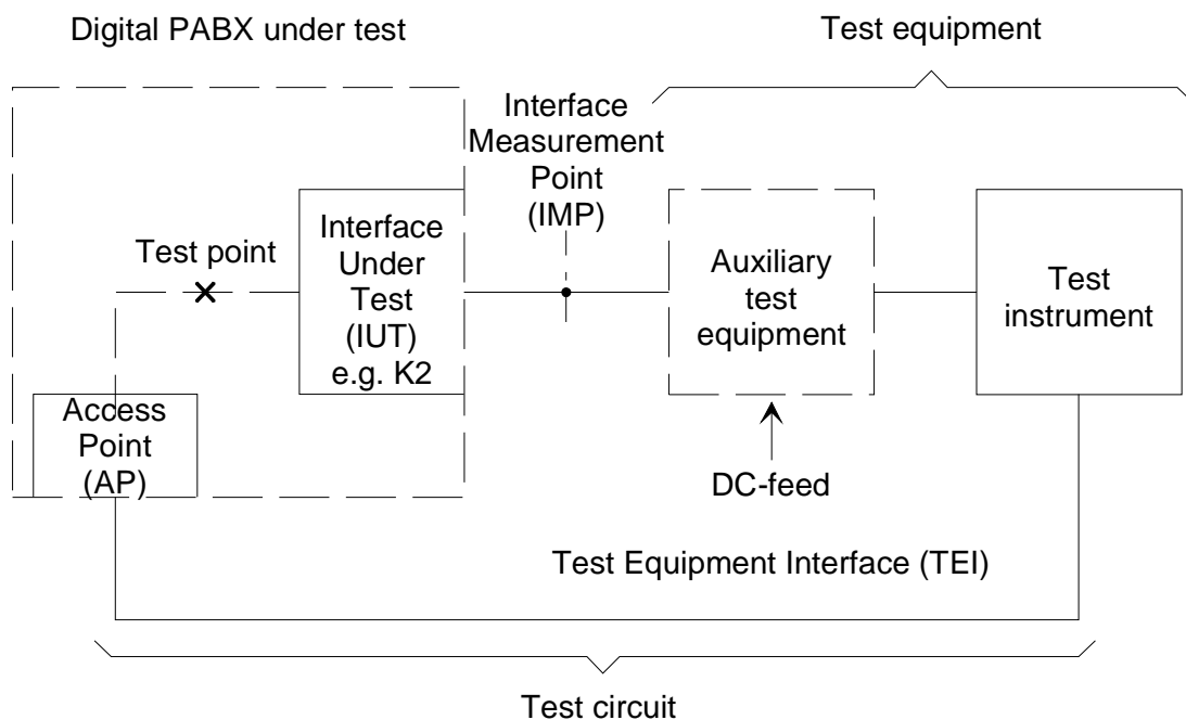
Figure A.1: Basic measurement configuration
