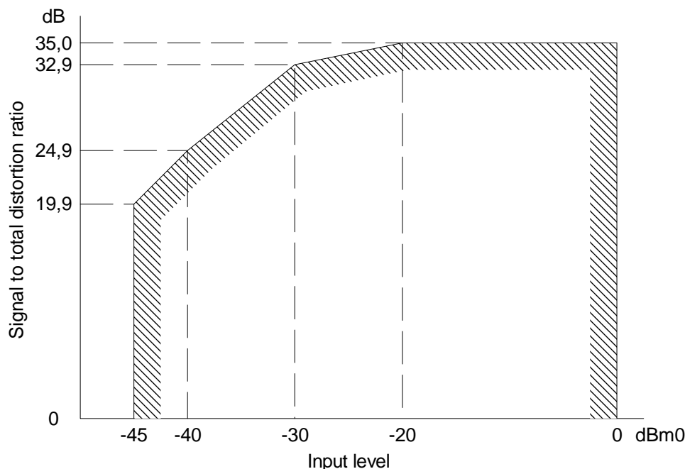
Figure 11: Limits for signal-to-total distortion ratio as a function of input level including analogue noise. Input connection ( L_i = 0 dBr). Interfaces L2 and M2 with feeding bridges
