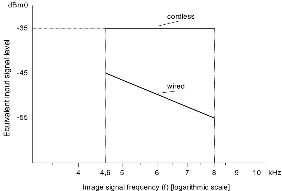
Figure 23: Discrimination levels (receiving)
