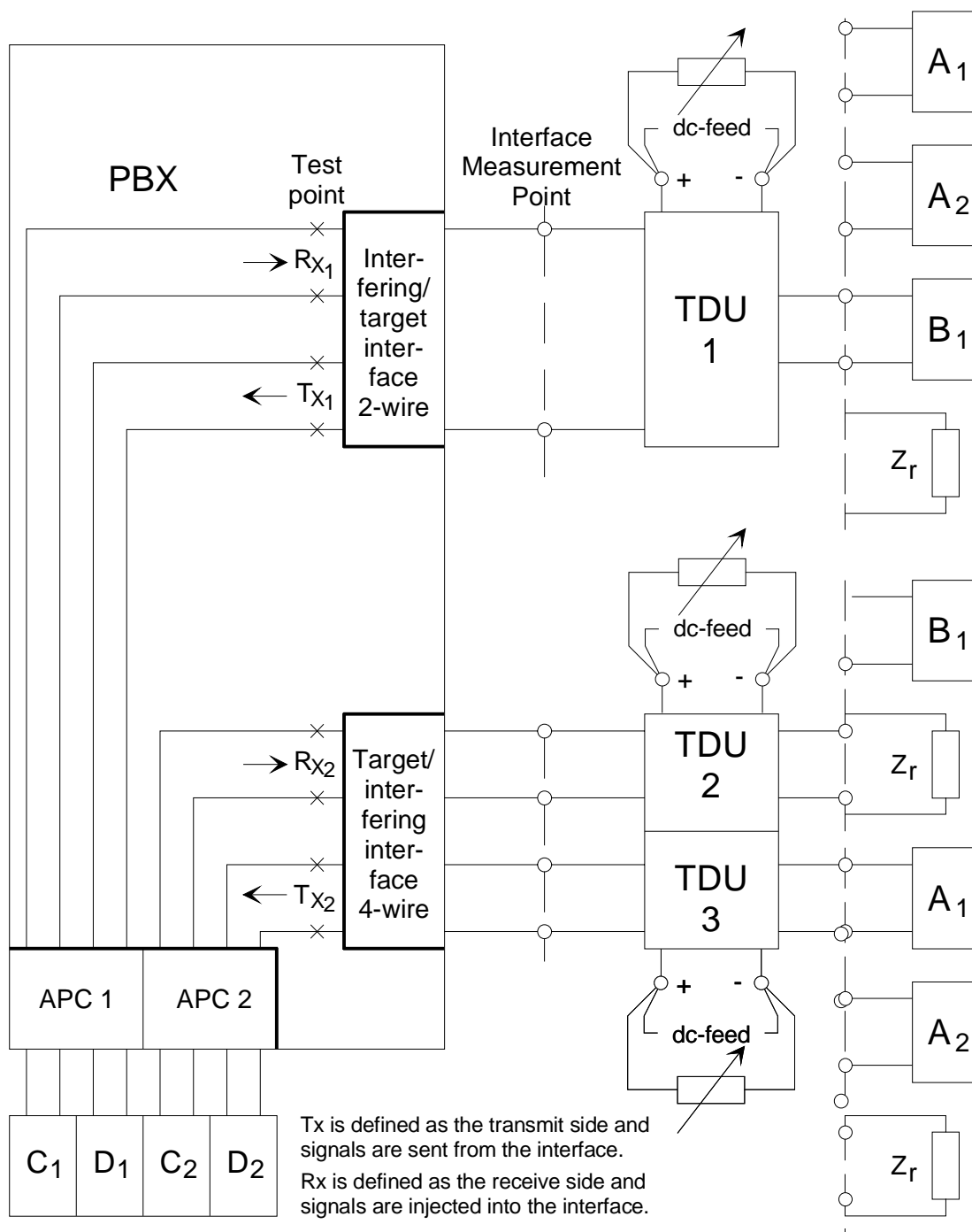
Figure A.15 (1 of 2): Crosstalk measurements between 4-wire and 2-wire analogue interfaces
