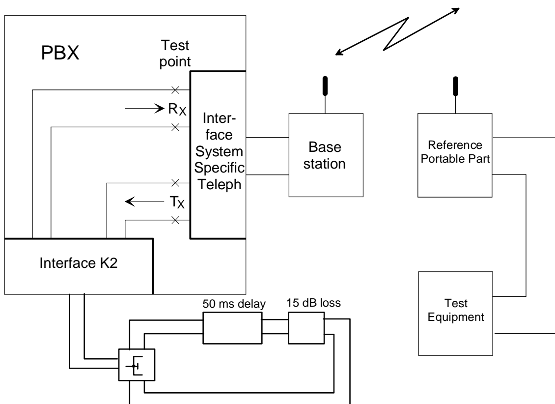
Figure A.24: Test configuration for measurement of Talker Echo Loudness Rating (case 3)
