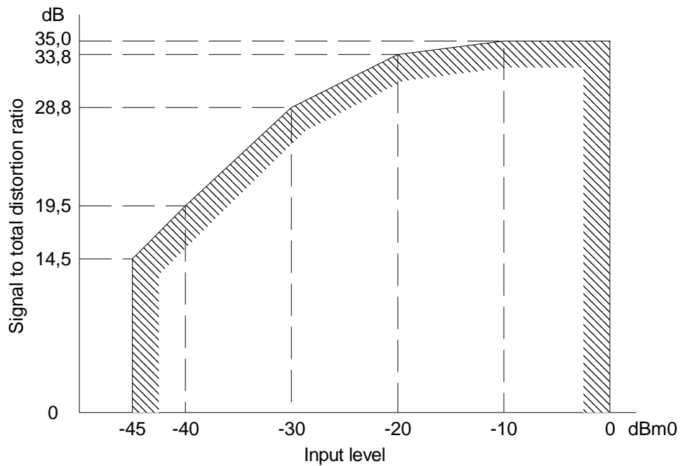
Figure 12: Limits for signal-to-total distortion ratio as a function of input level including analogue noise. Output connection ( L_o = -7 dBr). Interfaces L2 and M2 with feeding bridges
