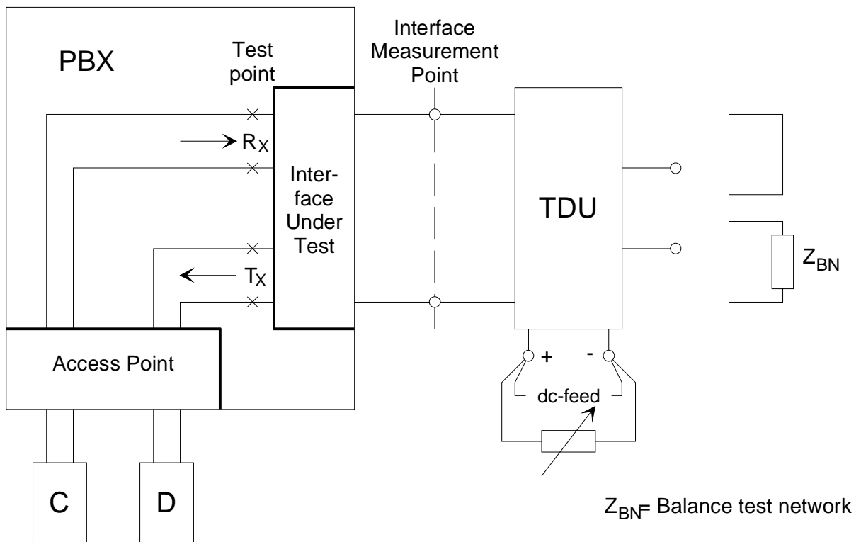
Figure A.12: Terminal Balance Return Loss, stability
