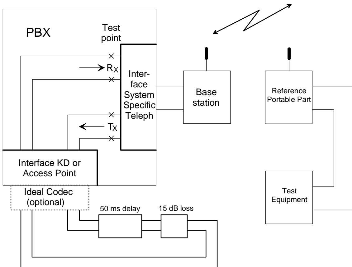
Figure A.23: Test configuration for measurement of Talker Echo Loudness Rating (case 3)
