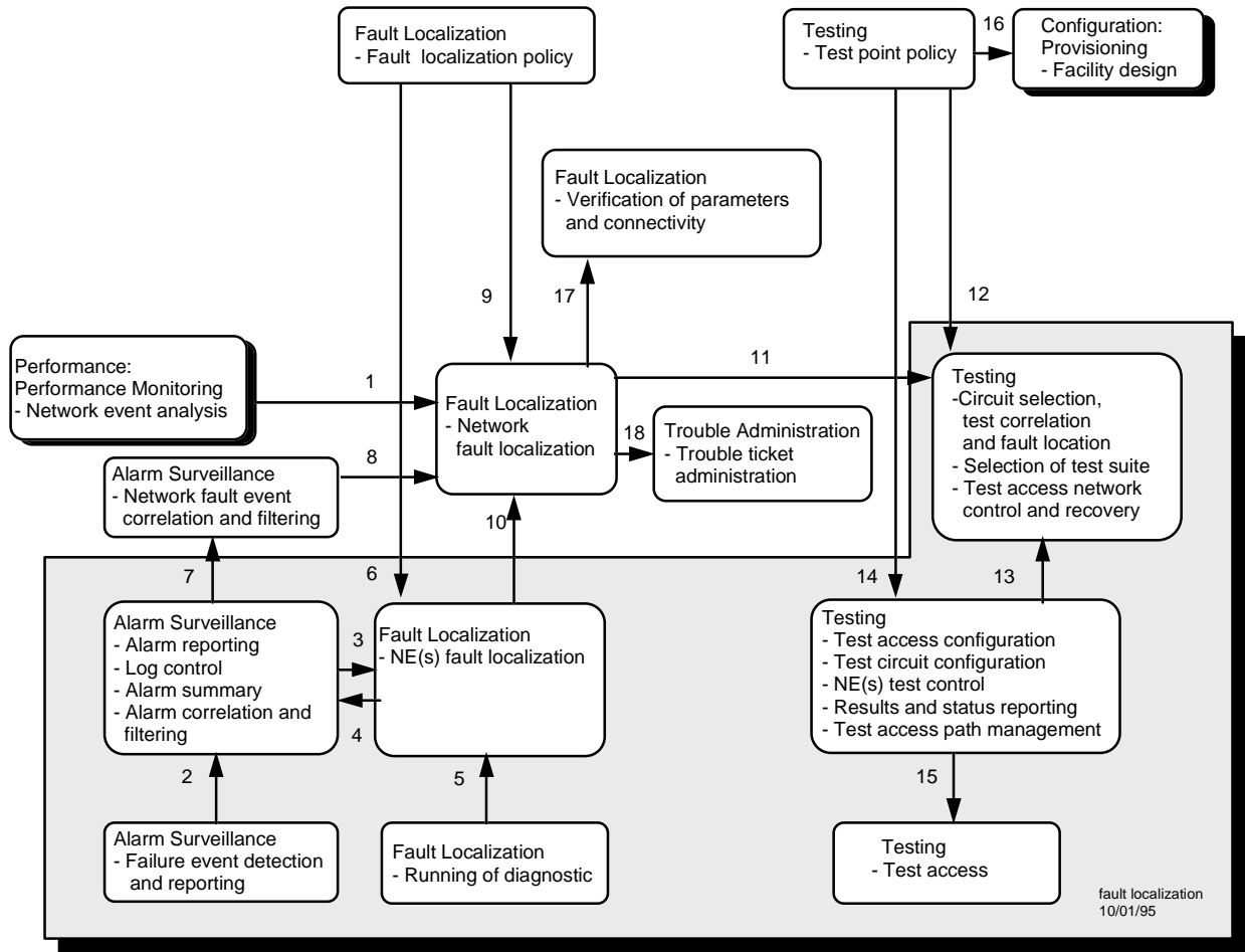
Figure 15: Fault localization (figure I-18/M.3400)
