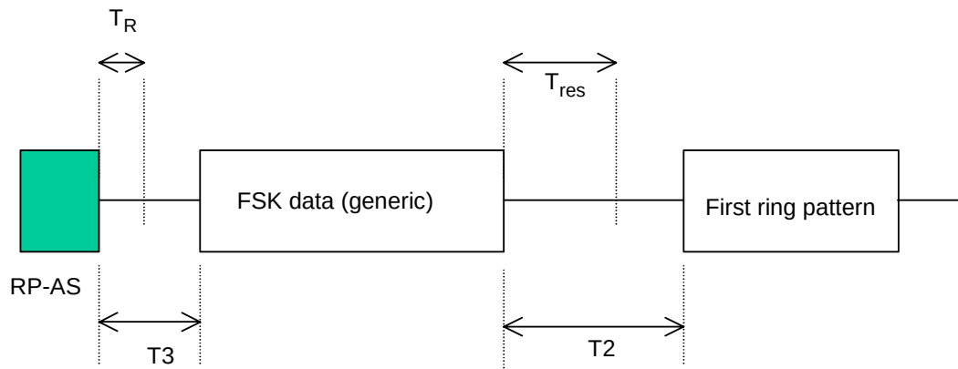
Figure 3: Data transmission prior to ringing - RP-AS
