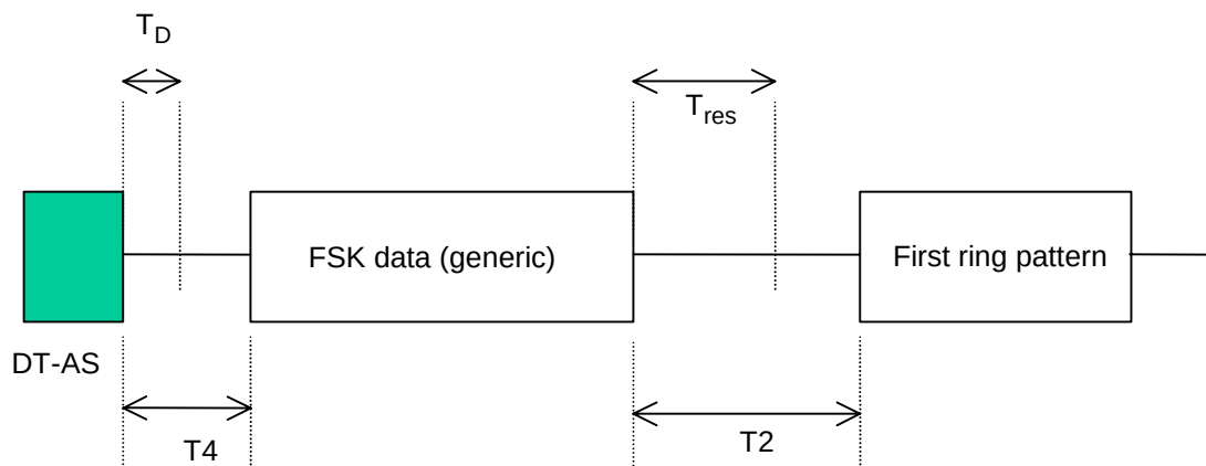
Figure 2: Data transmission prior to ringing - DT-AS
