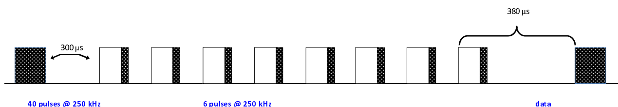
Figure 4: Wake-up trigger waveform
