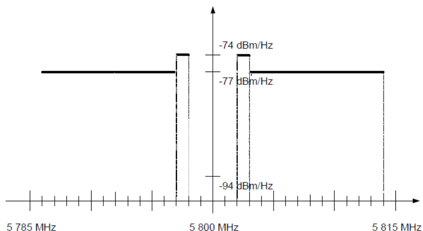
Figure 6: RSU transmitter spectrum mask - unwanted emissions
