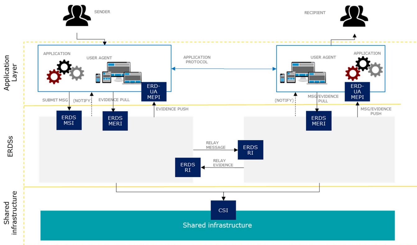
Figure 7: Interfaces
