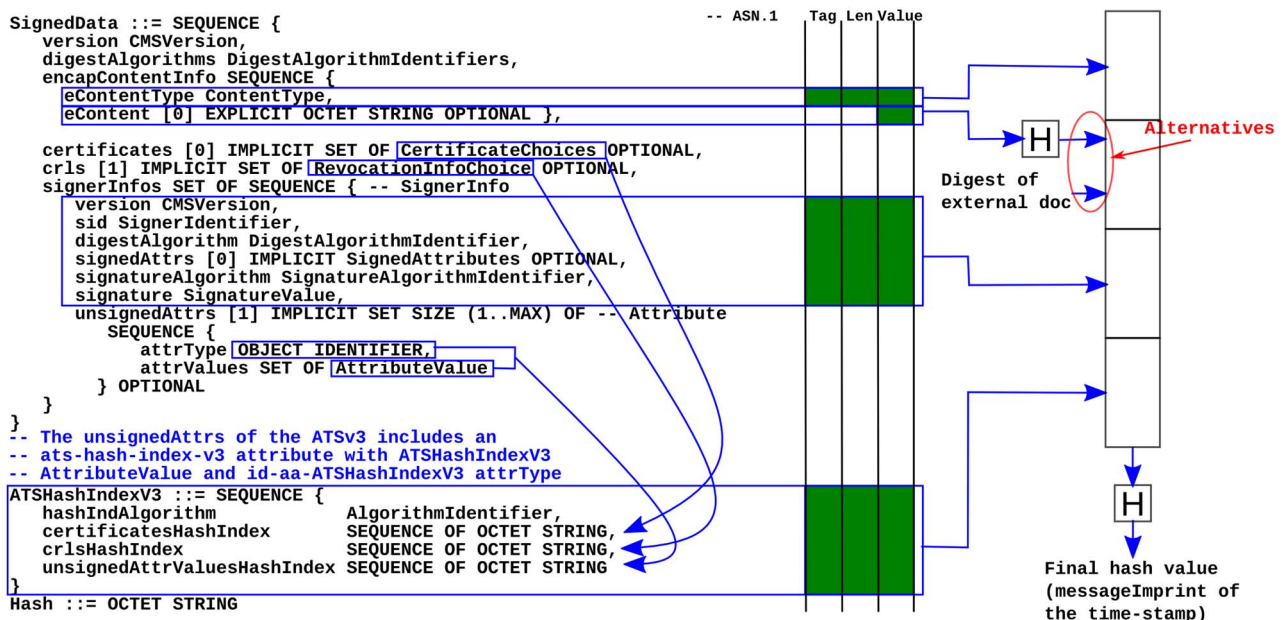
Figure 1: Hashing process
