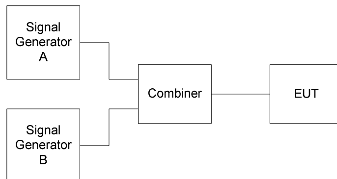
Figure 5.4.2.3-1: Measurement arrangement
