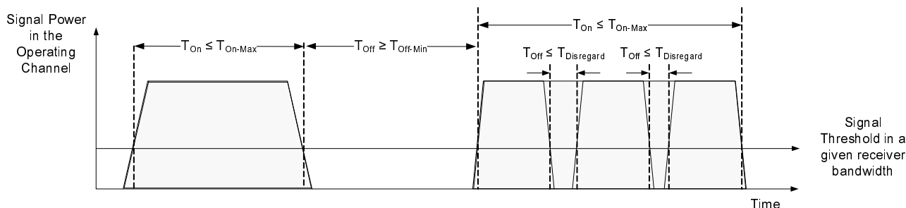
Figure 3.1-3: Transmission definitions
