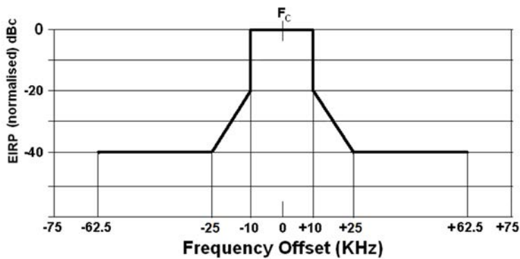
Figure 9: Transmitter spectrum mask
