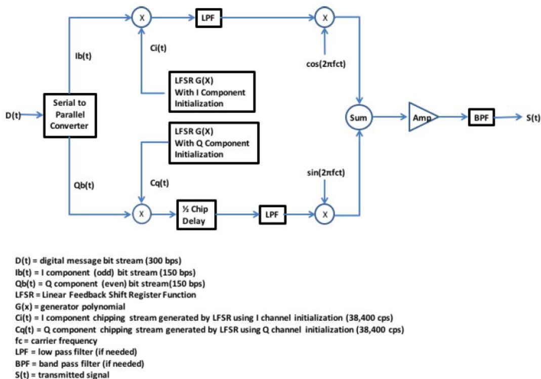
Figure 3: COSPAS-SARSAT modulation for SGBs
