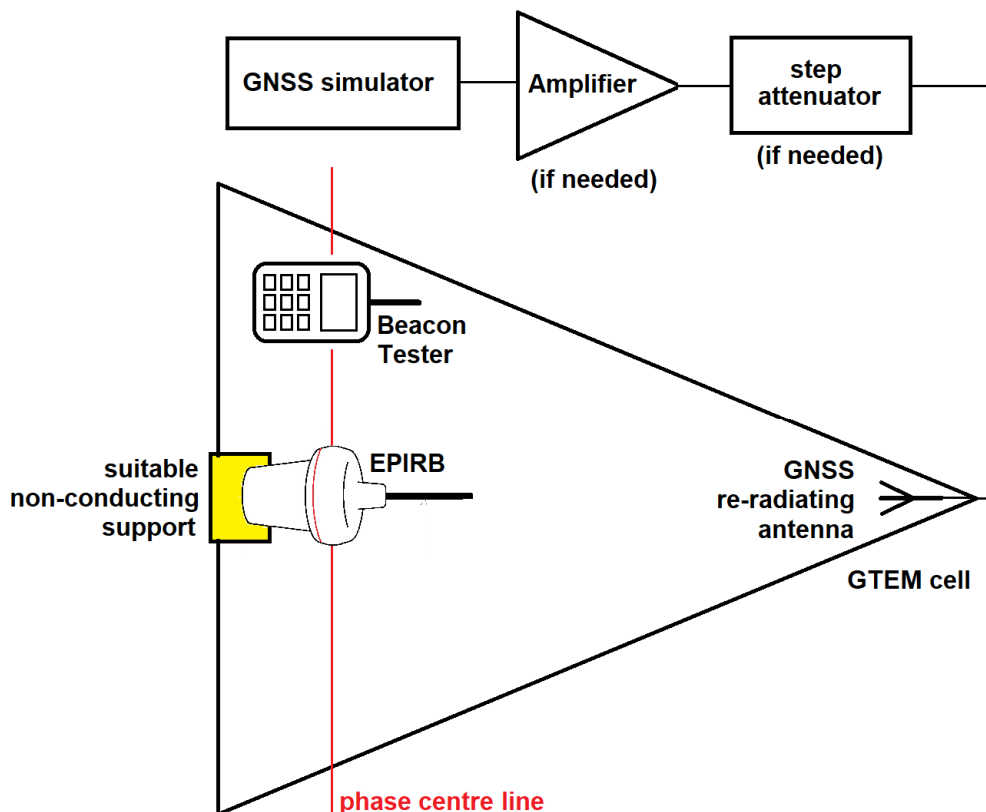
Figure 14: Test setup
