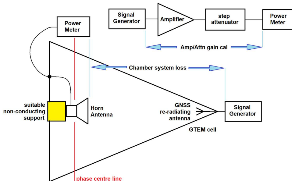
Figure 15: Calibration setup
