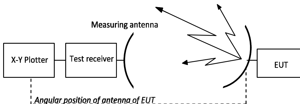
Figure 8: Test arrangement - antenna beam pointing
