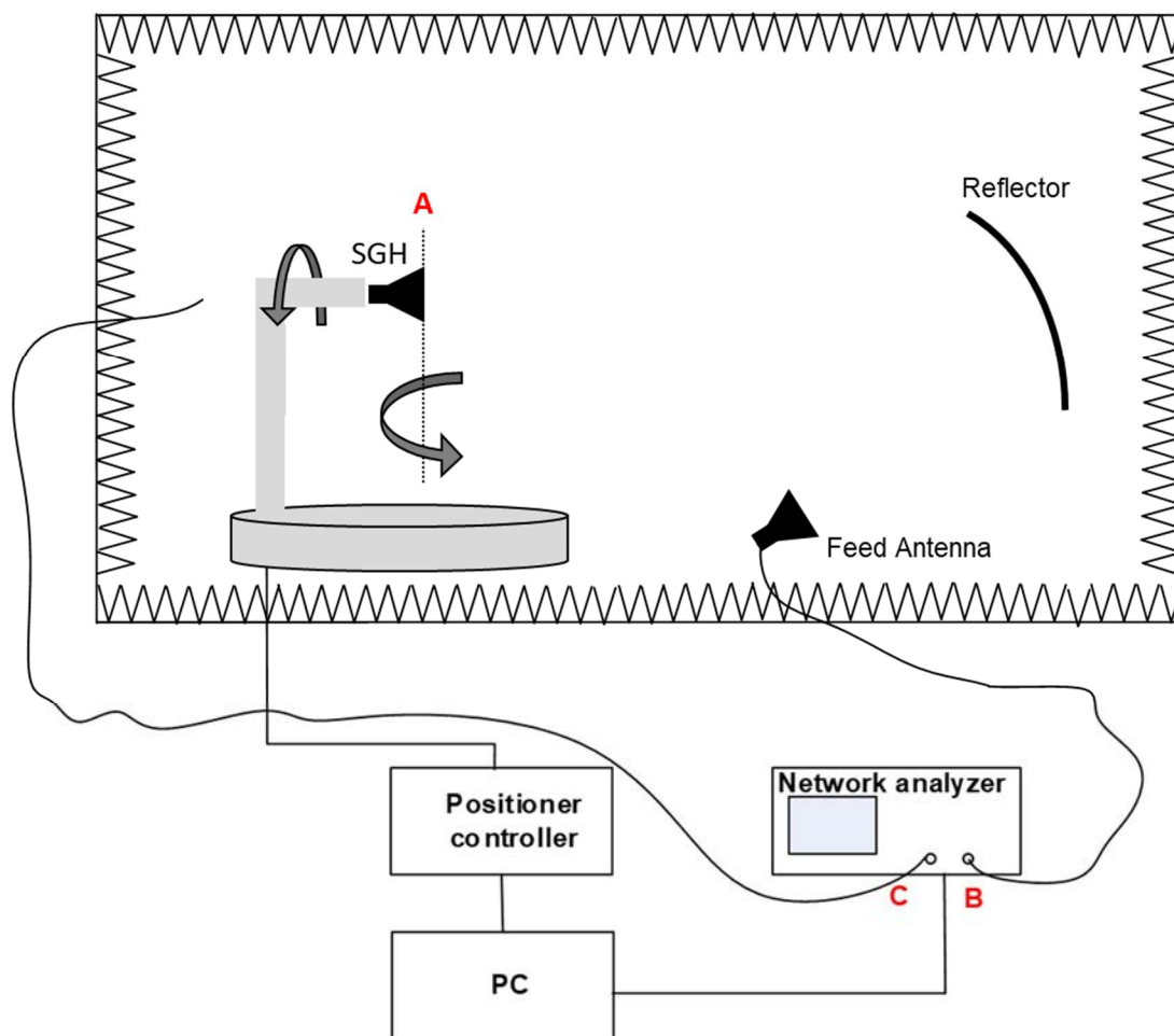
Figure B.6: CATR calibration system setup for EIRP
