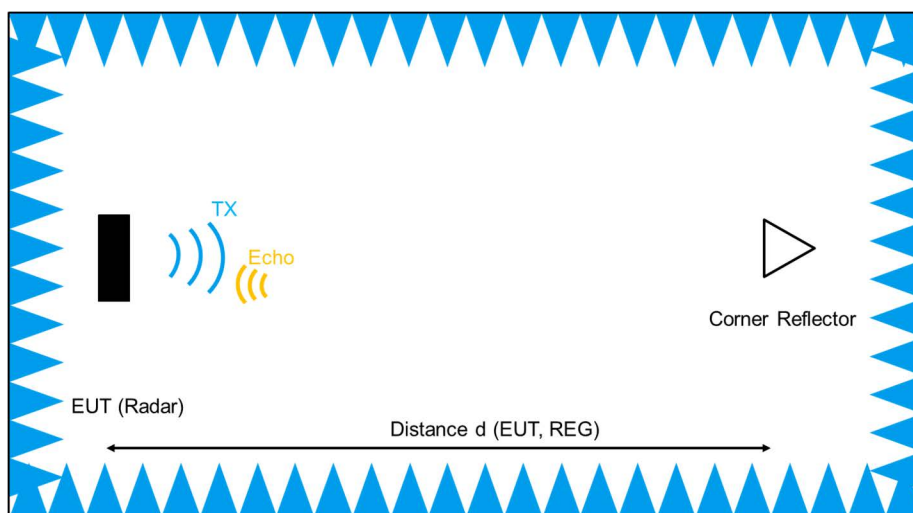
Figure D.2: Radar corner reflector inside an anechoic chamber
