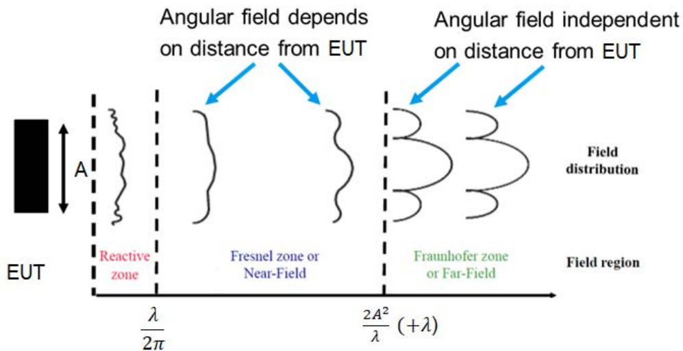
Figure D.3: Near-field and far-field considerations
