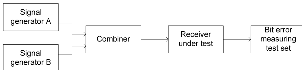
Figure 6: Measurement arrangement
