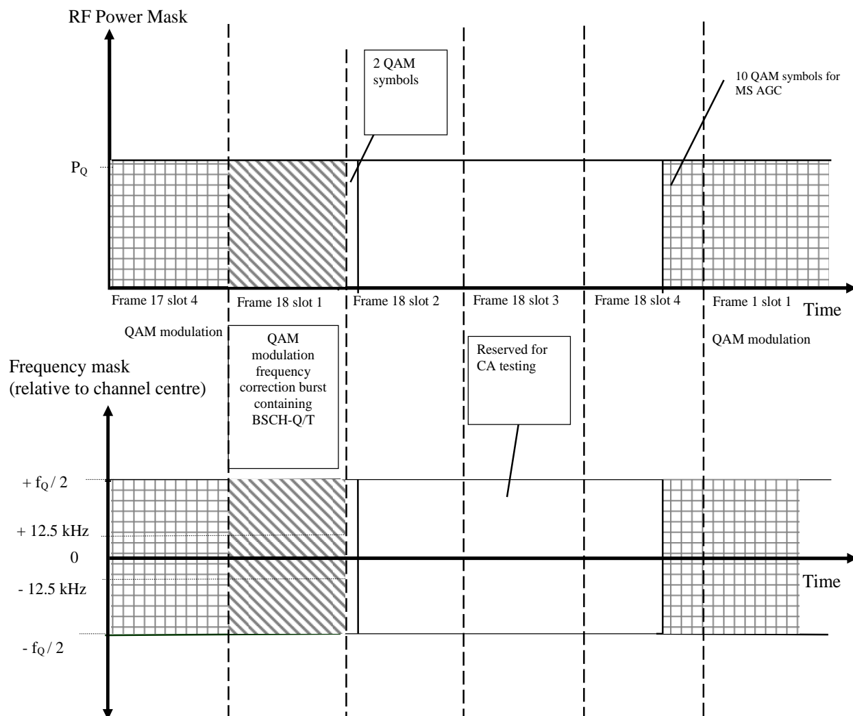
Figure 2: Variation of power, modulation type and frequency in a T4 signal for DA testing
