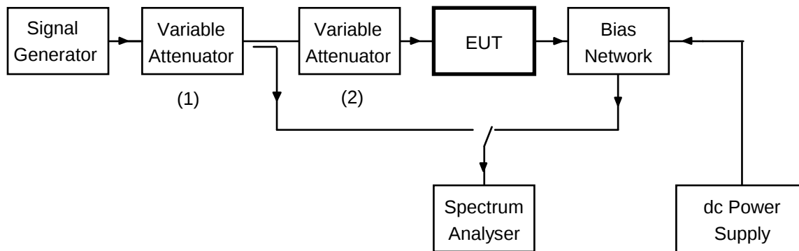
Figure 11: Test arrangement to measure image frequency rejection
