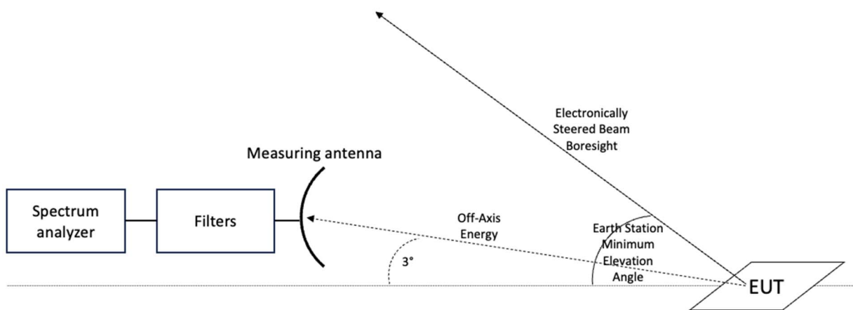
Figure 3: Test arrangement - spurious radiation measurements above 1 000 MHz for an EUT with electronically steered antenna
