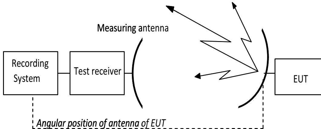
Figure 7: Test arrangement - antenna beam pointing
