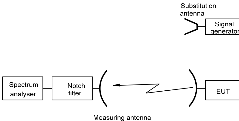
Figure 6: Test arrangement - on-axis spurious radiation measurements for an EUT with antenna
