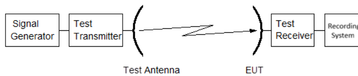
Figure 9: Test arrangement - EUT antenna receive pattern measurement
