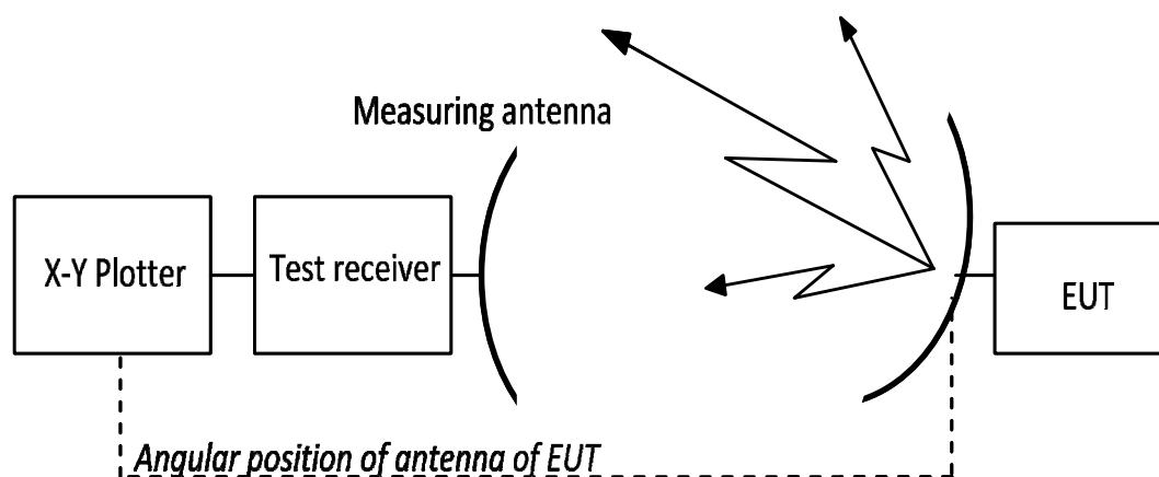
Figure 8: Test arrangement - antenna beam pointing
