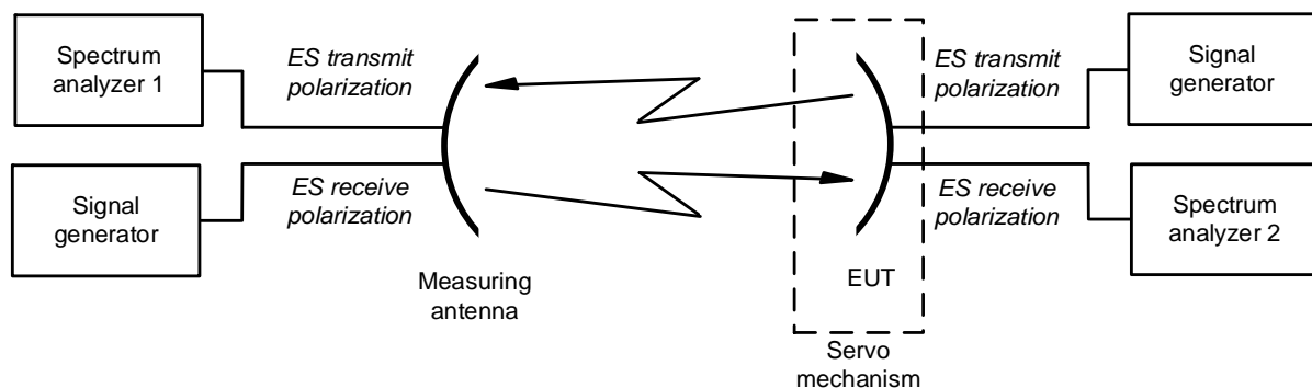
Figure 9: Test arrangement - polarization planes measurement
