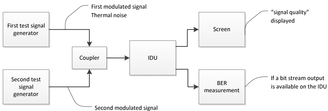
Figure 11: Test set-up for adjacent signal selectivity
