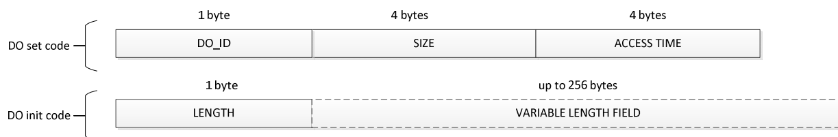
Figure 7.3: Format of a particular DO_Configcode
