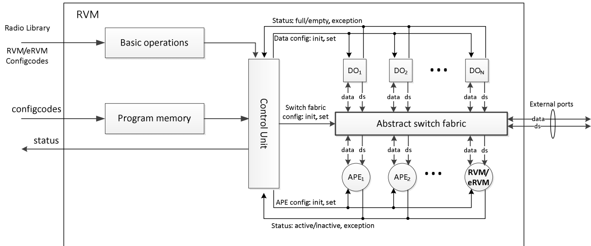
Figure 6.6: RVM hierarchy
