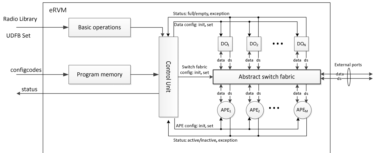
Figure 6.2: Elementary RVM
