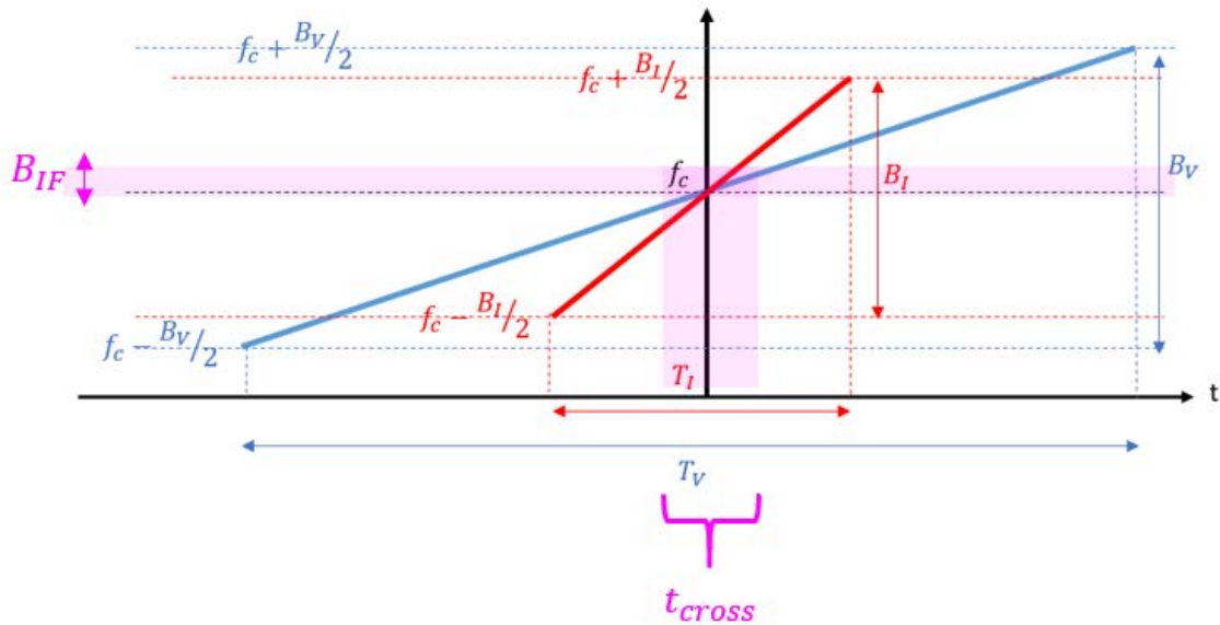
Figure E.2: Crossing time t_{\text{cross}} between interfering signals
