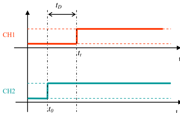
Figure 9: Minimum listen time, t_D , measurement
