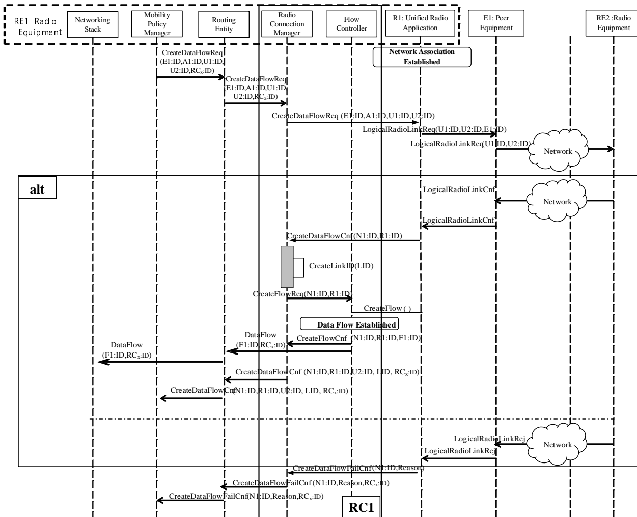
Figure 6.5-2: Creation of a logical radio link association initiated by Radio Equipment 1 (RE1)
