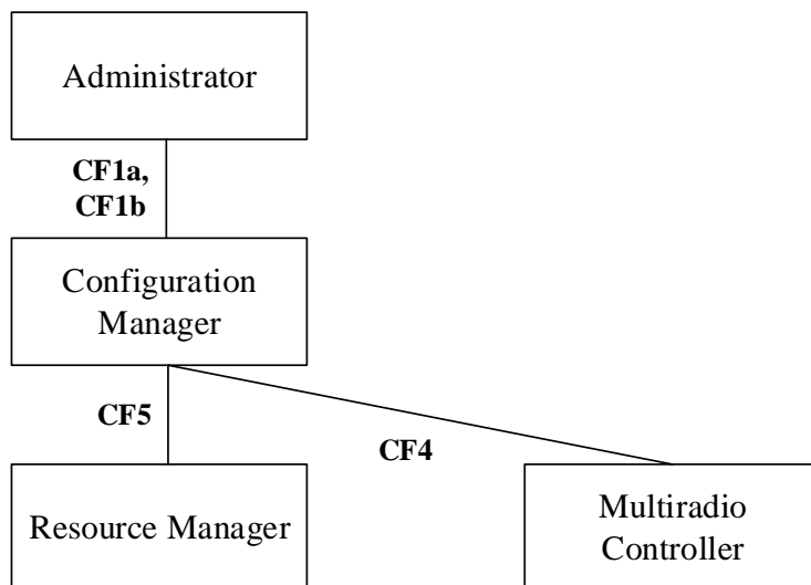
Figure 5.2-1: Illustration of reference points for installation/uninstallation and creating/deleting instance of a URA
