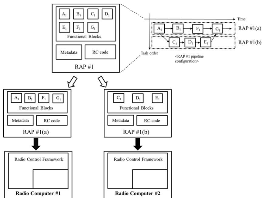
Figure A.1: Conceptual diagram of RA distributed installation on multiple radio computers
