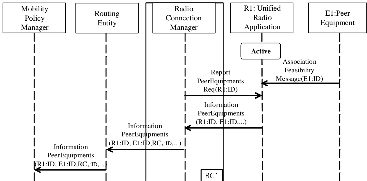
Figure 6.7-1: Report of discovered peer equipment
