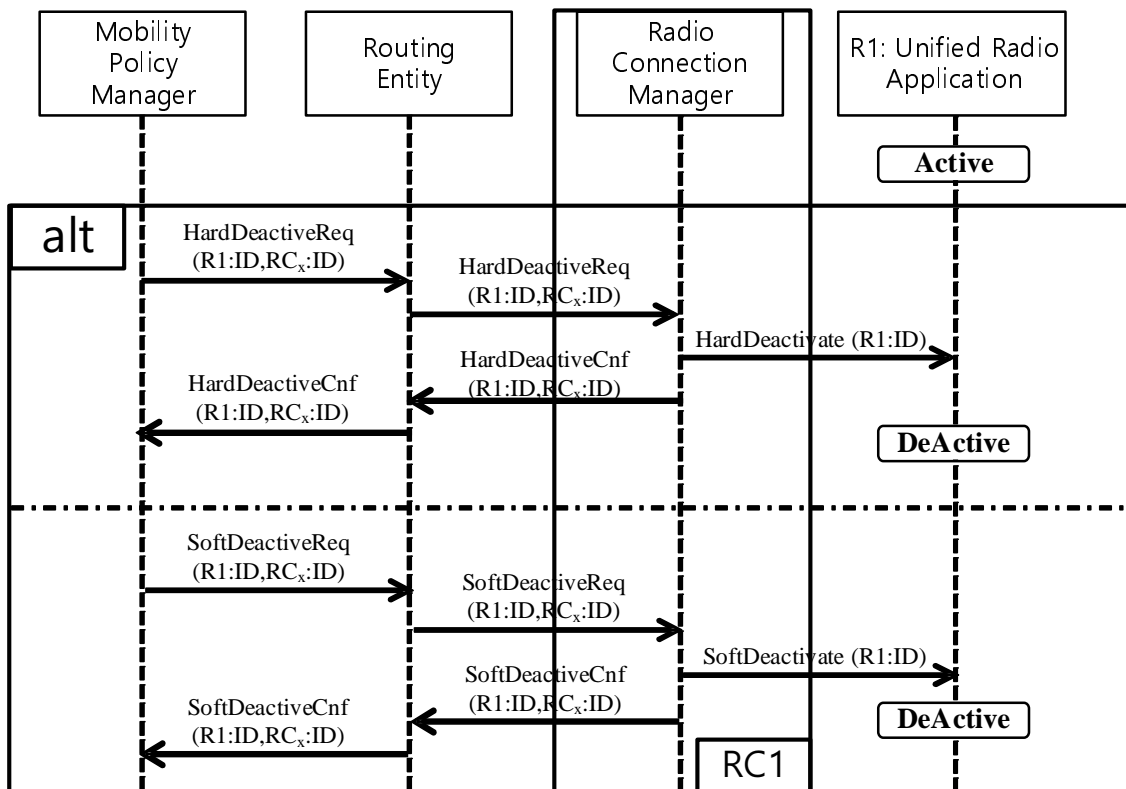
Figure 6.3-2: URA deactivation
