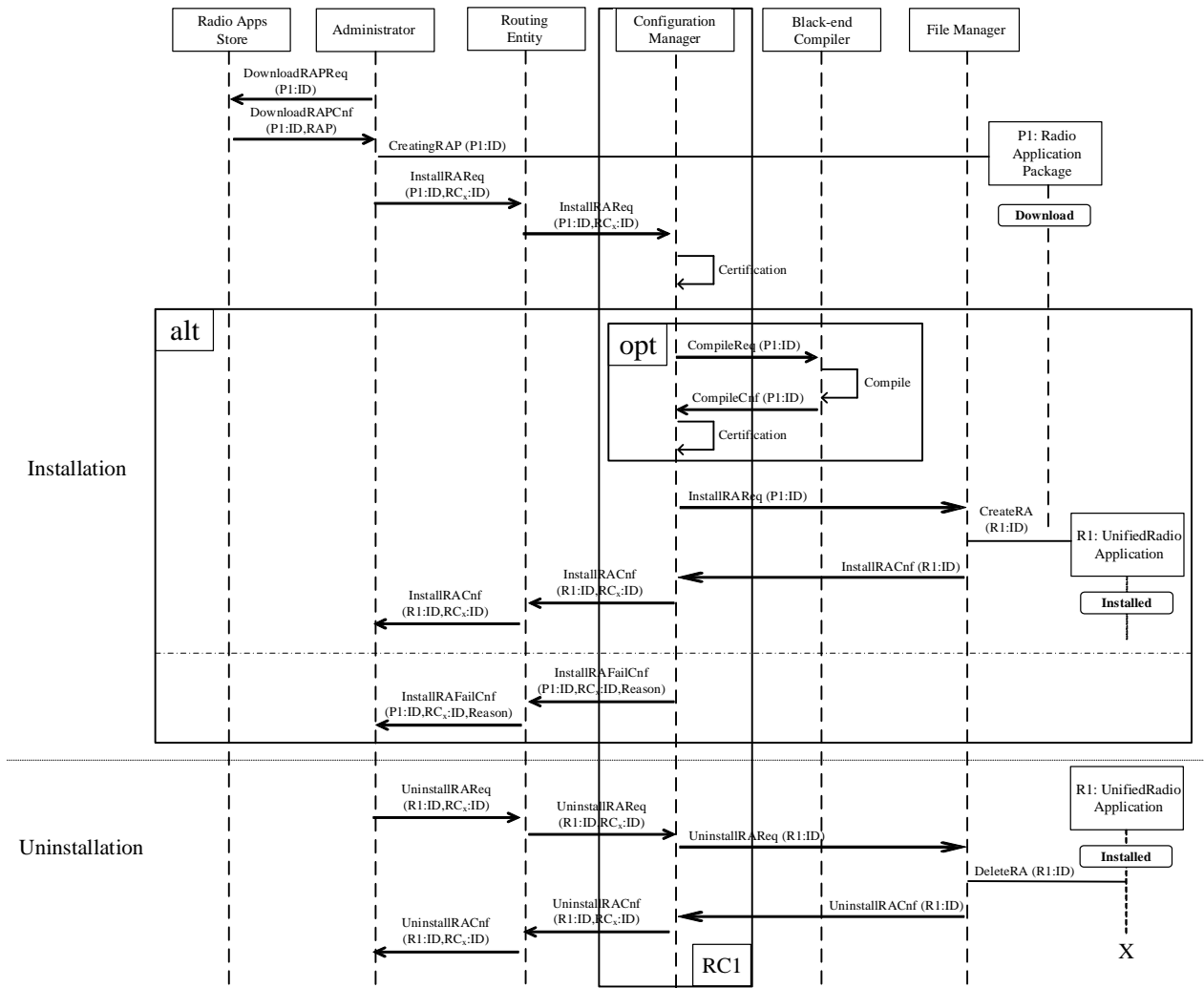
Figure 6.1-1: URA (un)installation
